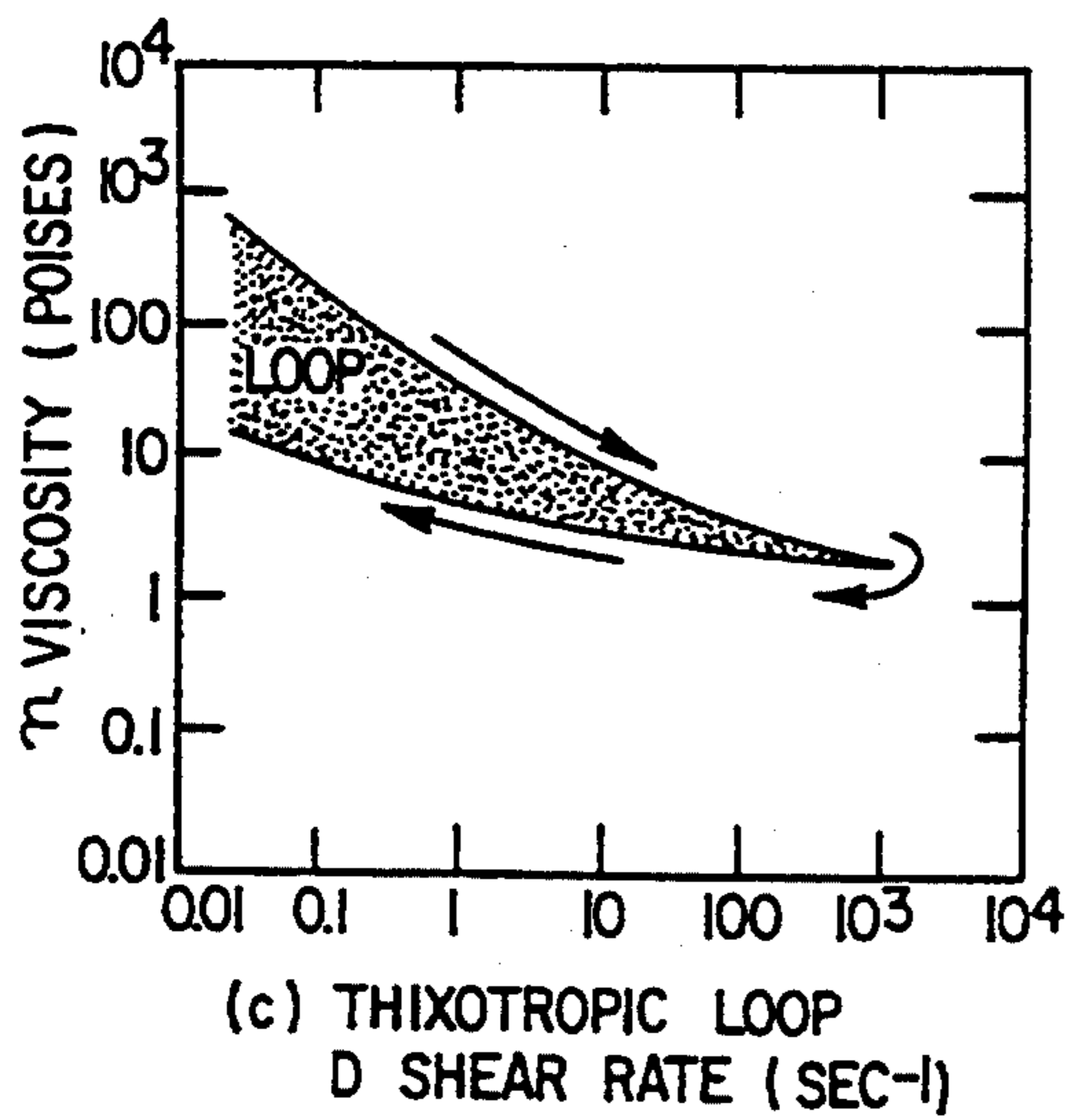
FIG. IIc PRIOR ART
