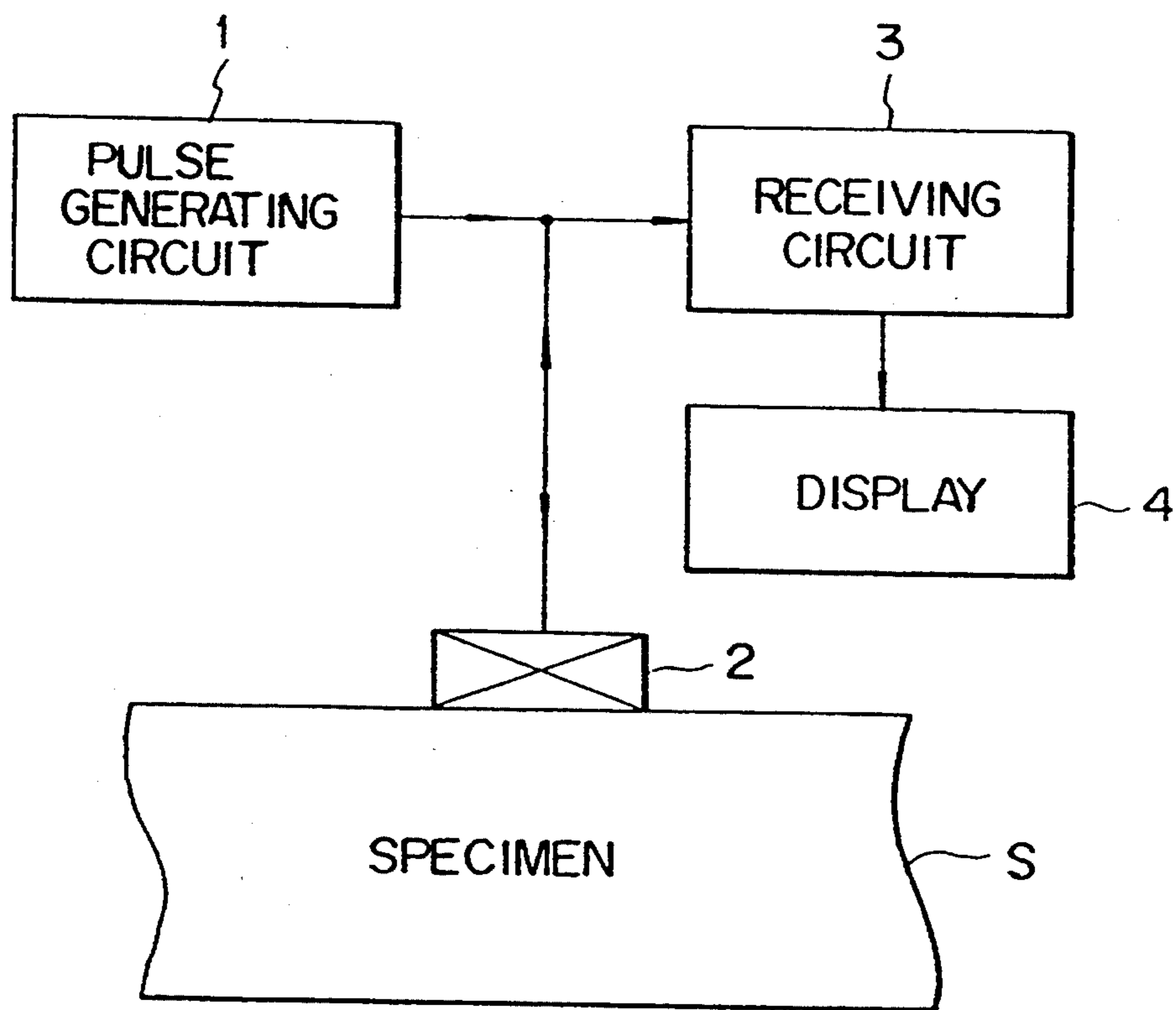
Fig. 1 (PRIOR ART)
