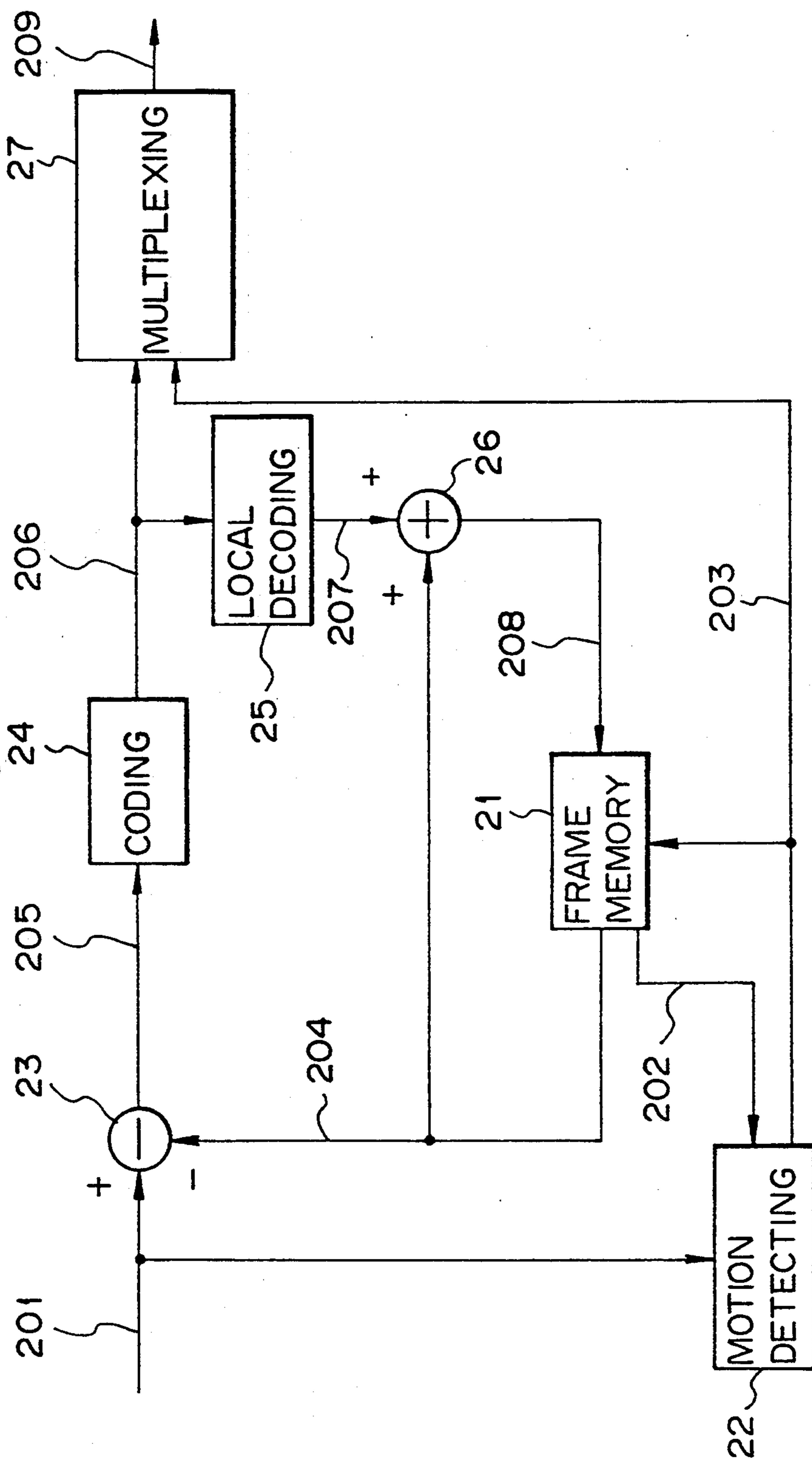
Fig. 4 (PRIOR ART)
