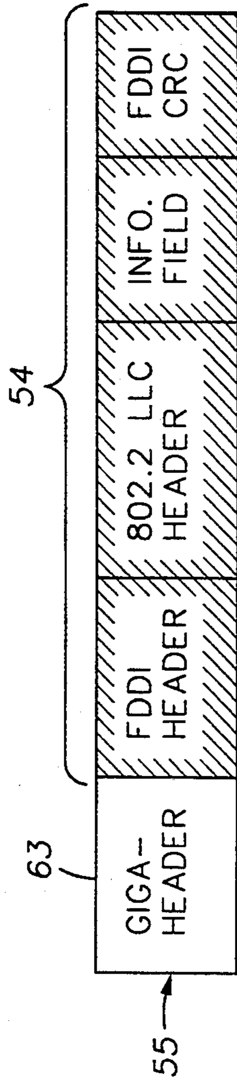
FDDI FRAME FORMAT
