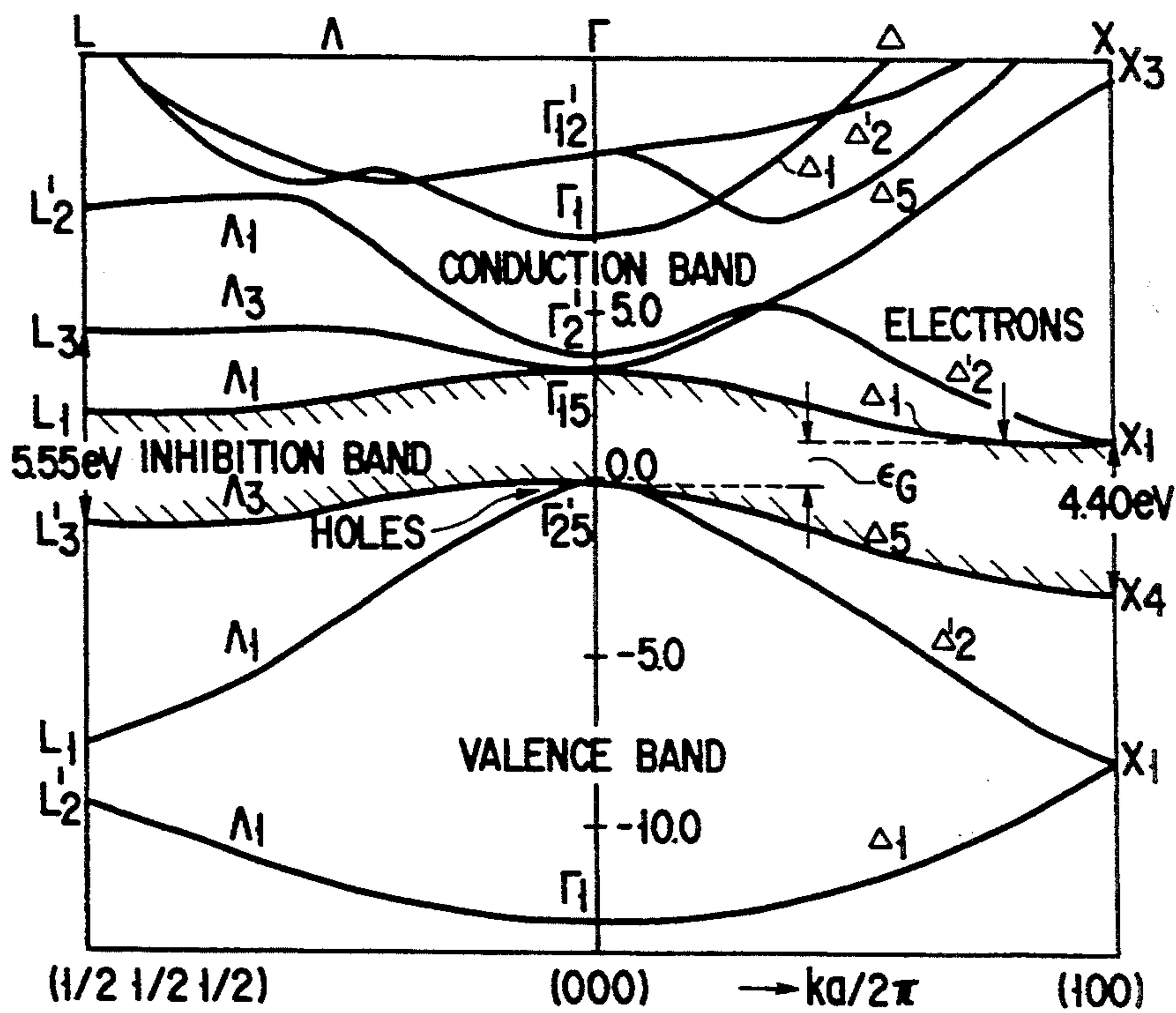
ENERGY-BAND CONFIGURATION OF SILICON
