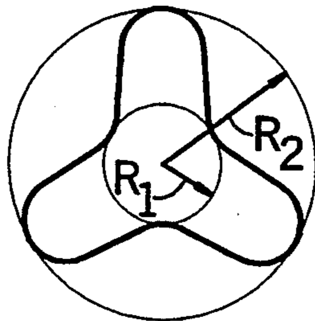
TRILOBAL, MR=1.7 and 2.4
