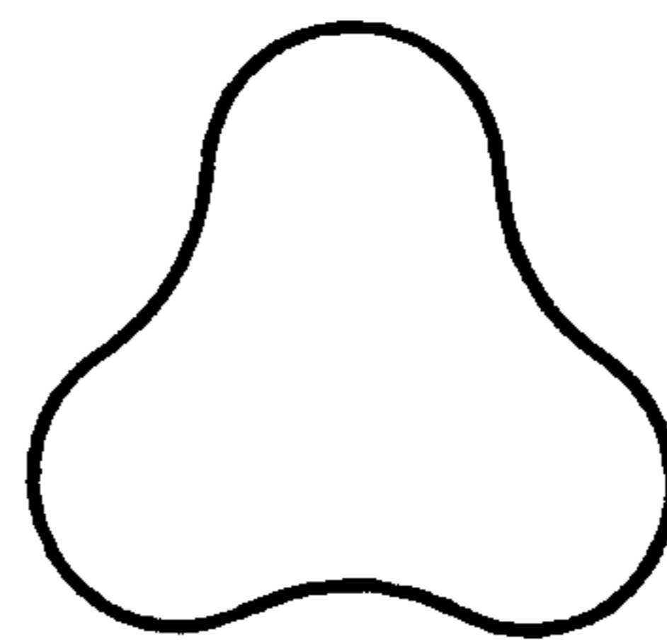
TRILOBAL, MR=1.7 and 2.4
