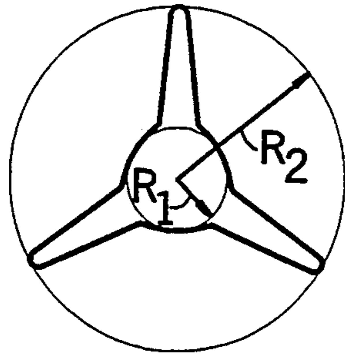
TRIANGULAR TRILOBAL, MR=2.4 AND 3.4
