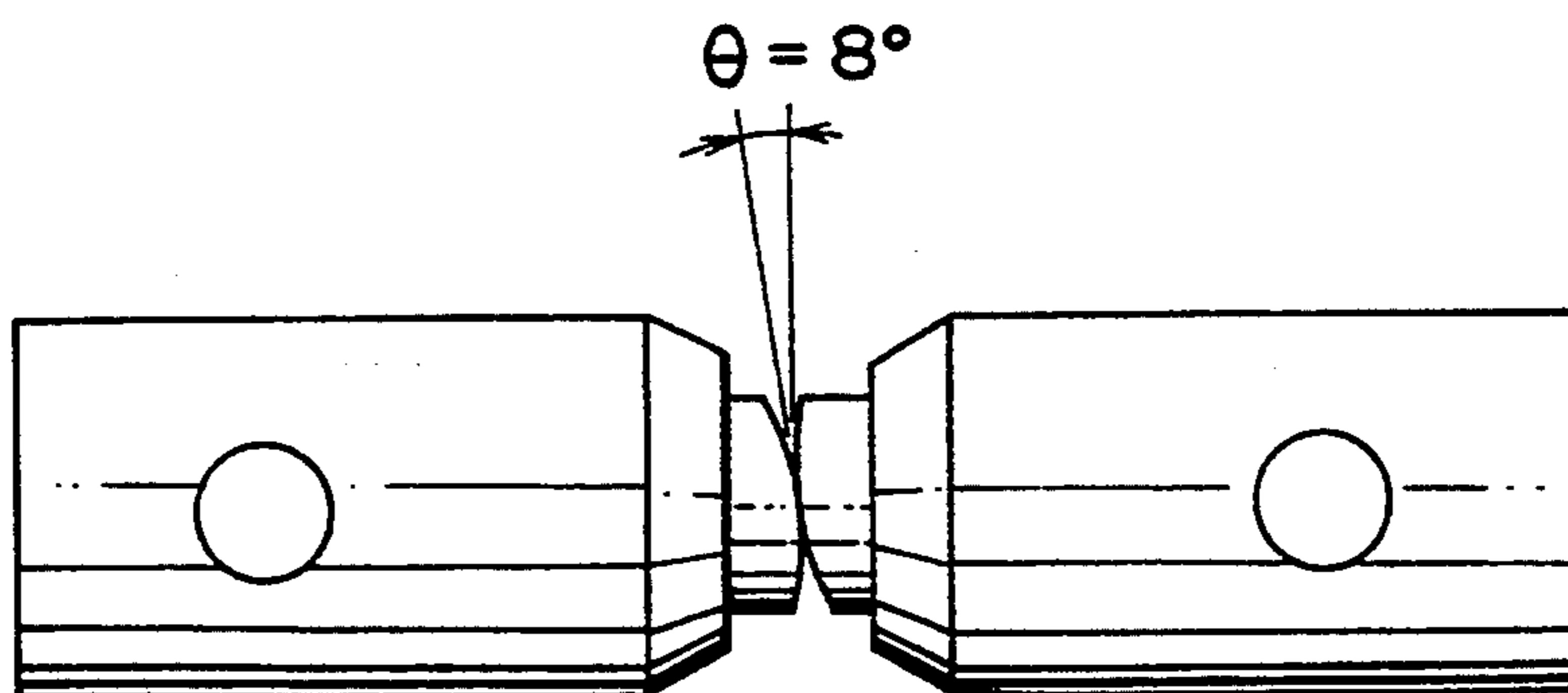
FIG. 7 PRIOR ART
