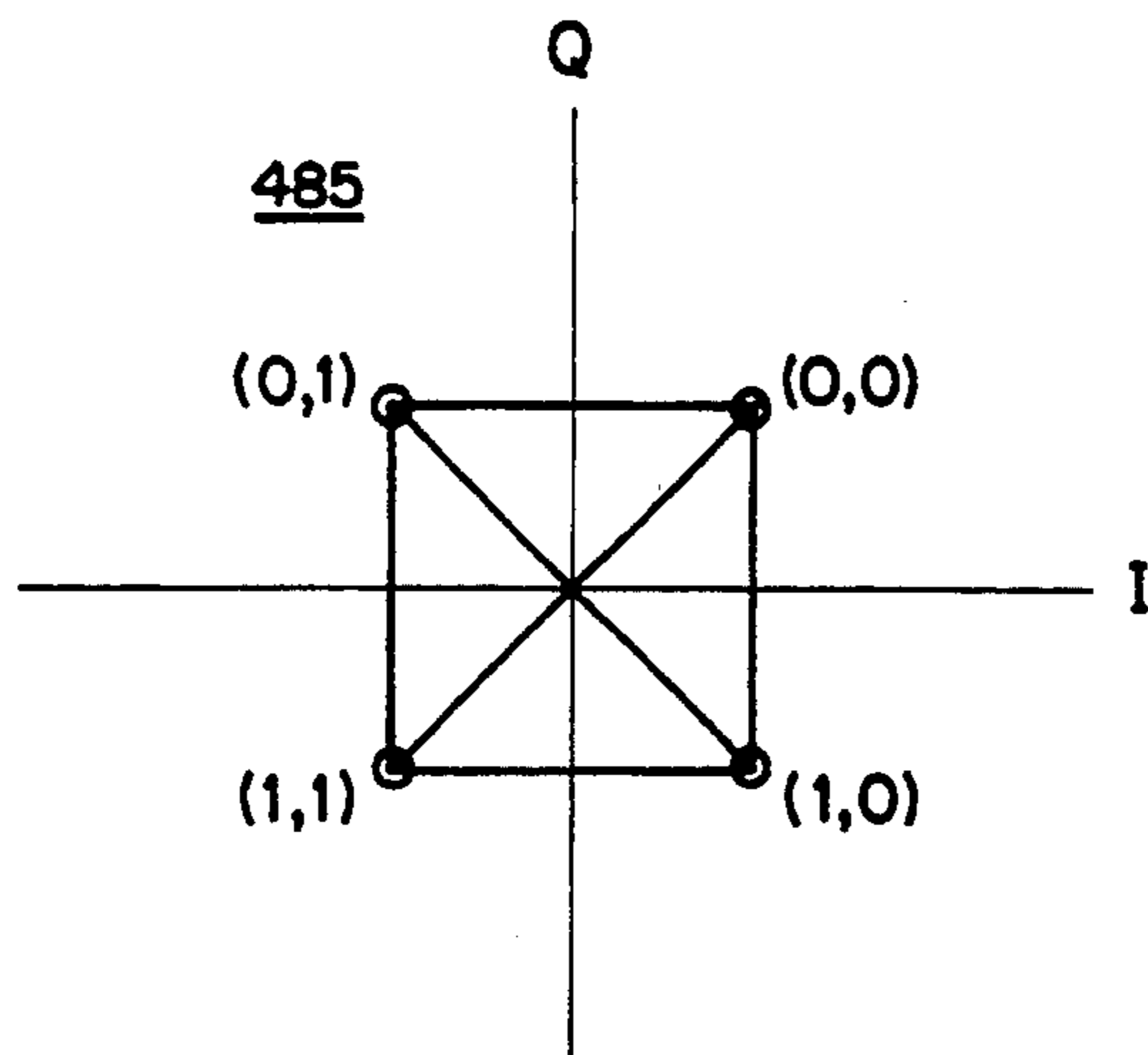
QPSK - CONSTELLATION
