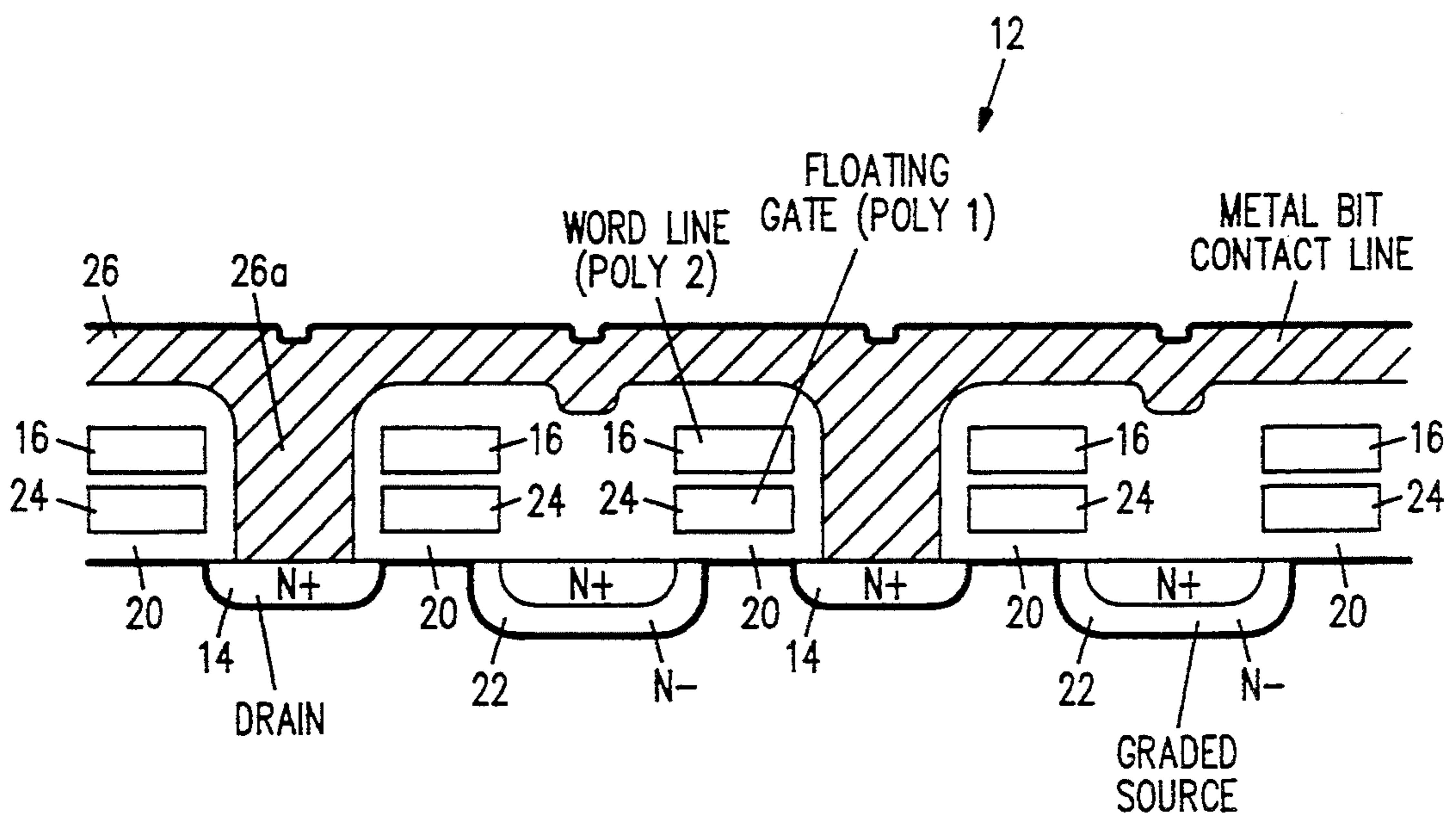
PRIOR ART
