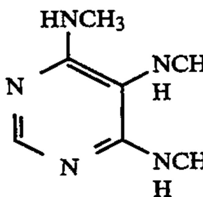
4,6-Diamino-5-(N,N-dimethylamino)pyrimidine PY-4
