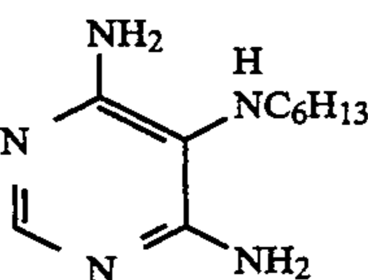
4,6-Diamino-5-(N-hexylamino)pyrimidine PY-5
