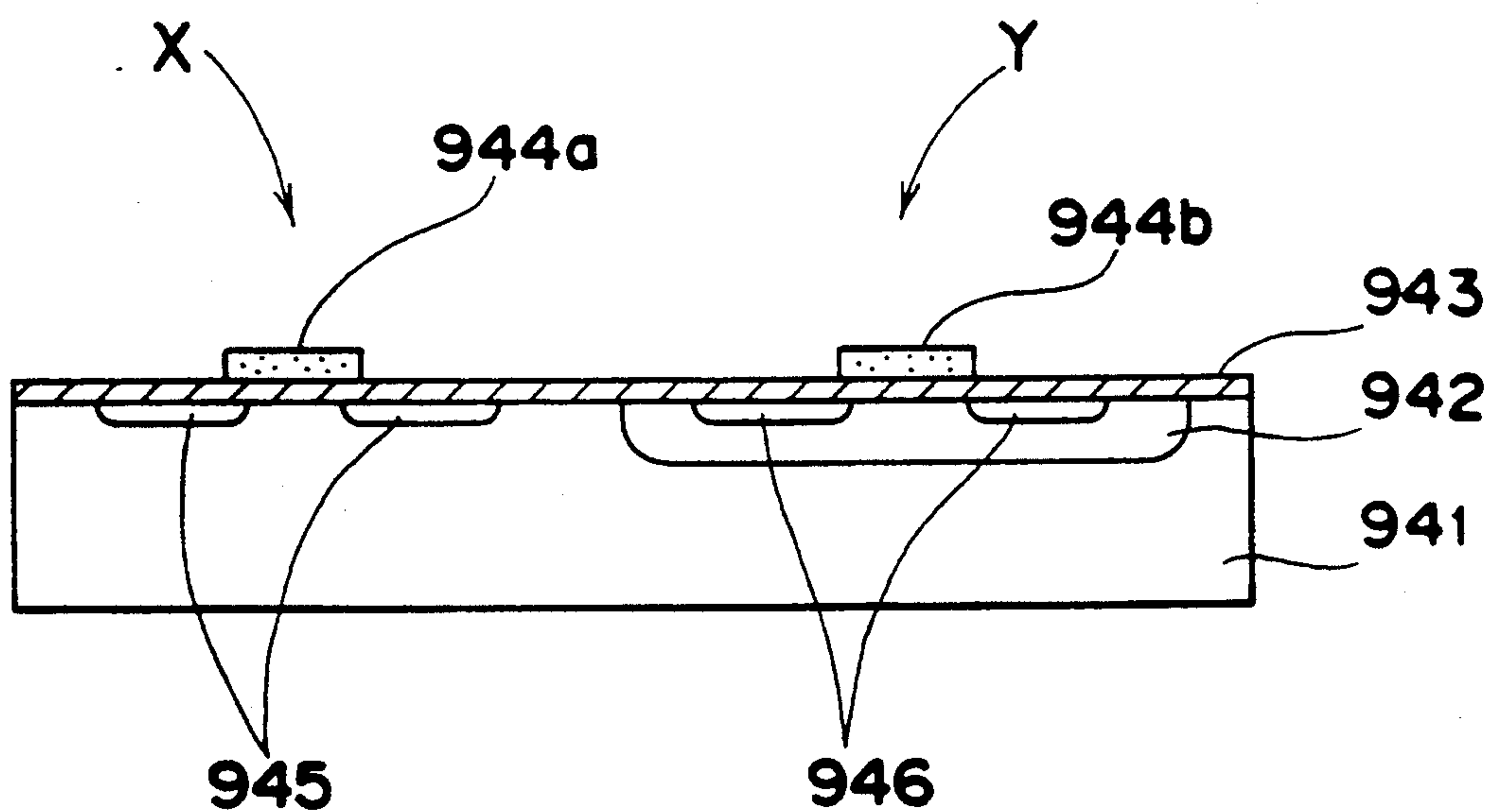
Fig. 3 PRIOR ART
