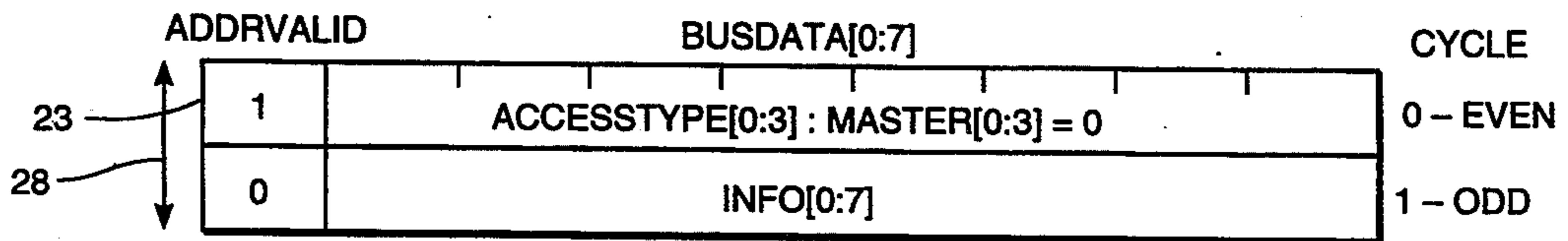
FIG 5 REJECT (NACK) CONTROL PACKET
