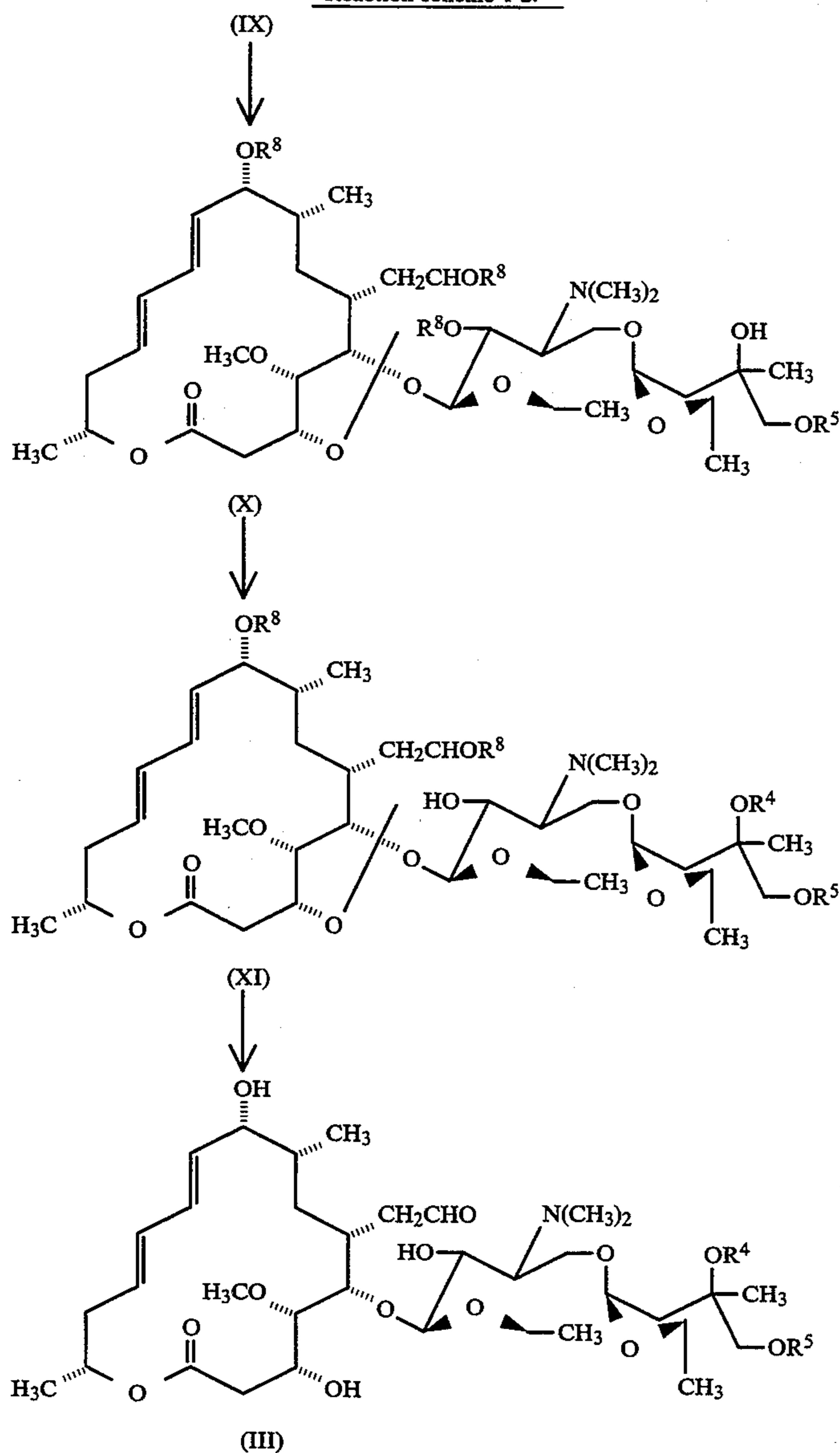
Reaction scheme 1-2:
