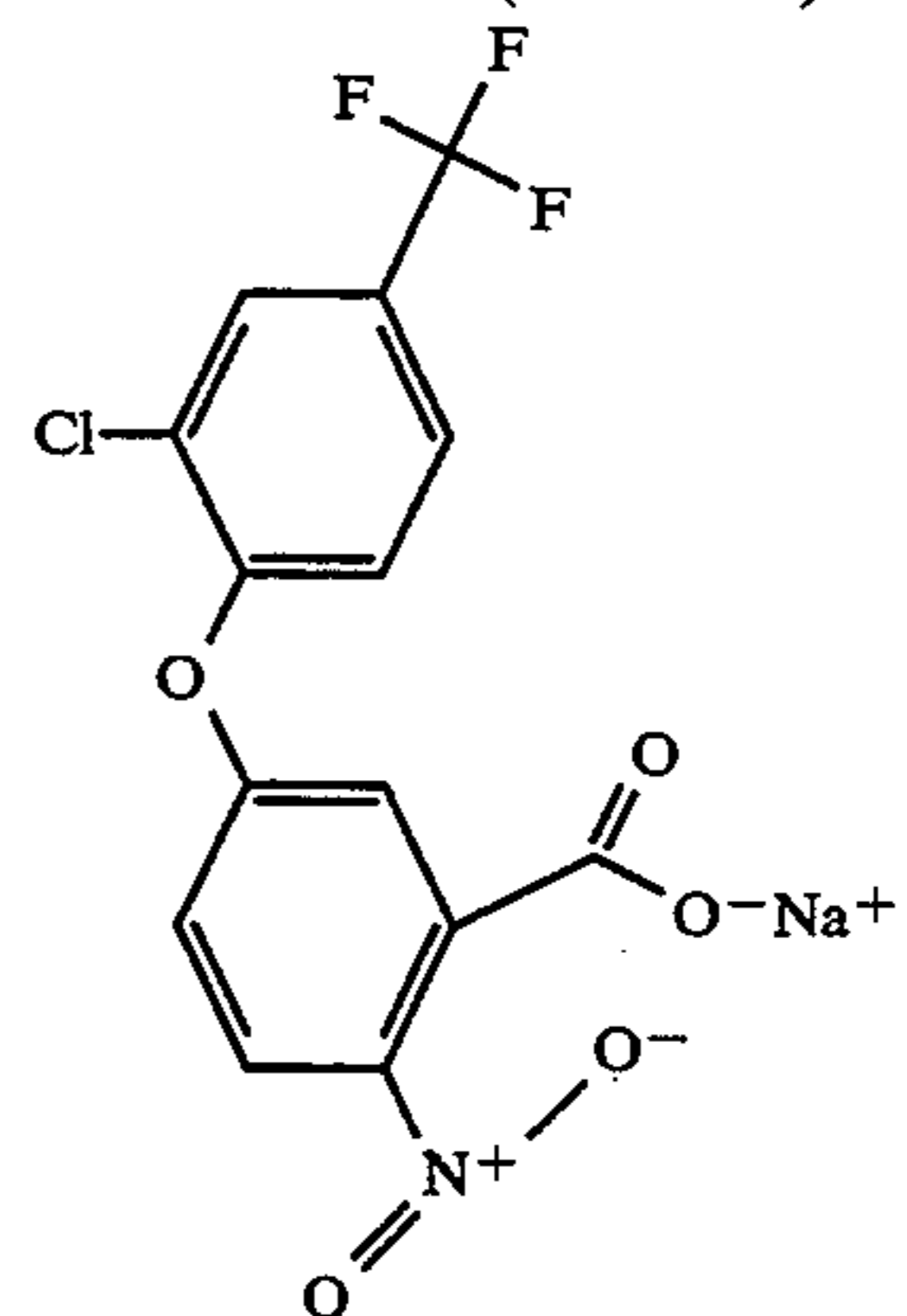
sodium 5-(2-chloro-4-(trifluoro-methyl)phenoxy)-2-nitrobenzoate (acifluorfen)
