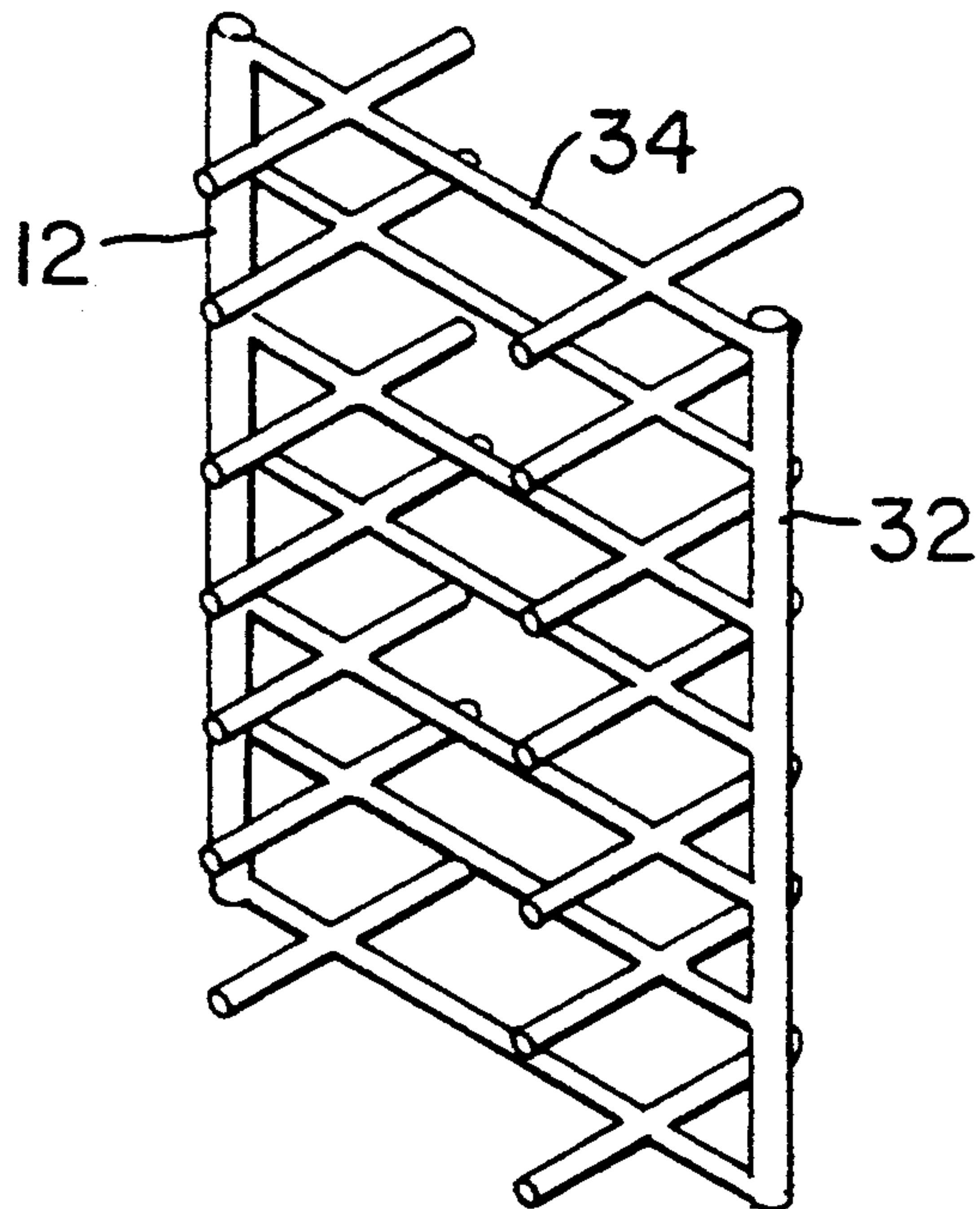
FIG. 6 PRIOR ART
