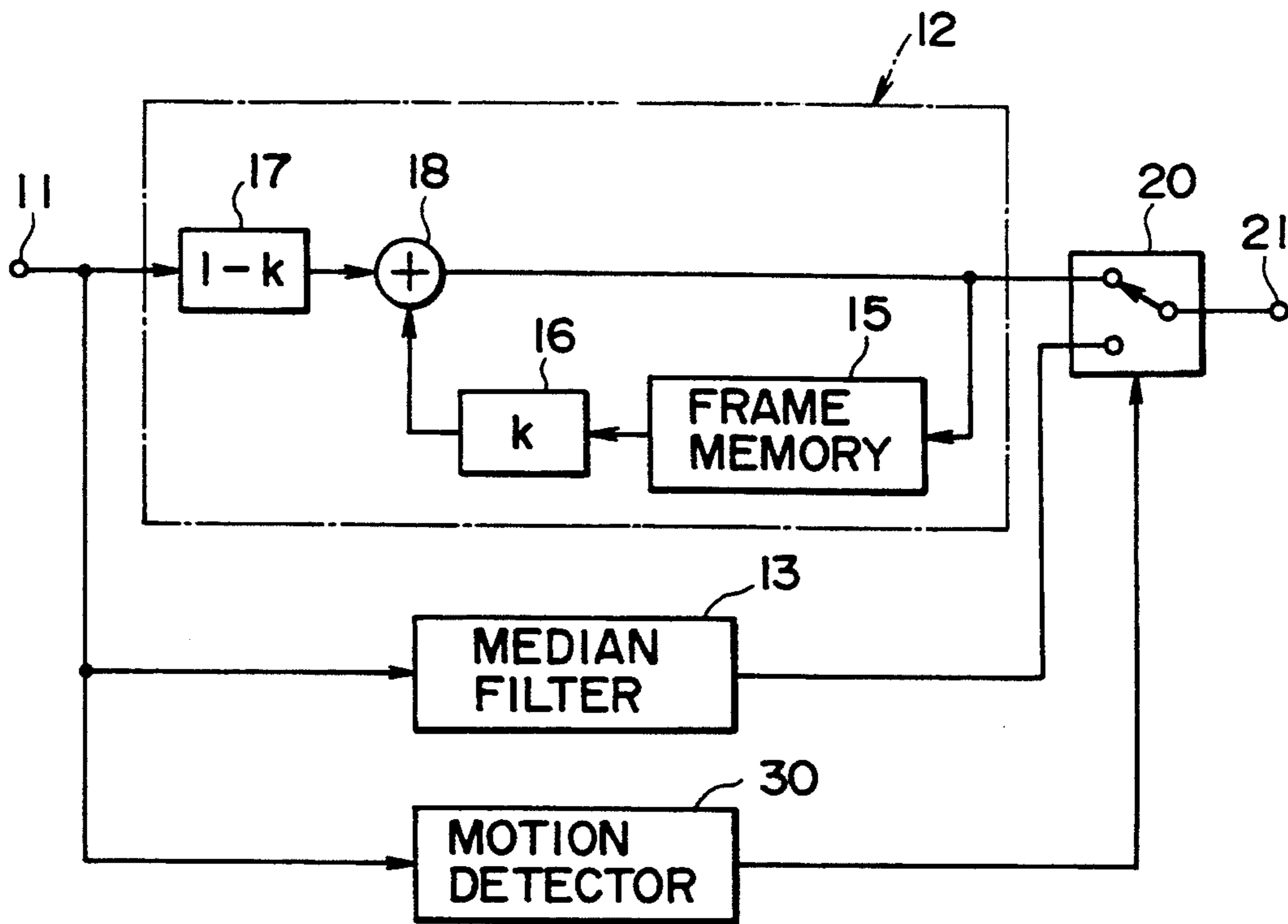
NOISE ELIMINATING CIRCUIT 10
