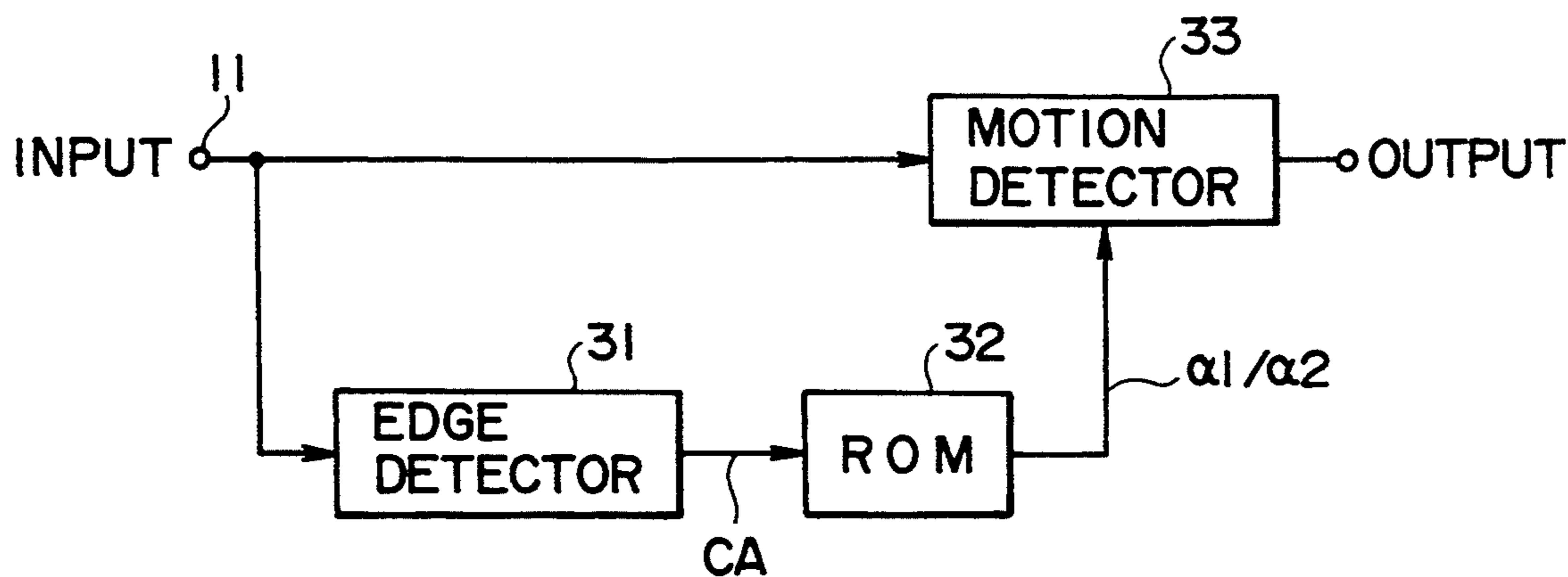
MOTION DETECTOR 30
