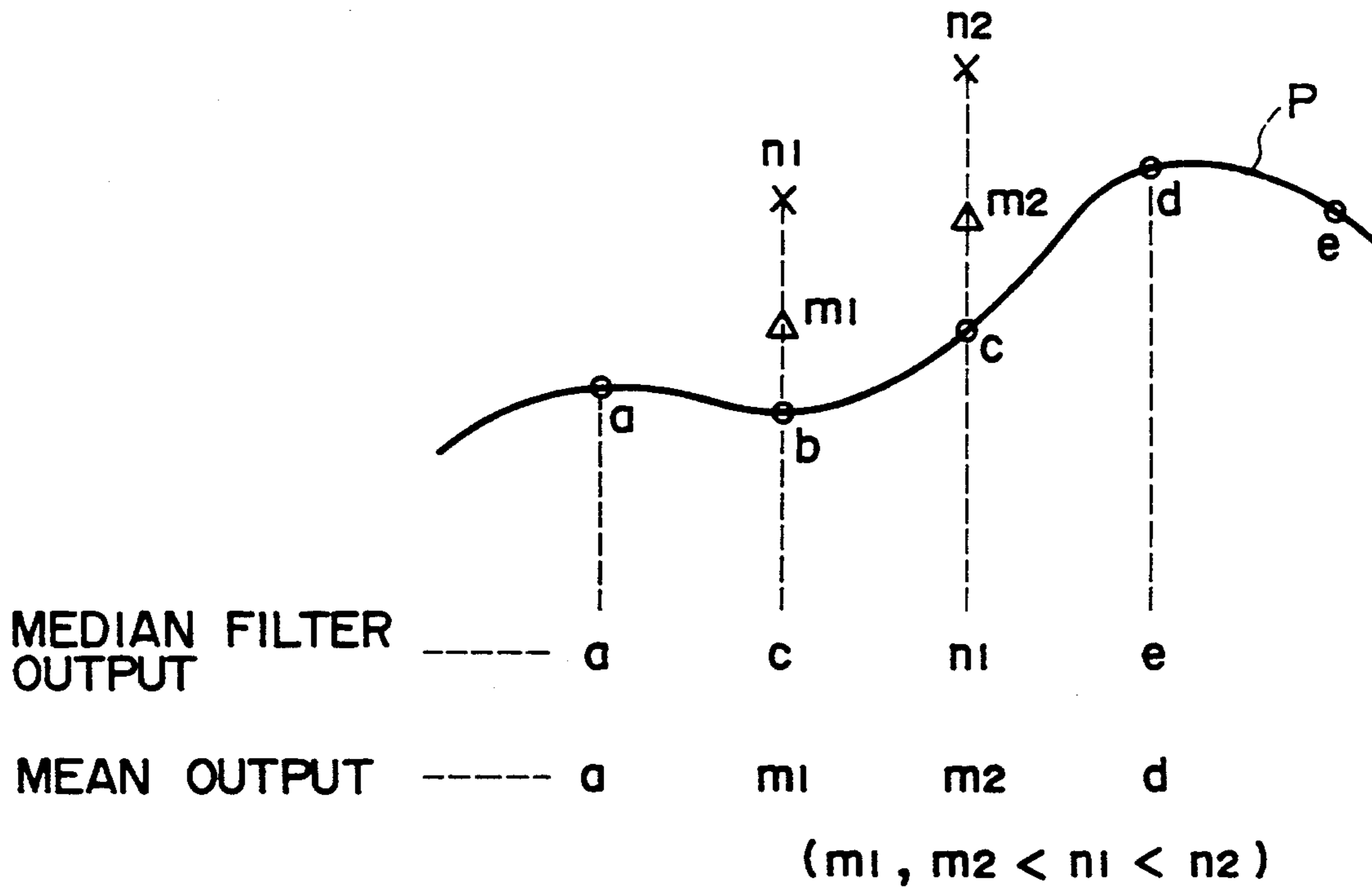
EXAMPLE OF MEDIAN FILTER PROCESSING
