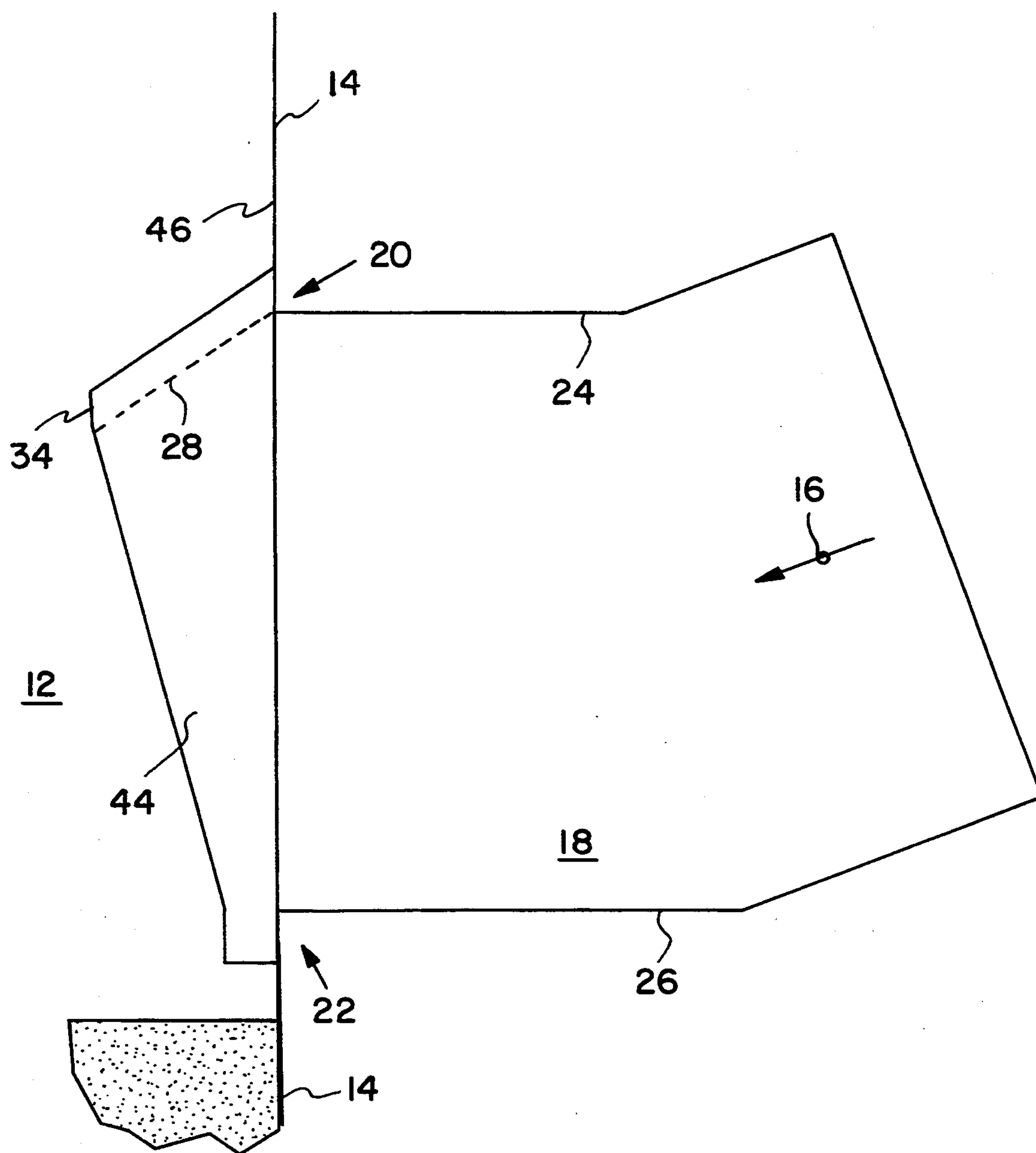
FIG. 5 PRIOR ART
