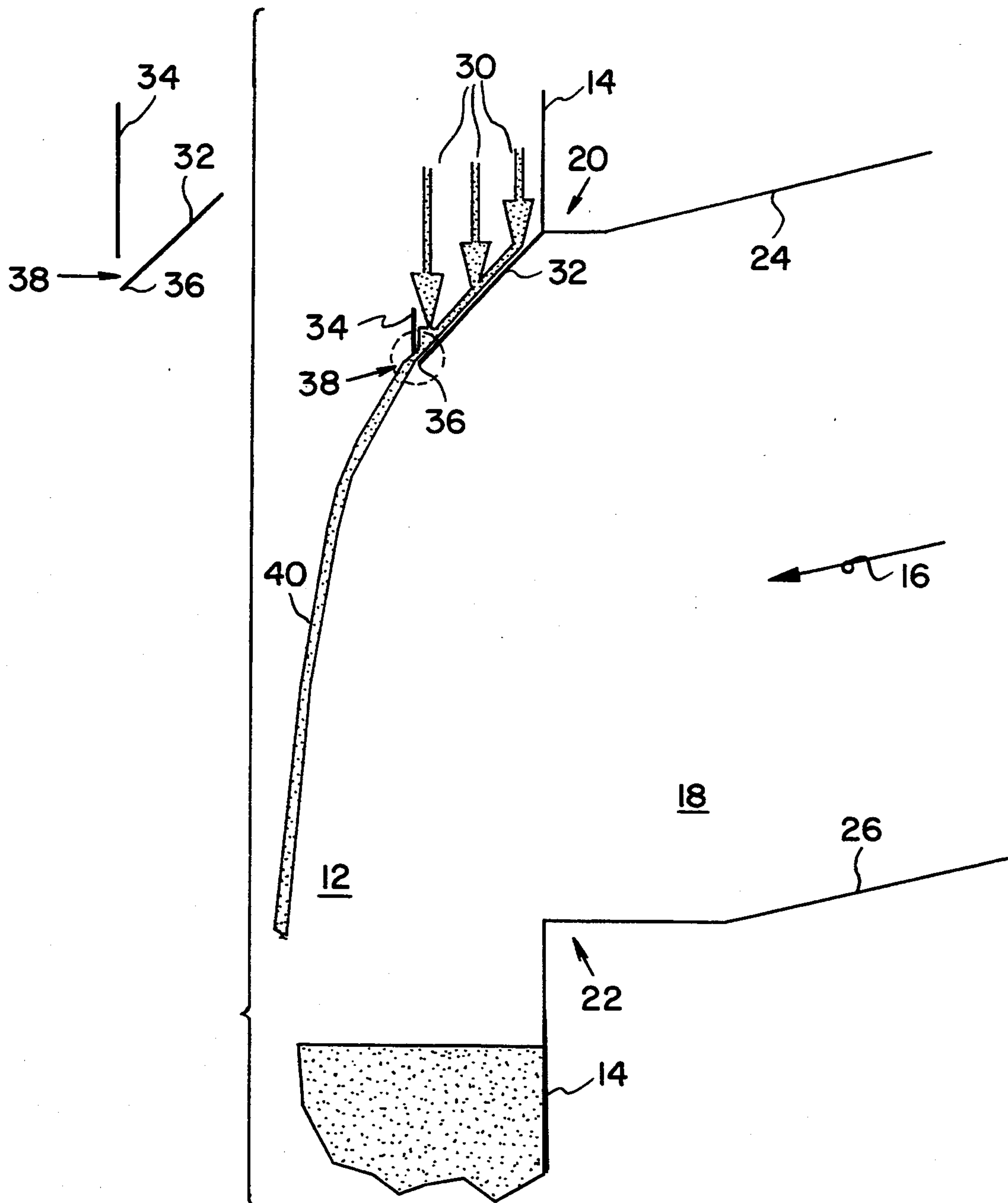
FIG. 2 PRIOR ART
