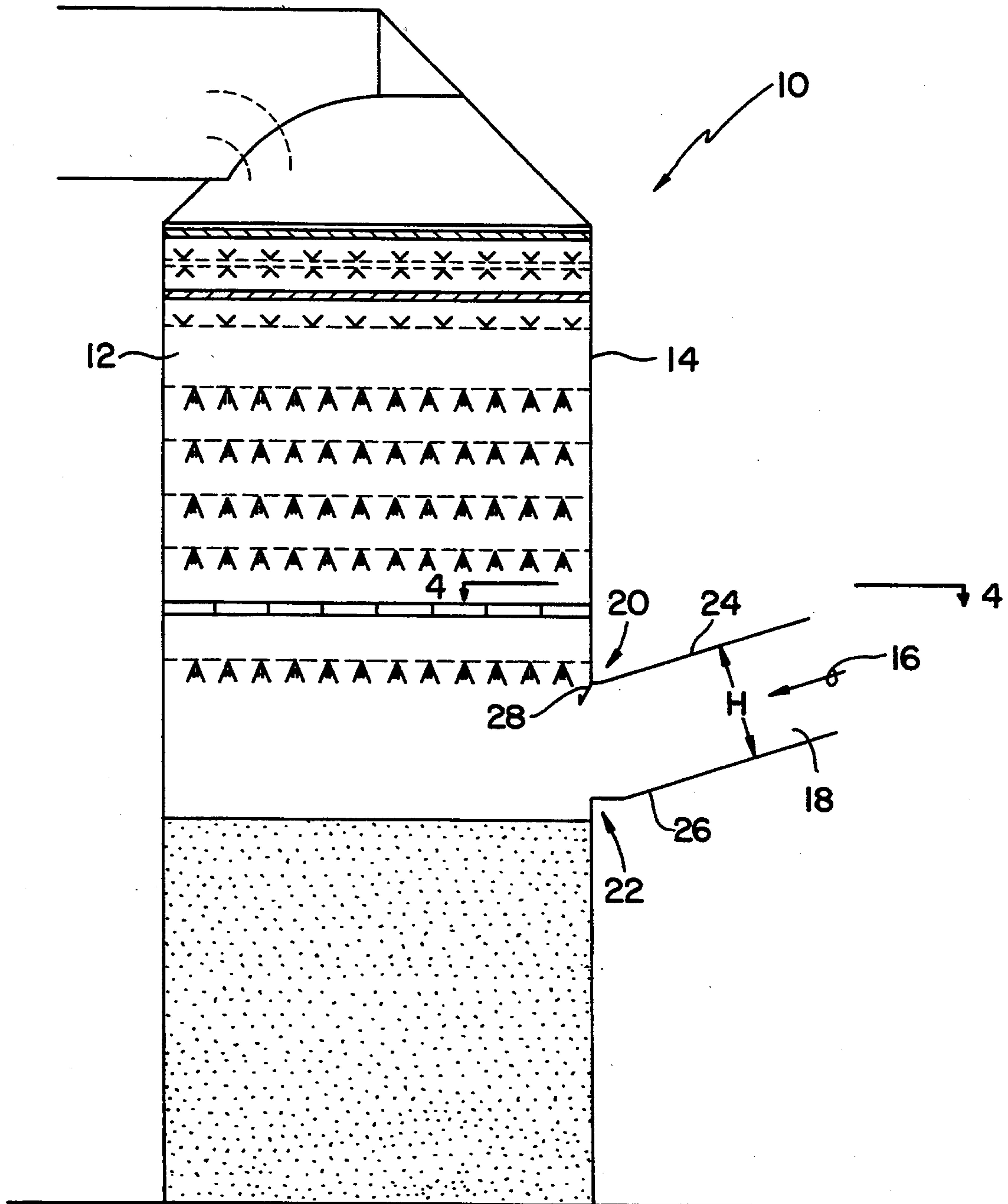
FIG. 1 PRIOR ART
