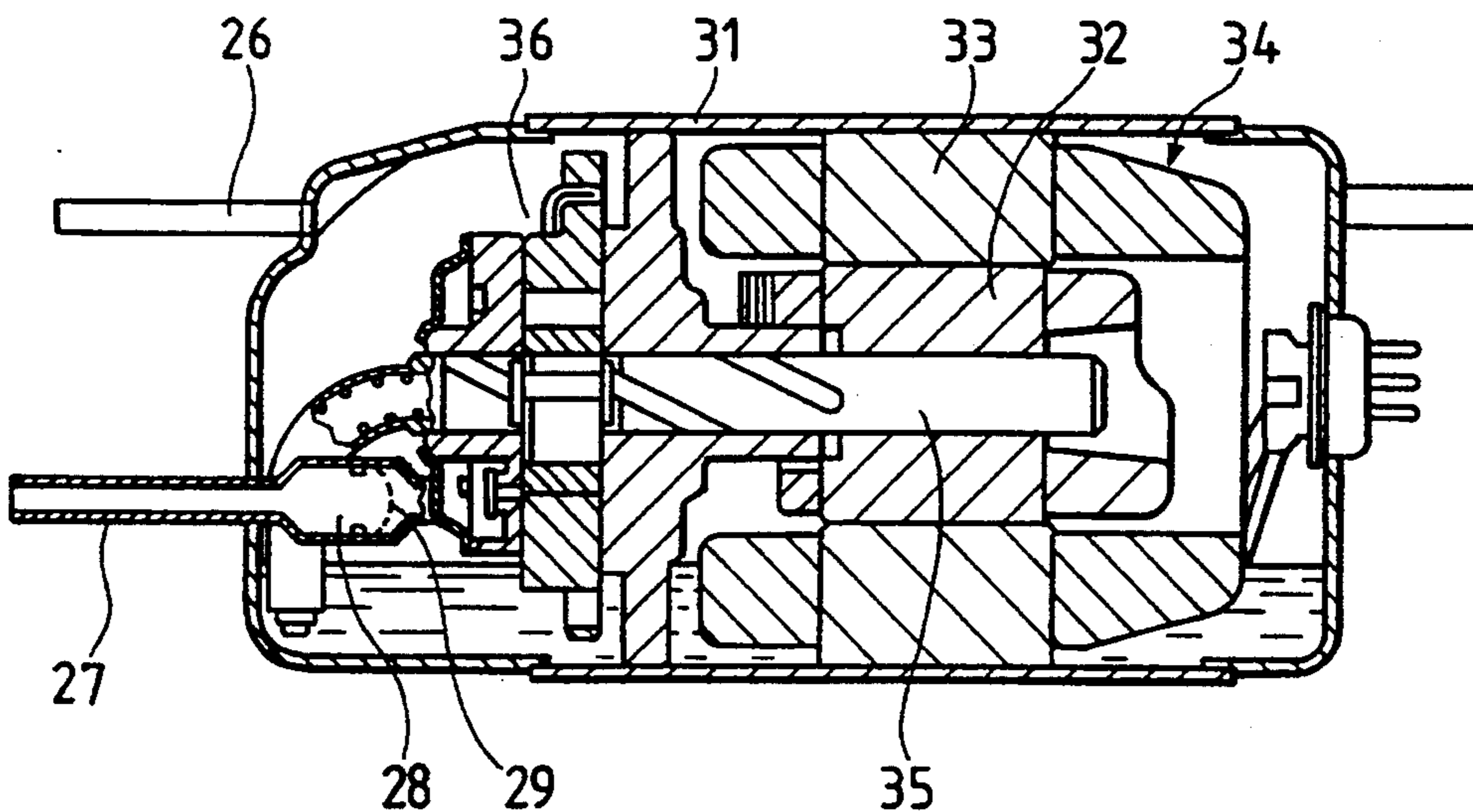
FIG. 20 PRIOR ART
