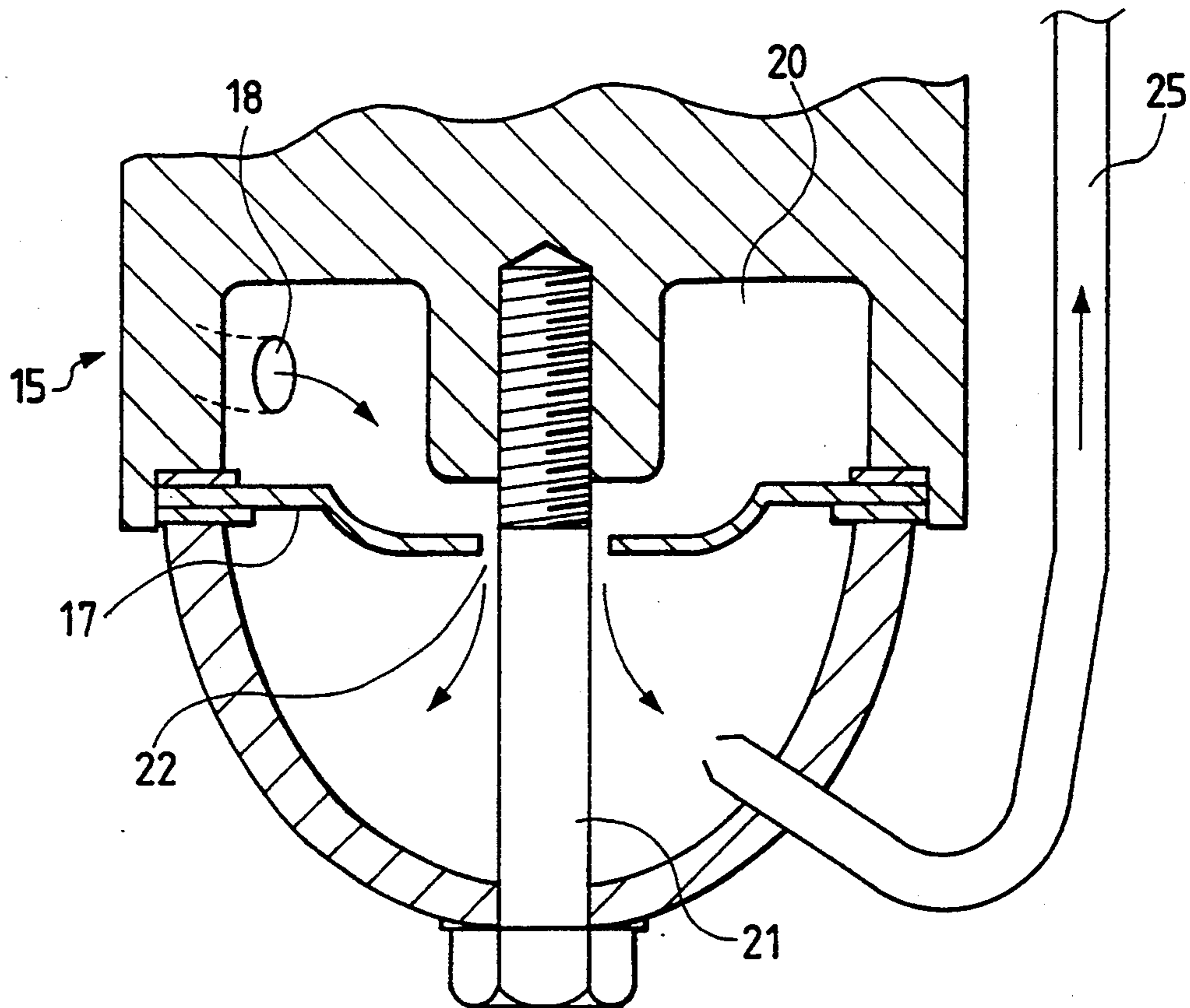
FIG. 19 PRIOR ART
