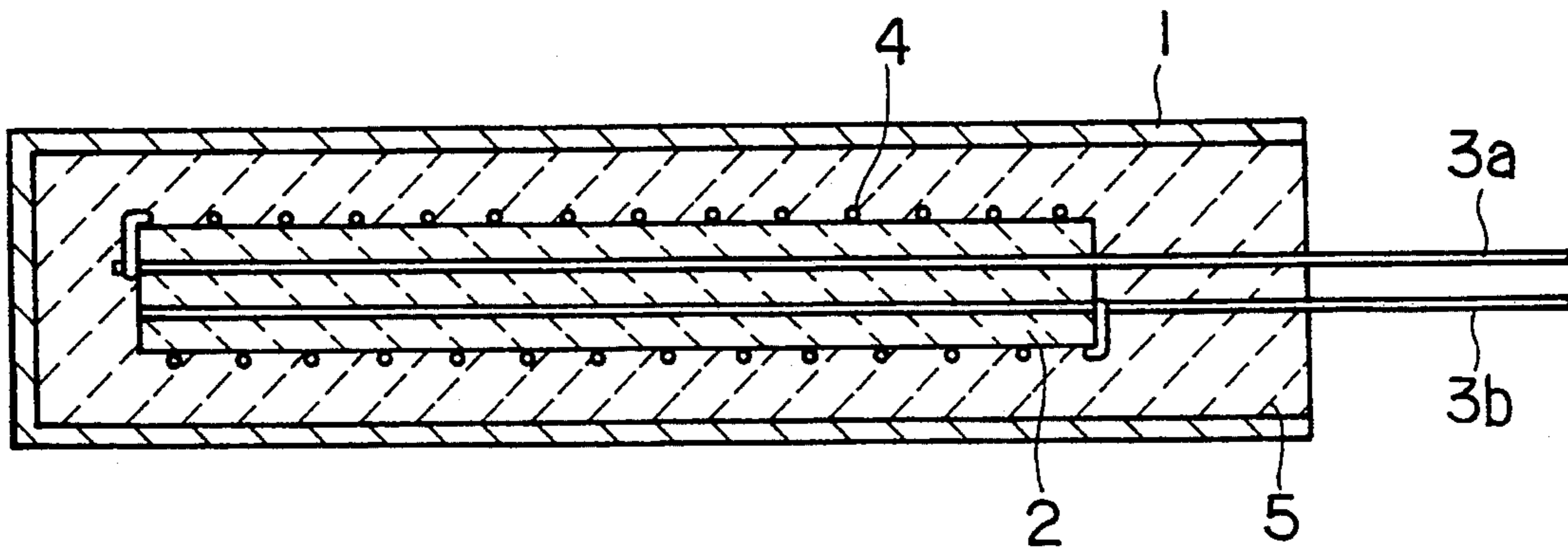
FIG. 1 PRIOR ART
