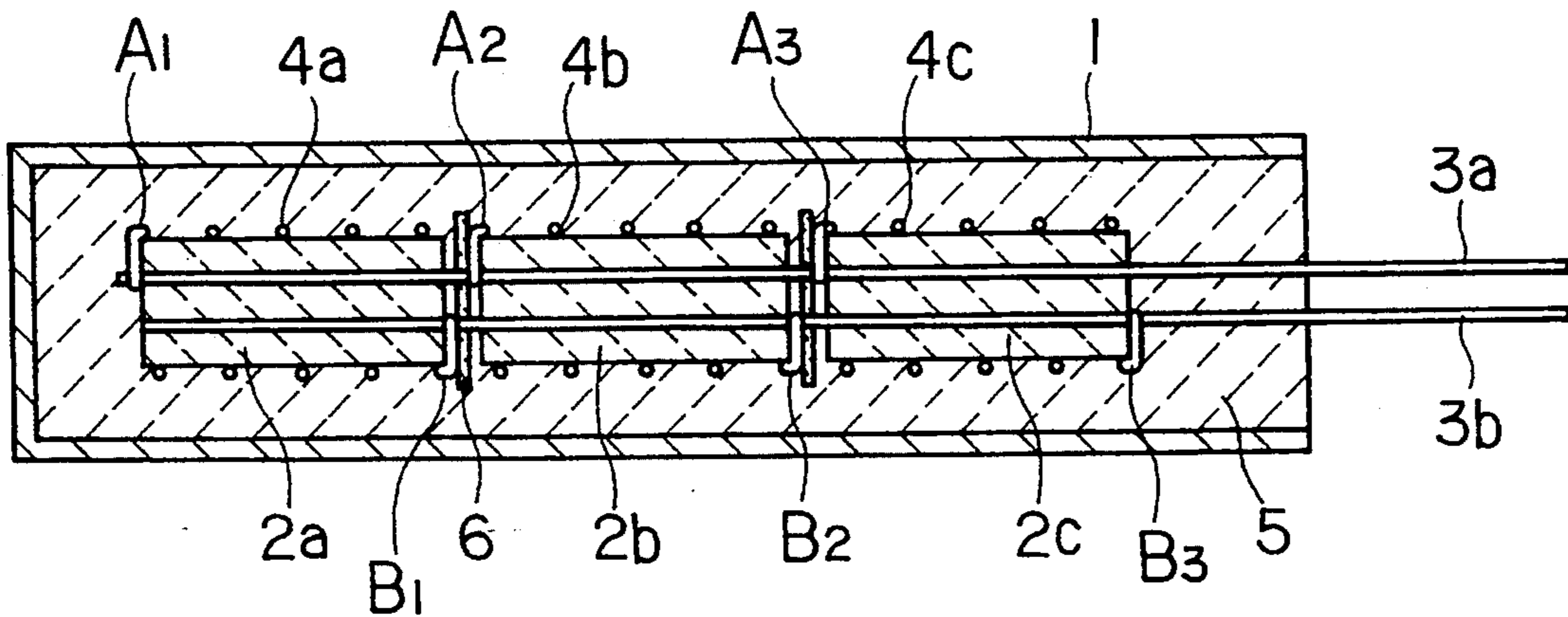
FIG. 2 PRIOR ART
