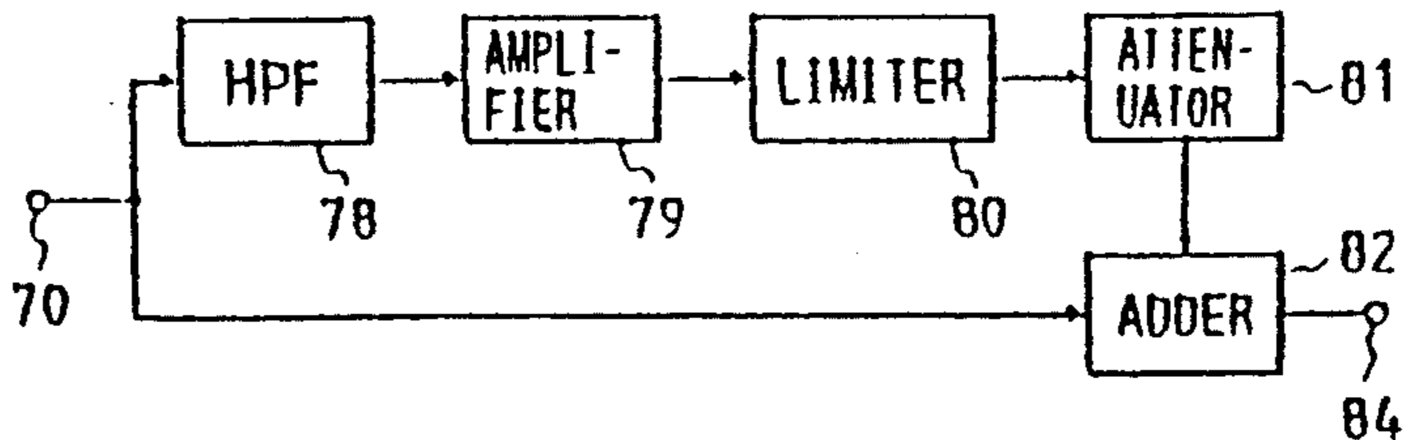
FIG. 13 PRIOR ART
