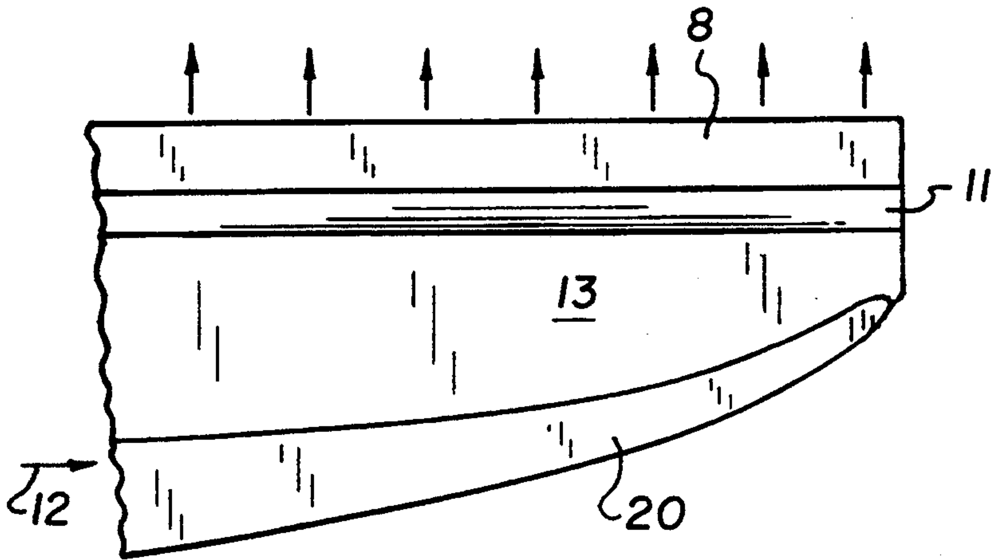
FIG. 3 (PRIOR ART)
