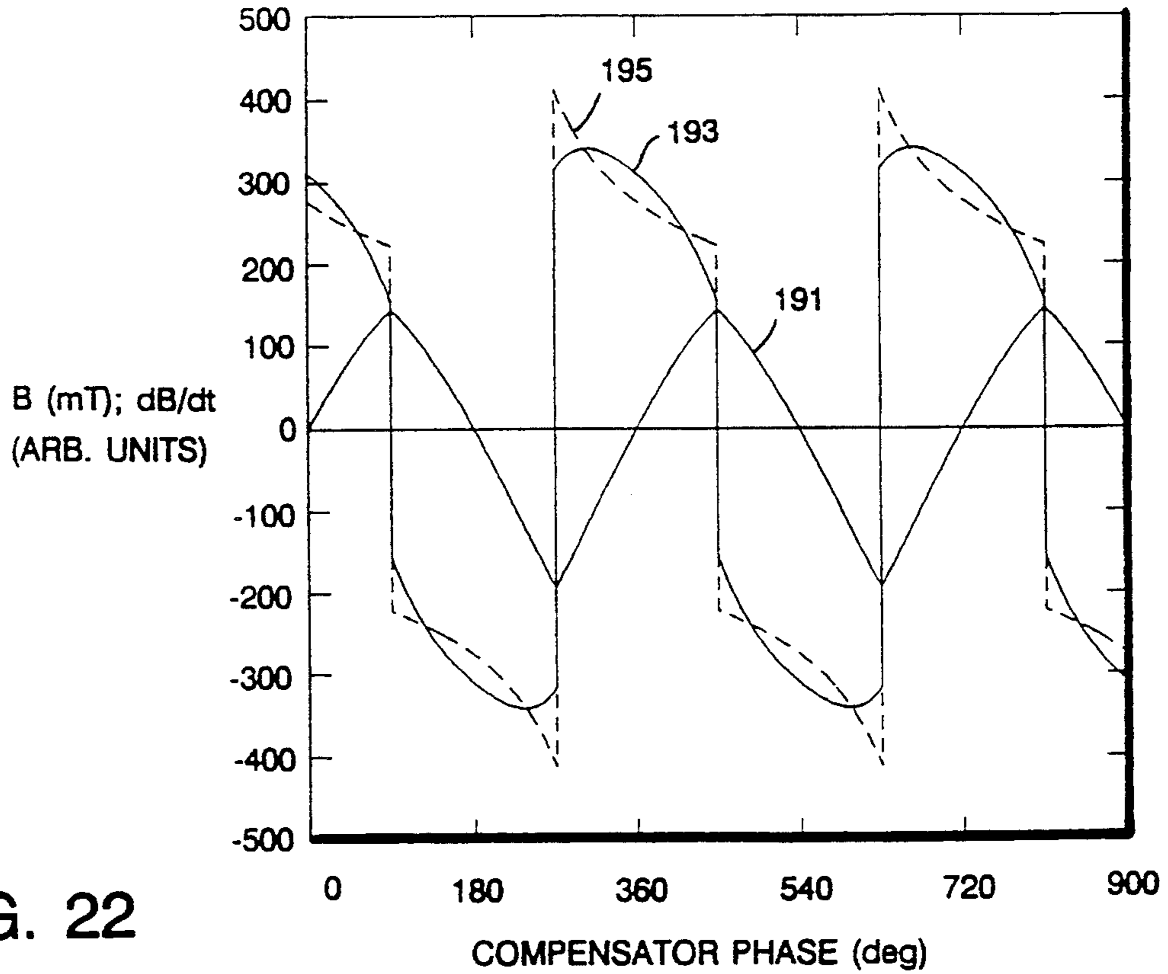
SCANNER FIELD & SCAN VELOCITY (---) vs COMPENSATOR PHASE
