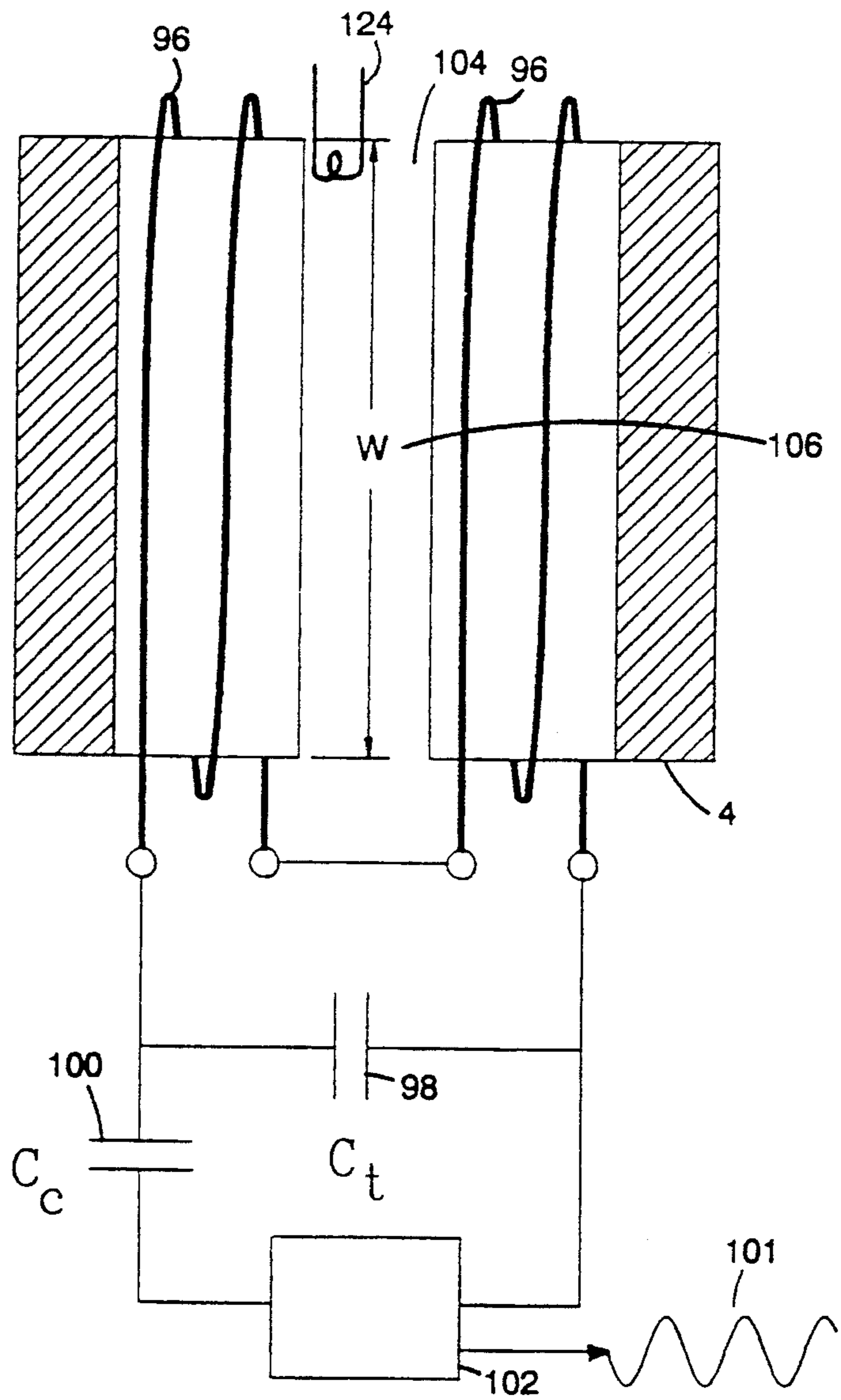
POWER AMPLIFIER
