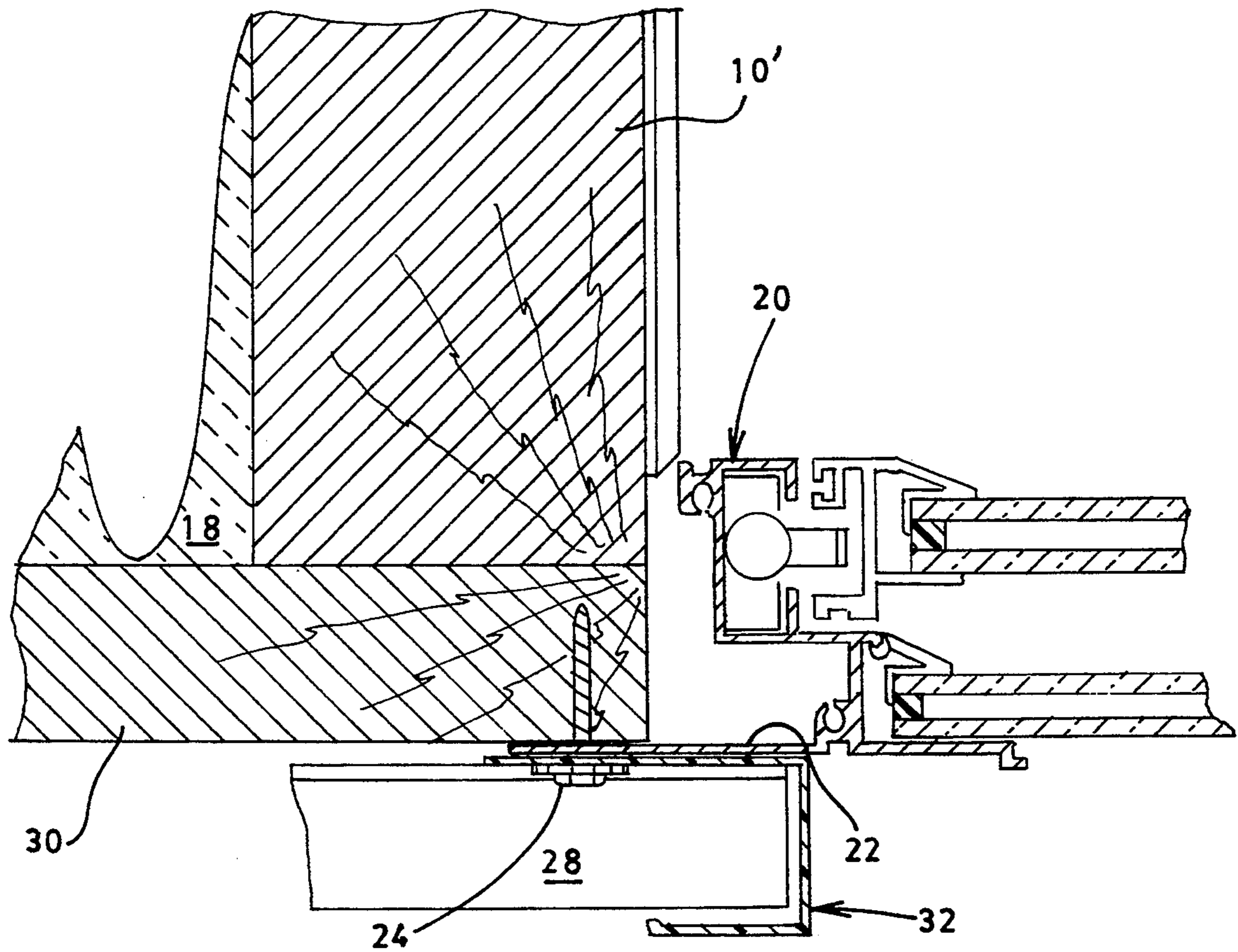
FIG. 1C (PRIOR ART)
