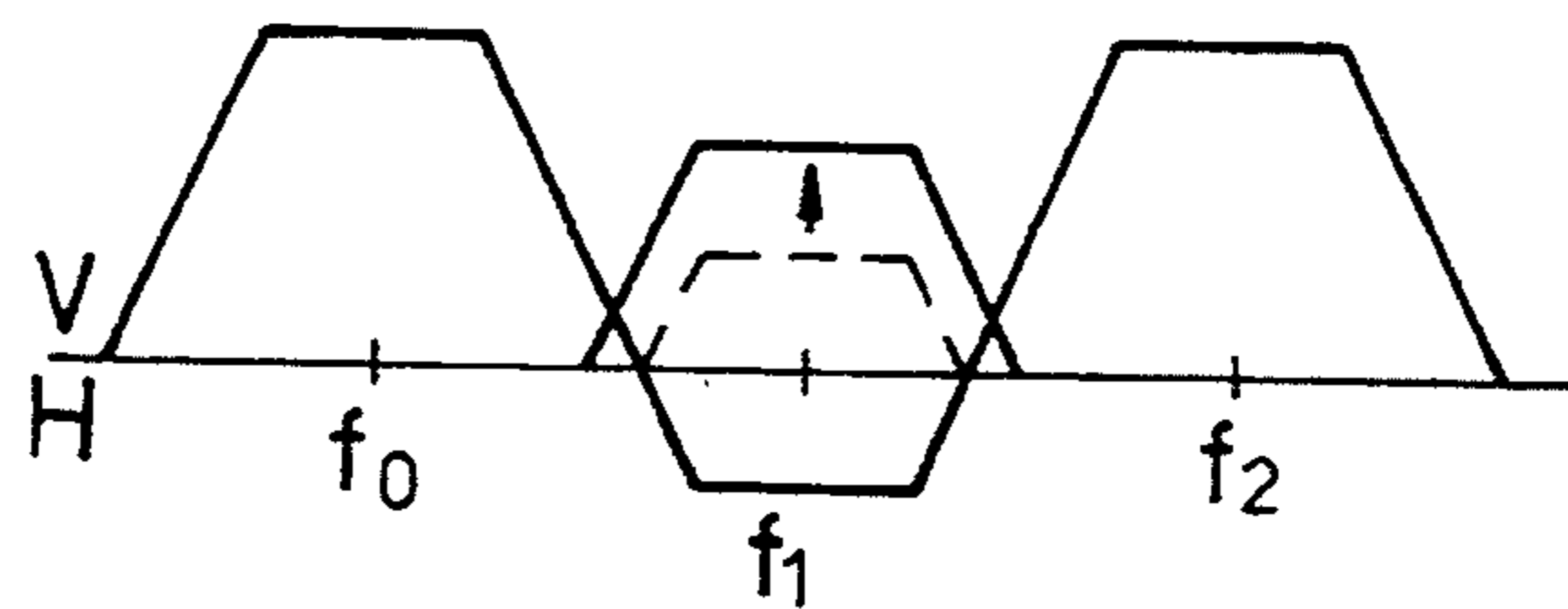
FIG. 2(c) (PRIOR ART)
