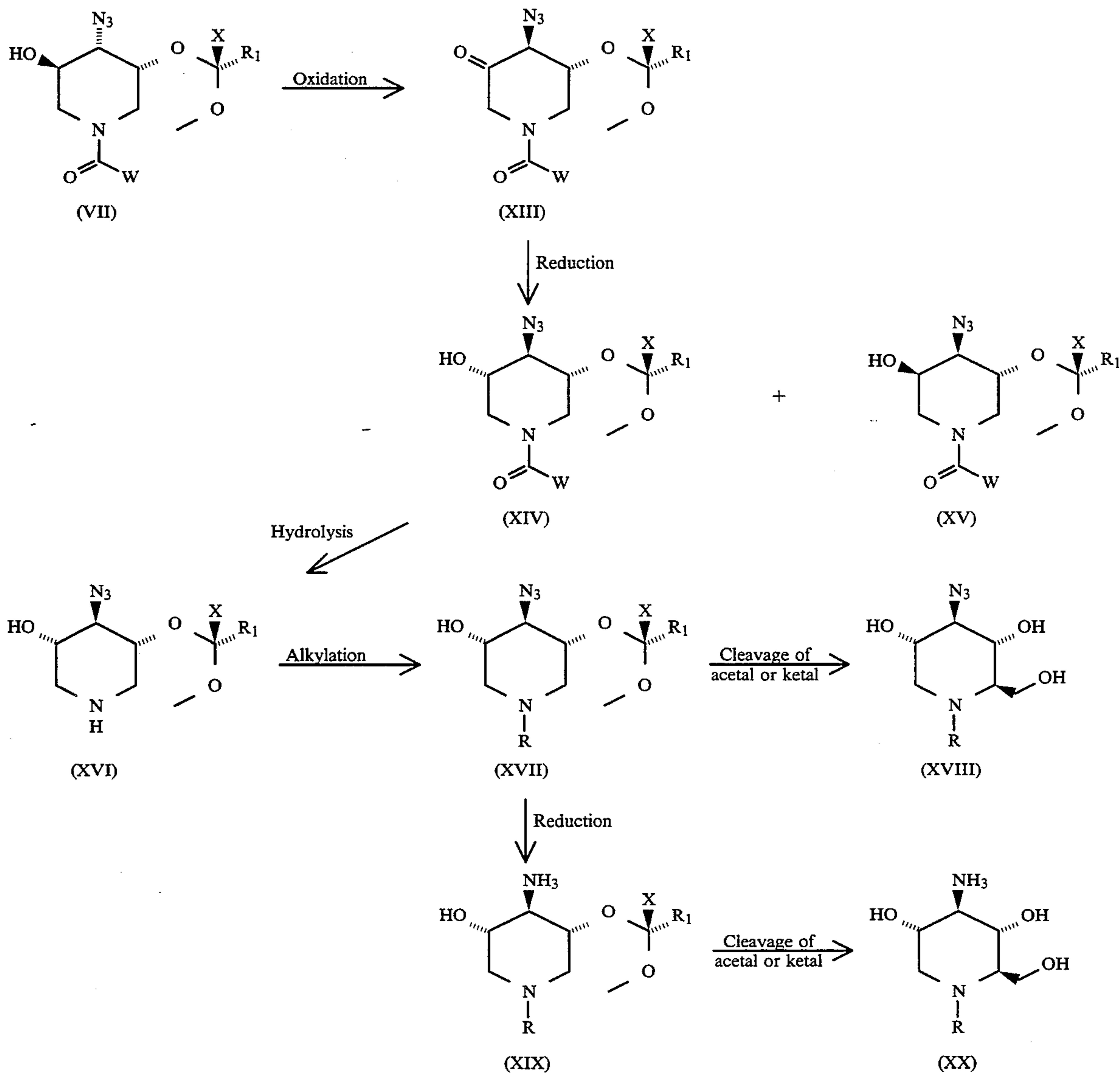
Scheme D: Generic Synthesis of 3-azido- & 3-amino-1,5 iminosugar
