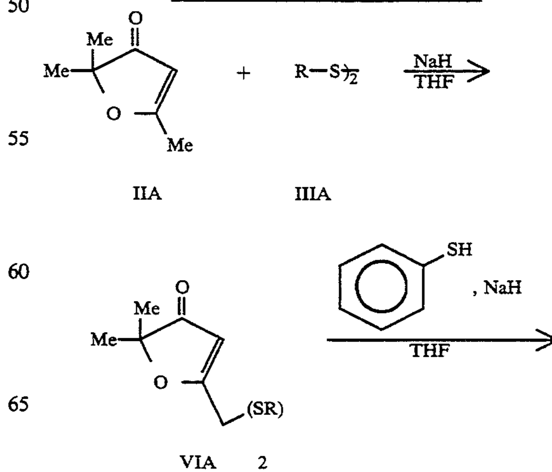
Scheme 8 (for Examples 13 to 14)
