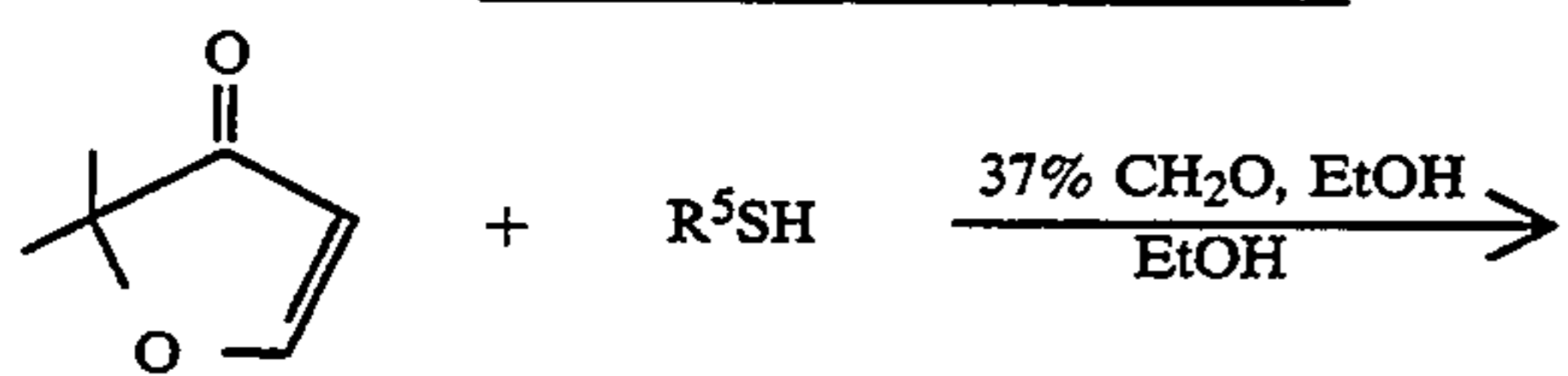
Scheme 1 (for Examples 1 to 5)
