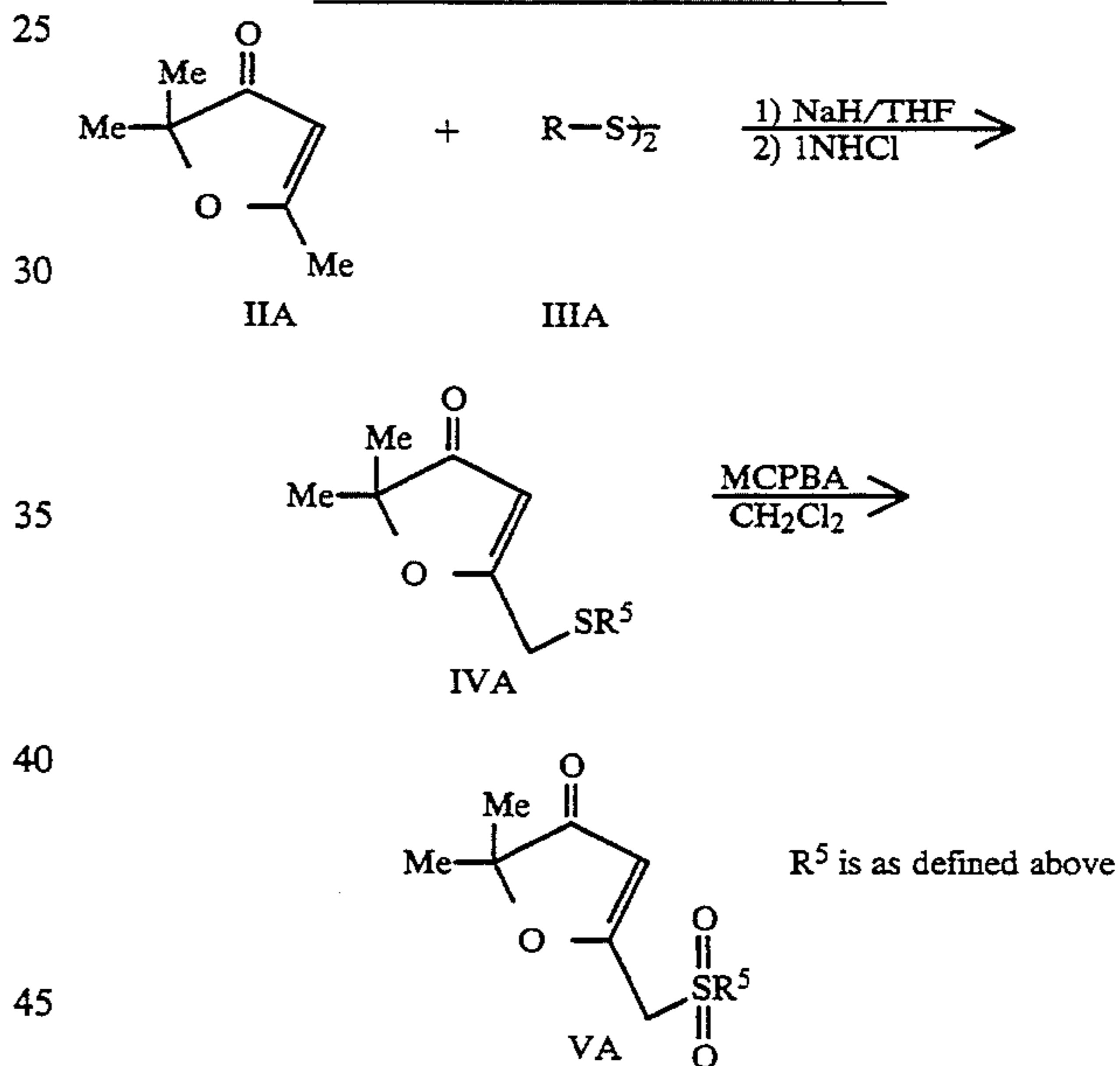
Scheme 7 (for Examples 11 to 12)
