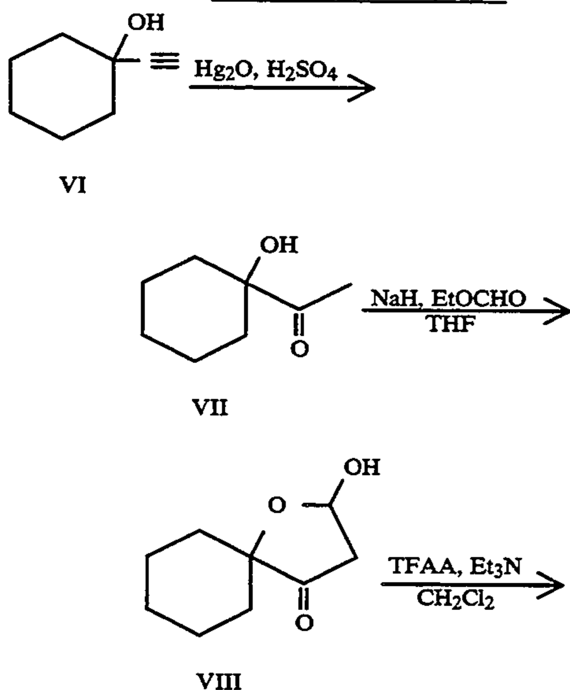
Scheme 2 (for Example 6)
