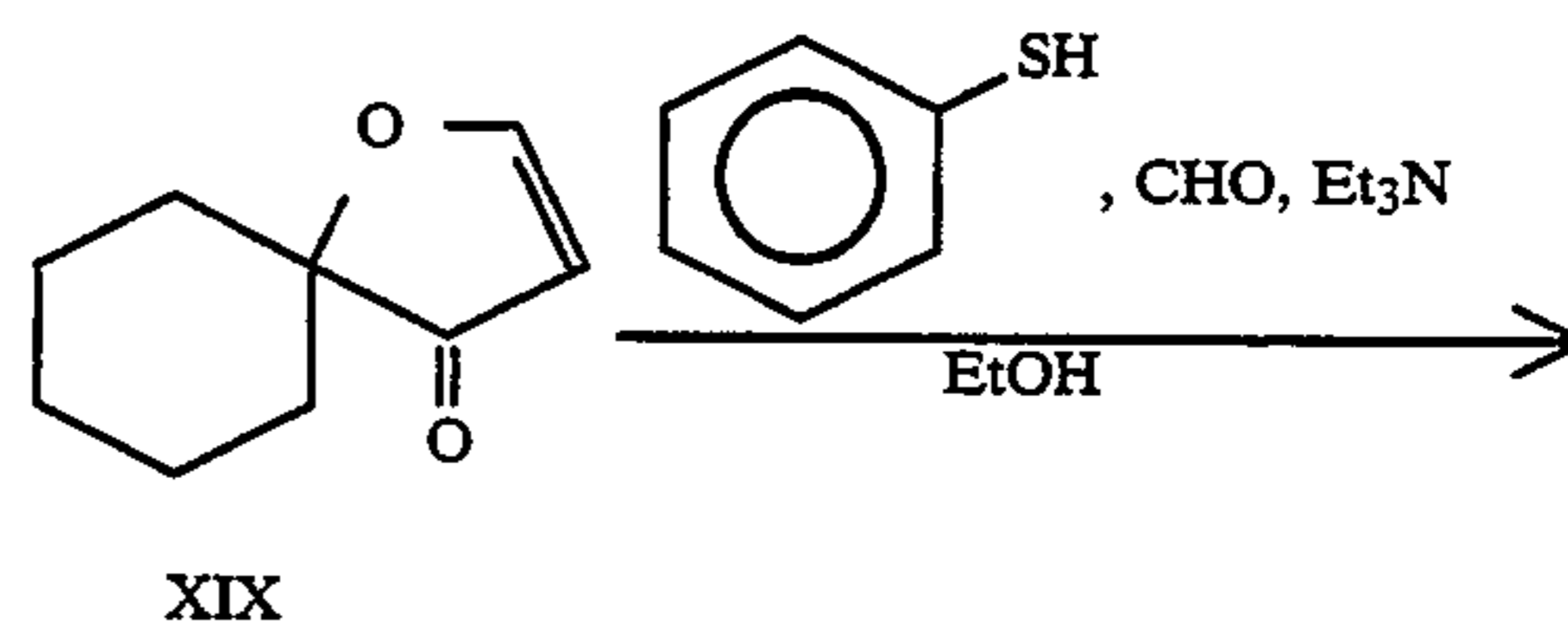
Scheme 2 (for Example 6)
