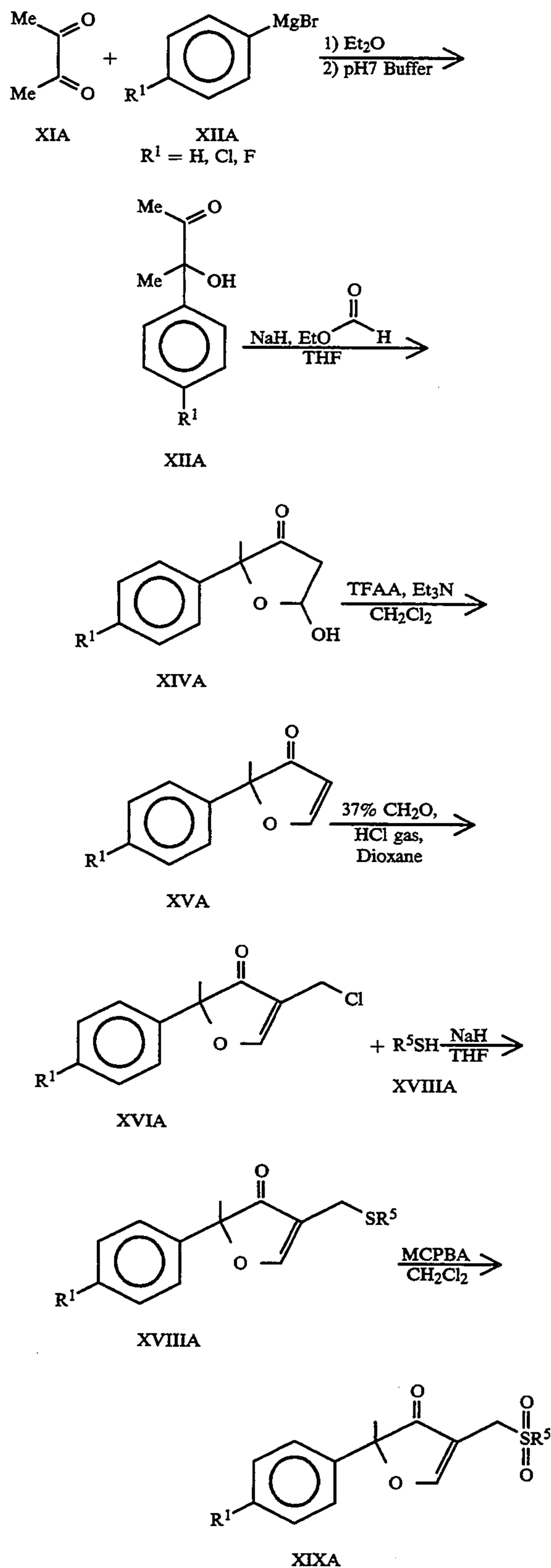
Scheme 10 (for Example 18)
