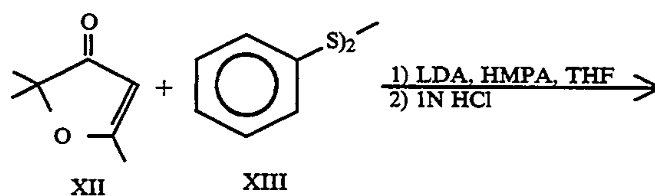
Scheme 3 (for Example 9)
