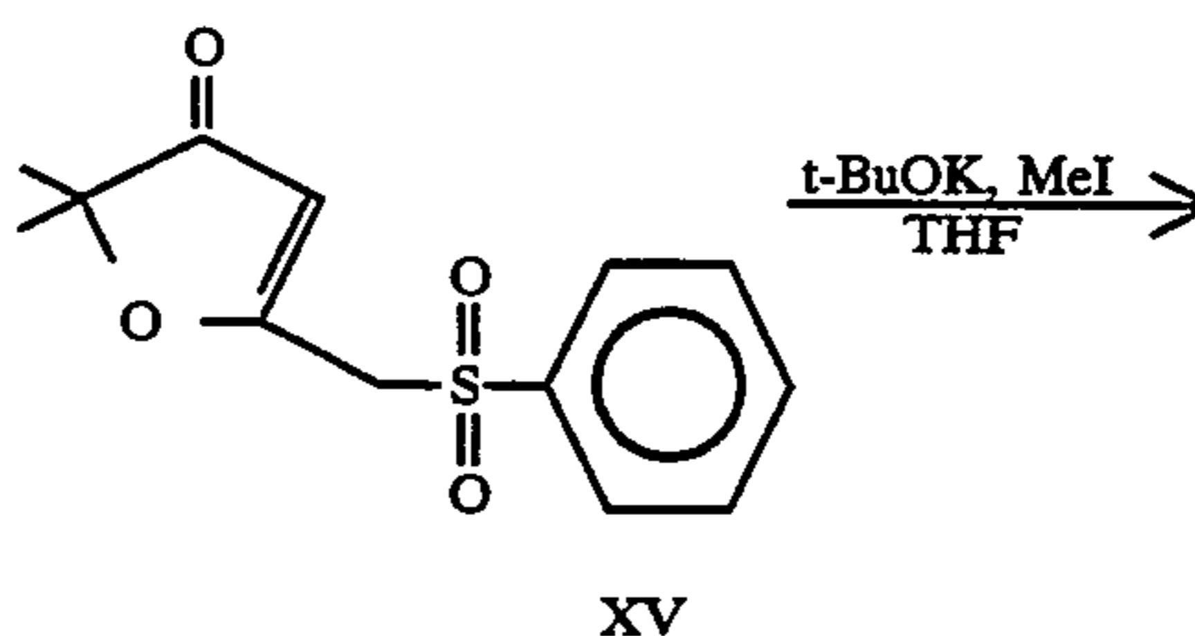
Scheme 4 (for Example 8)
