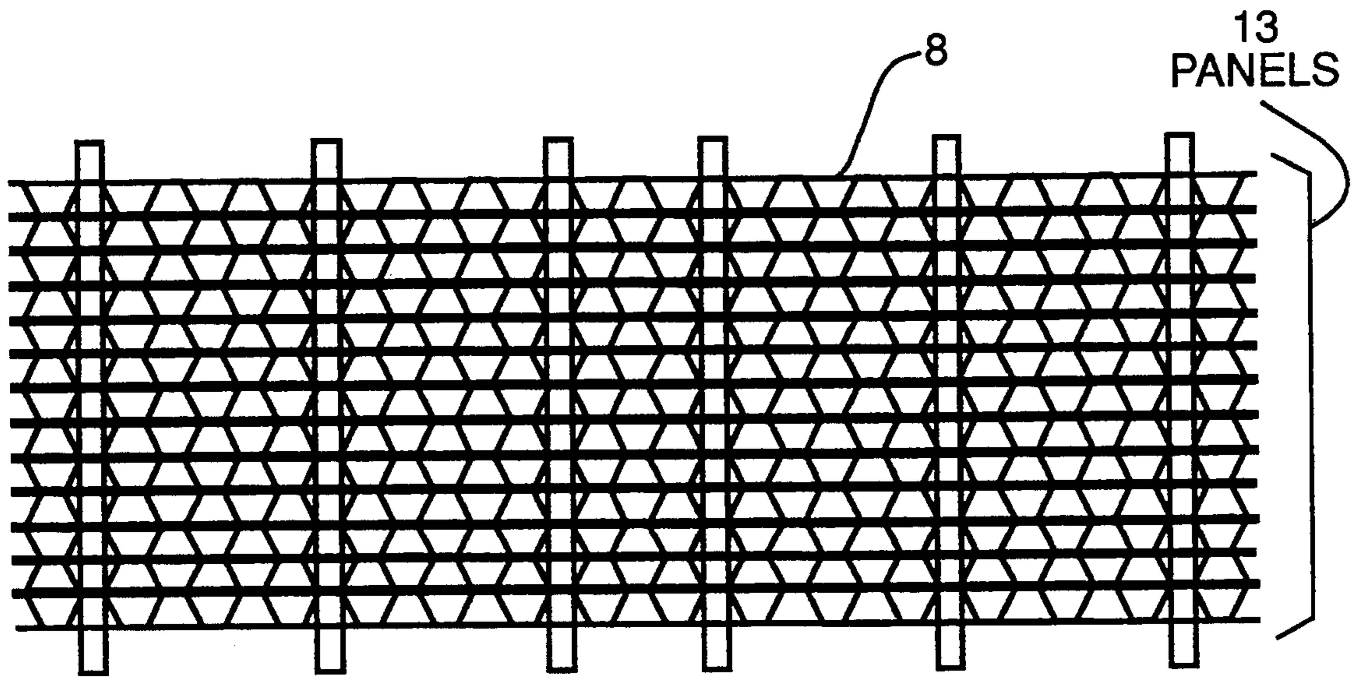
COMPLETED 15 x 48 MEDIA MODULE (2 REQUIRED PER PLANT)
