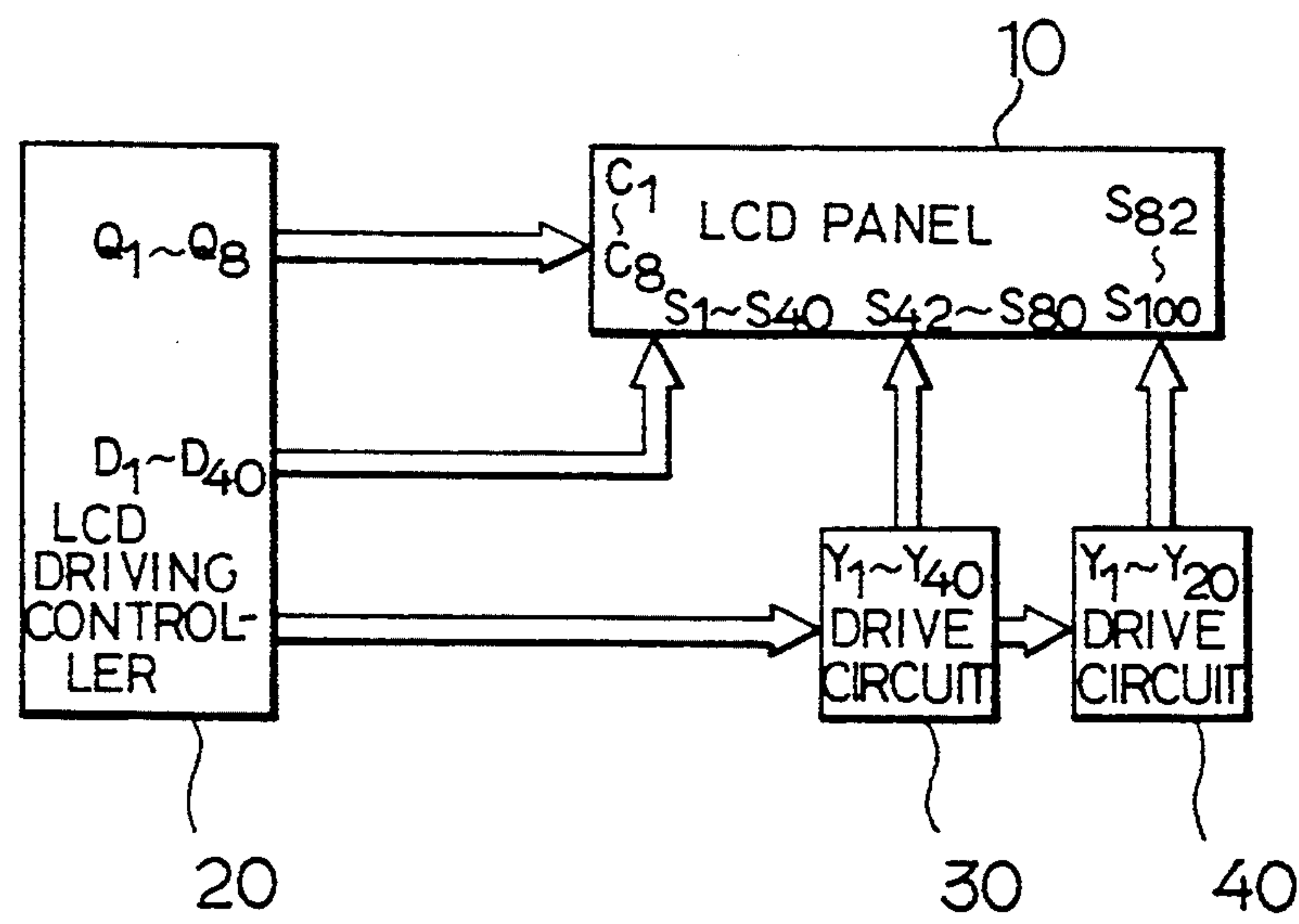
FIG. 4 PRIOR ART
