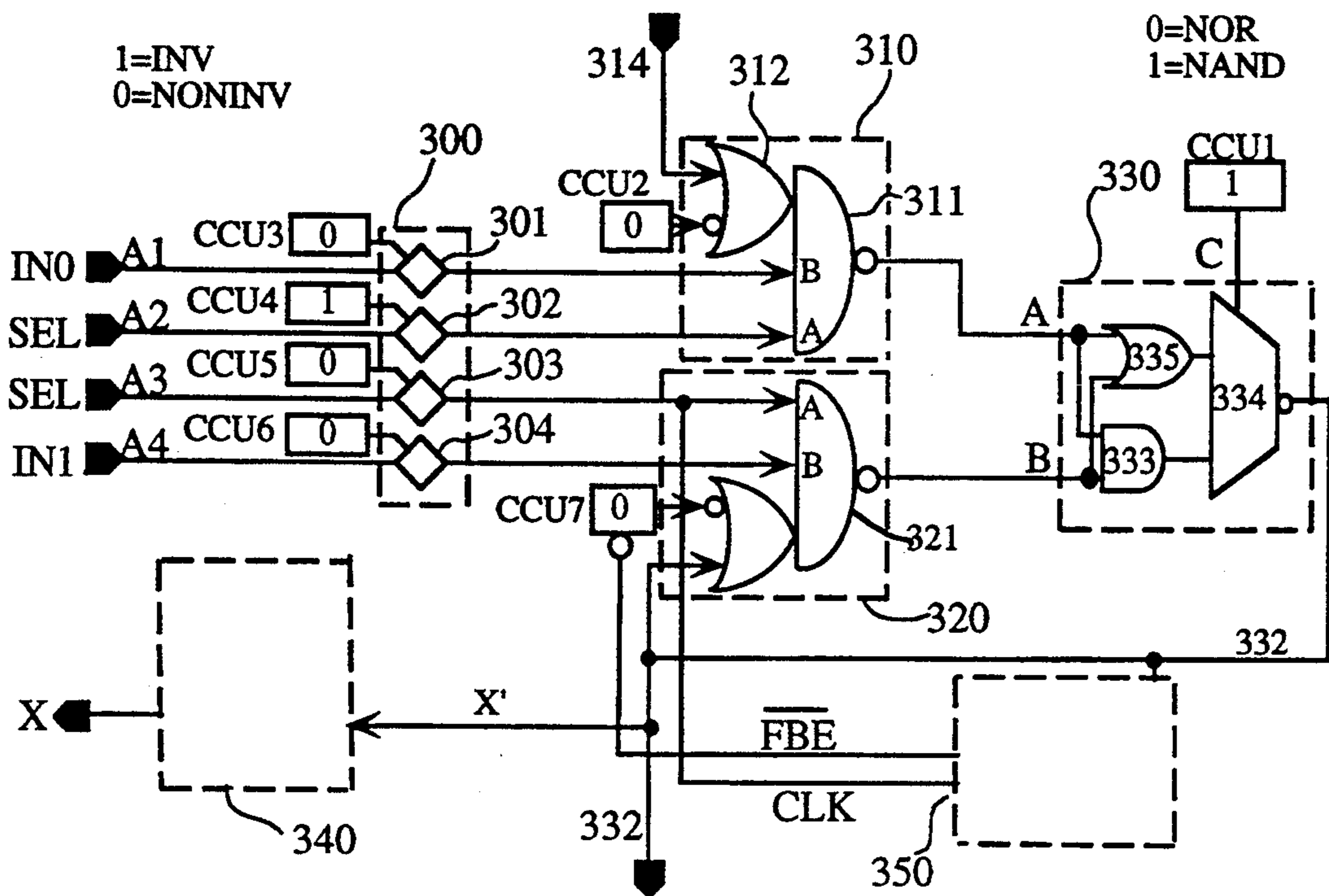
FIG. 5B MULTIPLEXER
