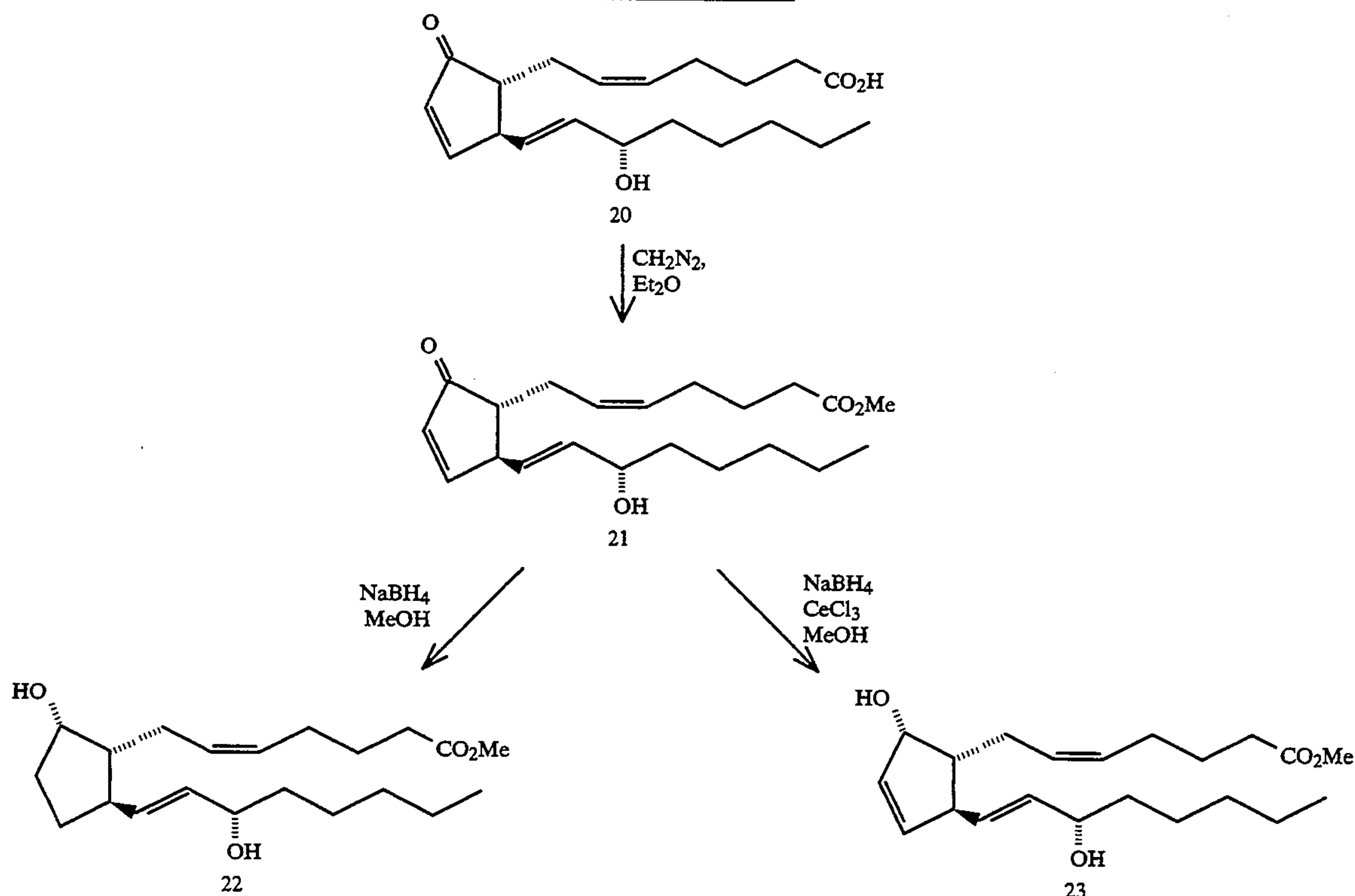
Reaction Scheme 1
