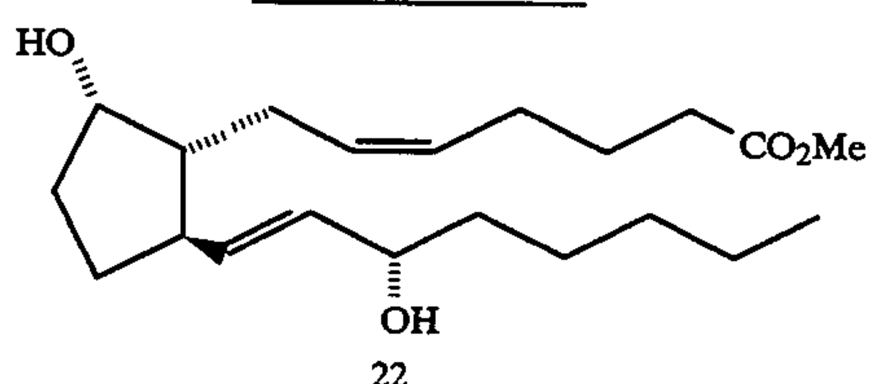
Reaction Scheme 2
