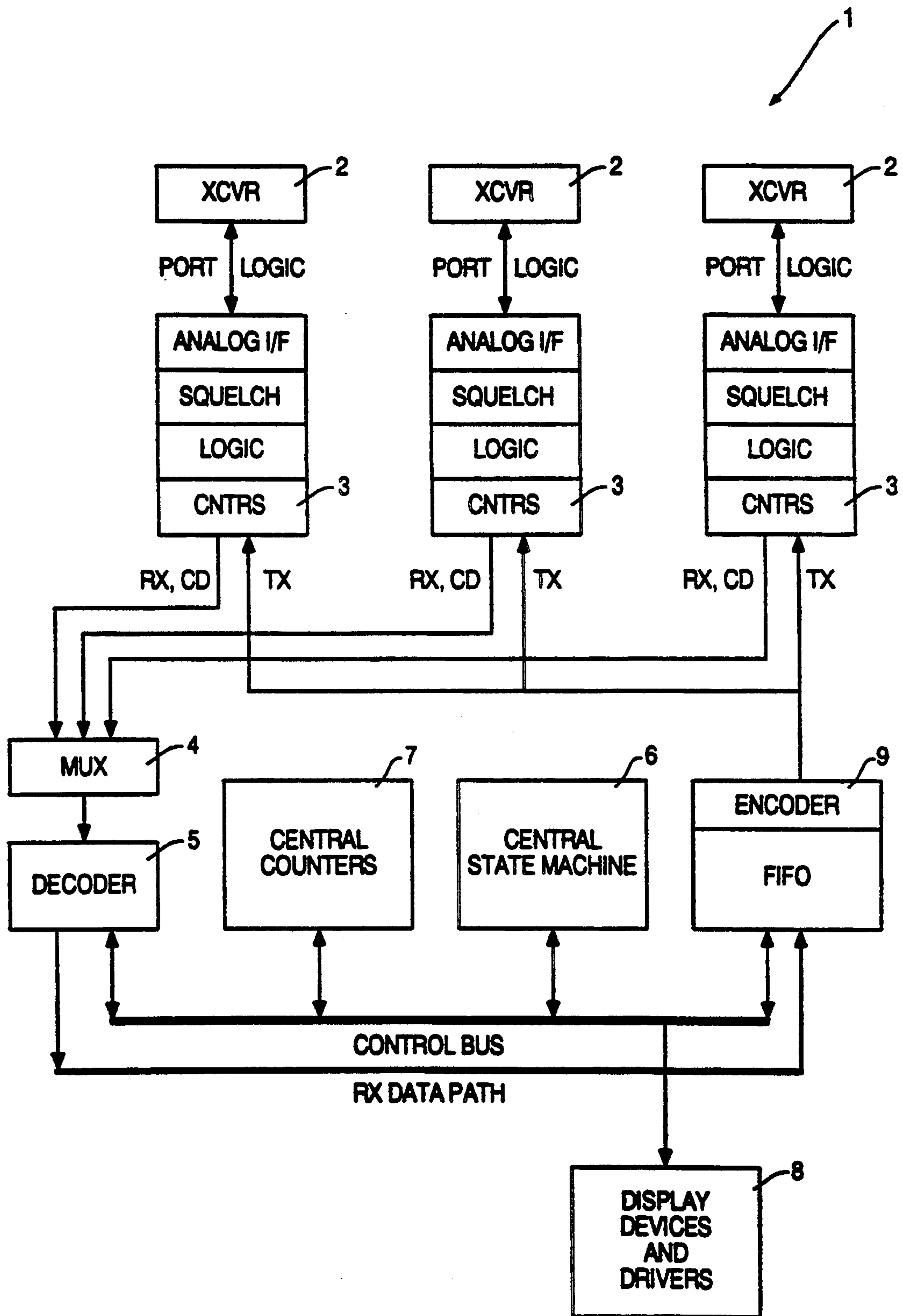
FIG. 4 (PRIOR ART)
