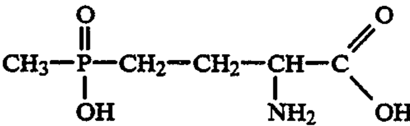
(1, 2) Ammonium (3-amino-3-carboxypropyl)- methylphosphinic acid
