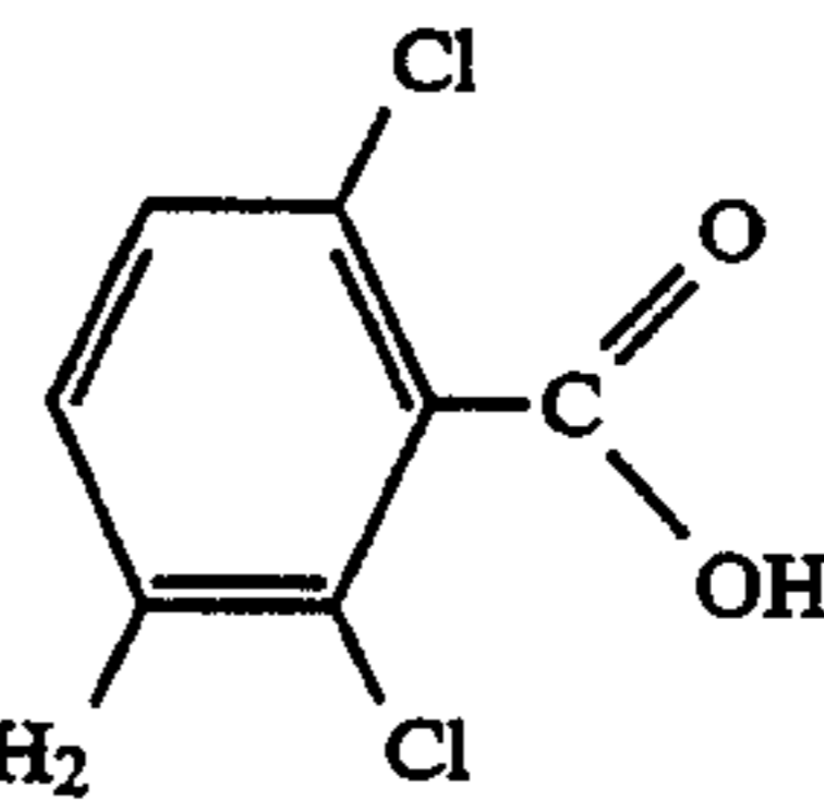
(1) 3-Amino-2,5 dichlorobenzoic acid
