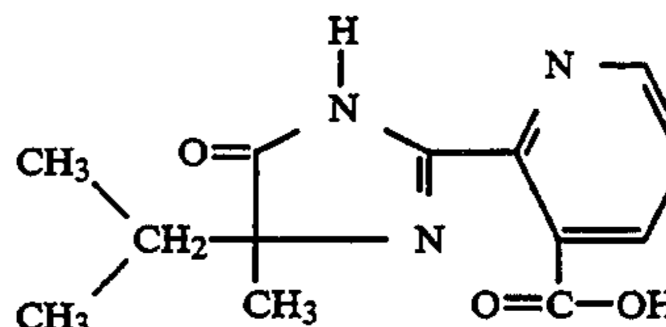
(1) 2-[4,5-dihydro-4-methyl-4-(1-methyl-ethyl)-5-oxo-1 H- imidazol-2-yl]-3-pyridinecarboxylic acid
