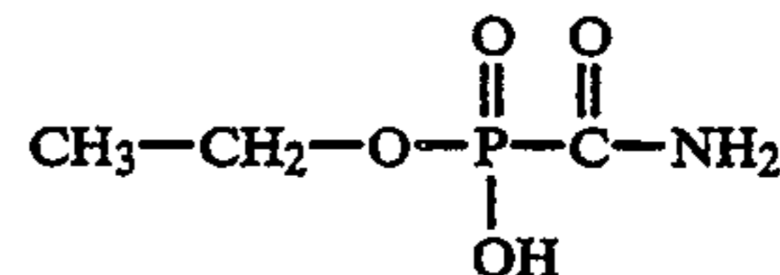
(1) (Aminocarbonyl)phosphonic acid
