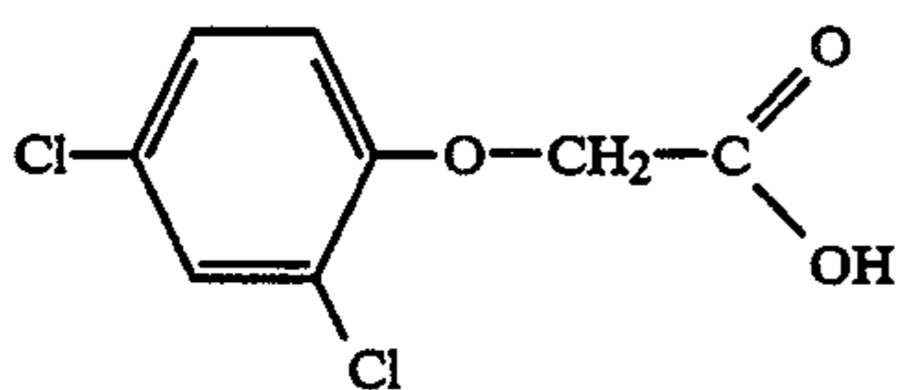
(1) 2,4-Dichlorophenoxyacetic acid
