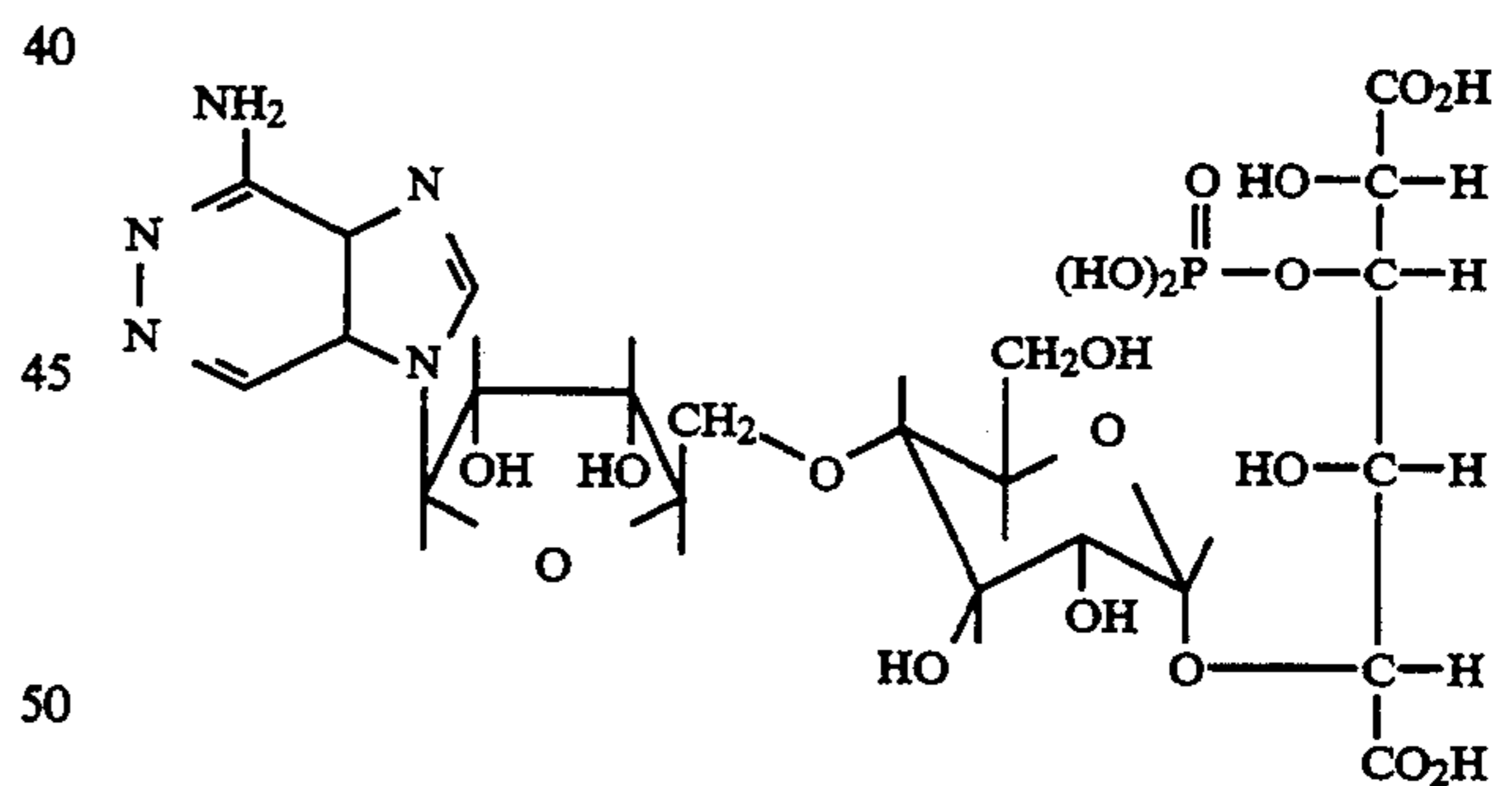
(1, 2, 3, 4)
