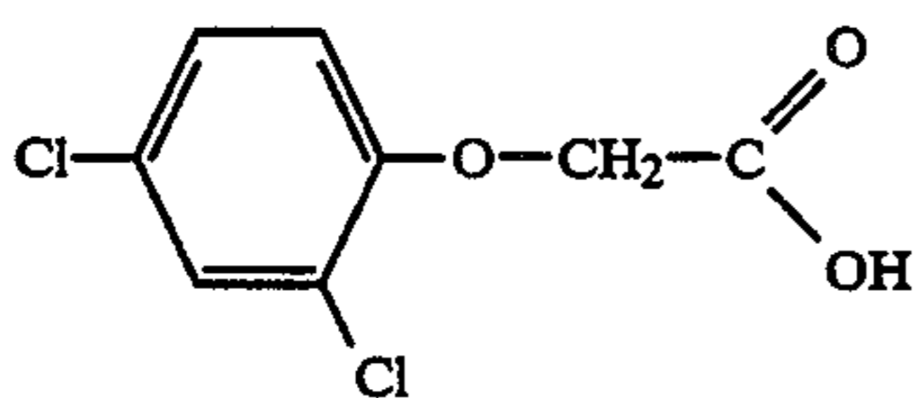
(1) 2,4-Dichlorophenoxyacetic acid
