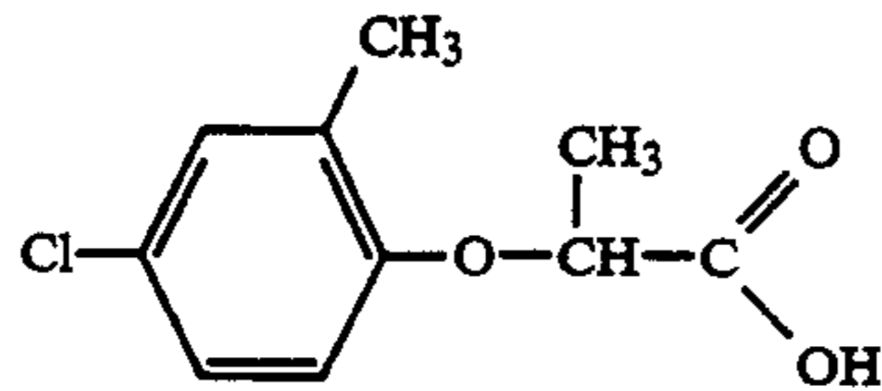
(1) 2-(2-Methyl-4-chlorophenoxy) propionic acid
