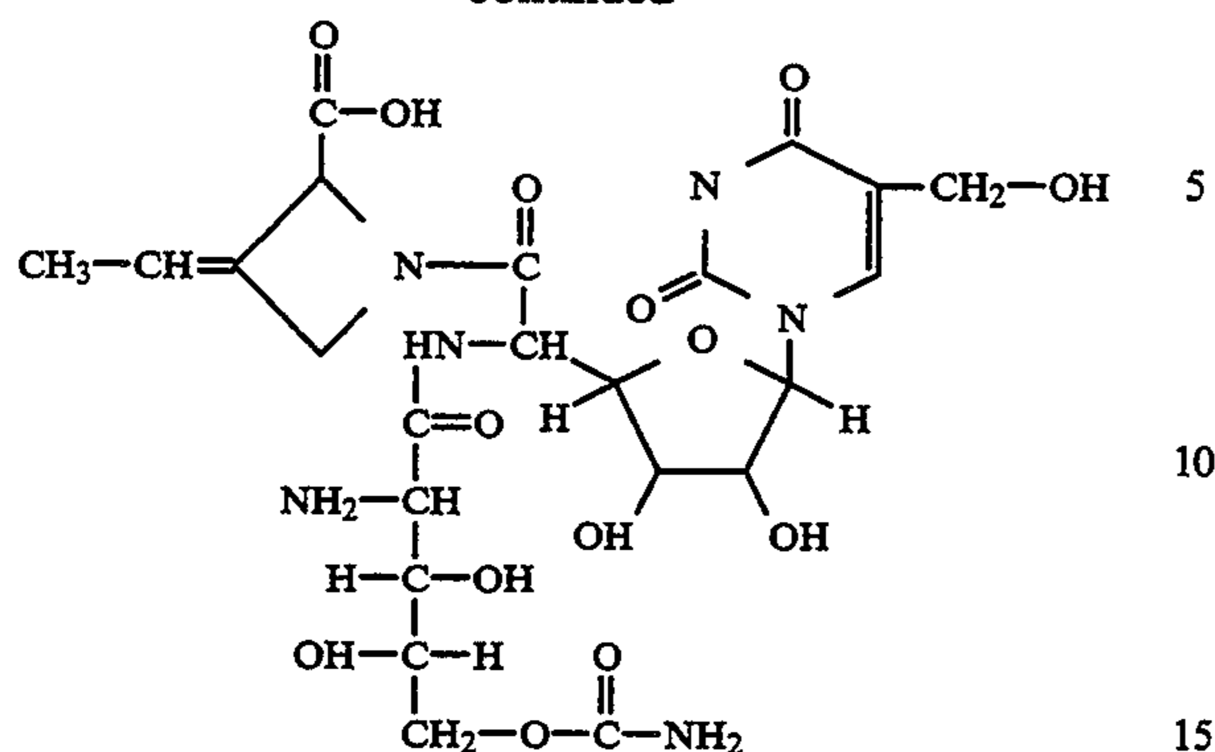
(1) 1-5-N-(5''-O-carbomonyl-2''-deoxy-L-xylonyl-5'-deoxy-beta-D-allofurano-syl-uronic acid)-5-hydroxymethyl uracid
