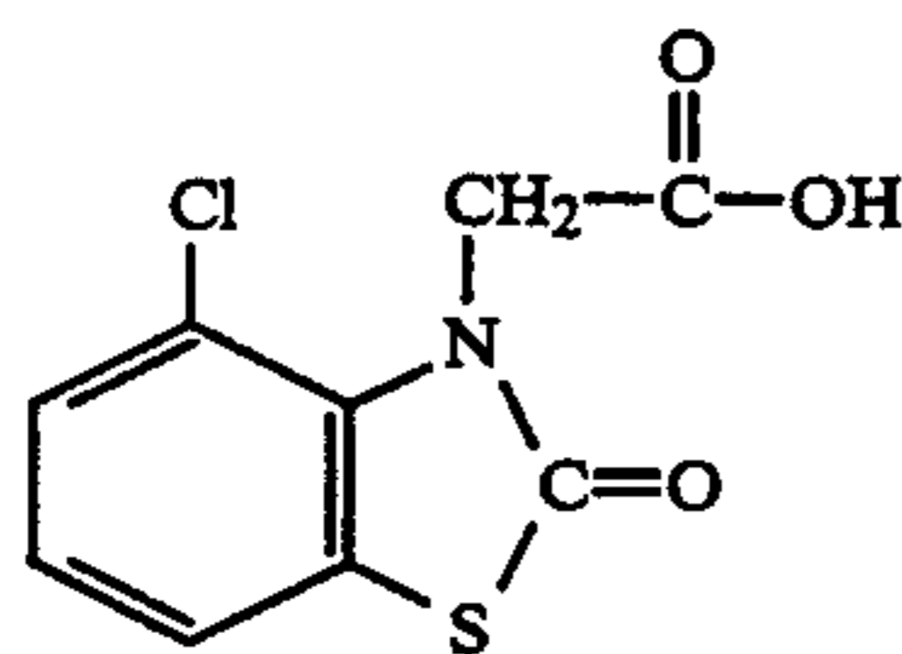
(1) 4-Chloro-2-oxobenzothiazolin-3-ylacetic acid
