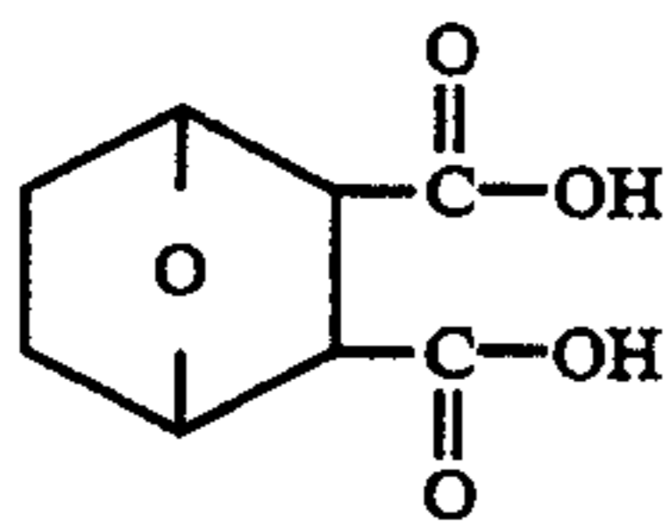
(1, 2) 7-oxabicyclo (2,2,1) heptane-2,3-dicarboxylic acid
