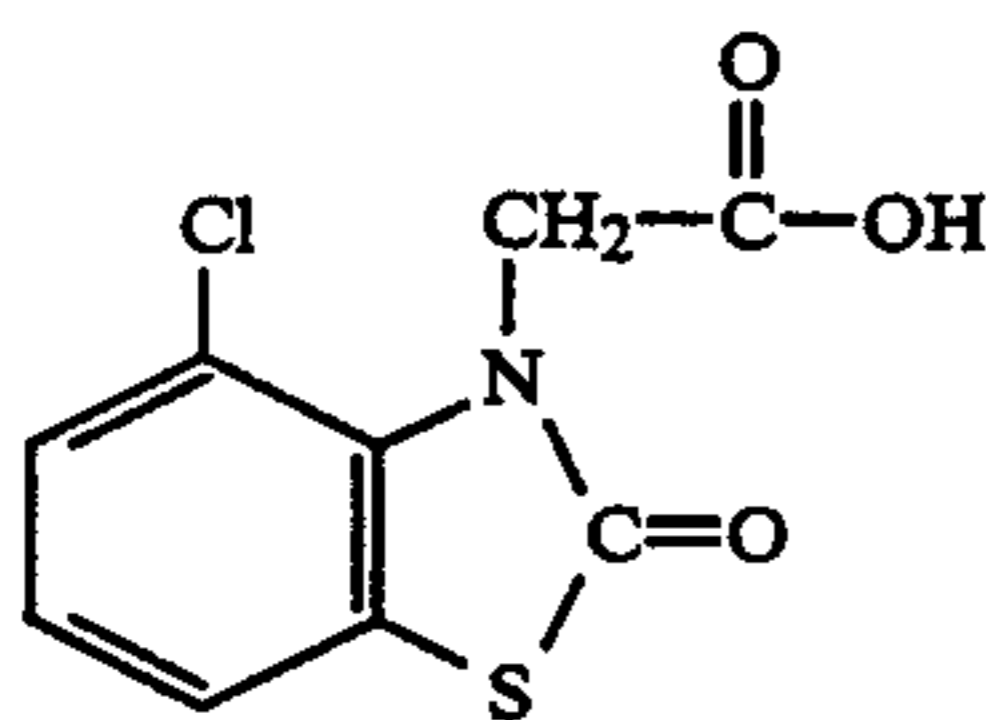
(1) 4-Chloro-2-oxobenzothiazolin-3-ylacetic acid
