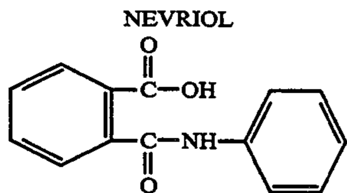
(1) N-phenylphthalamic acid
