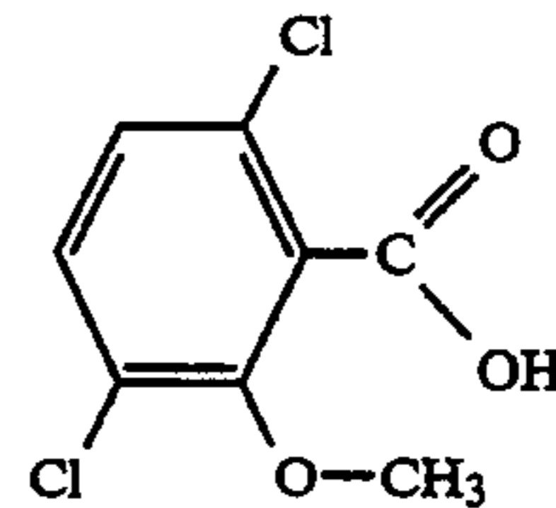
(1) 3,6-dichloro-O-anisic acid
