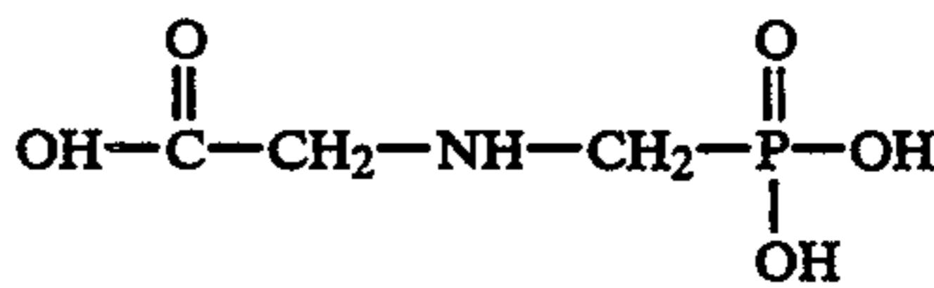
(1, 2, 3) N-(phosphonomethyl) glycine
