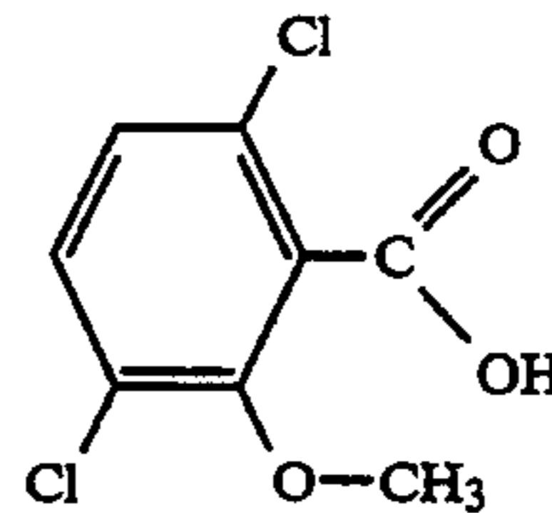
(1) 3,6-dichloro-O-anisic acid
