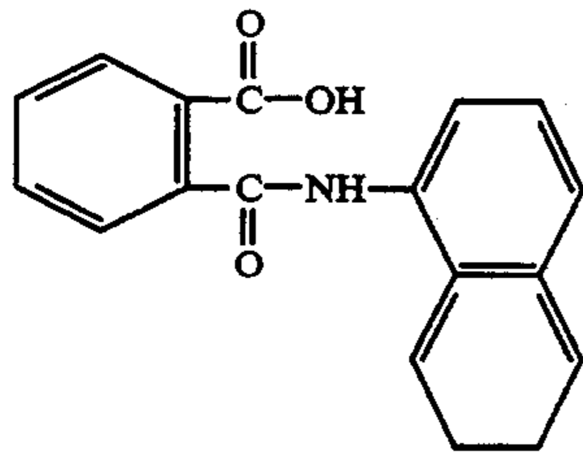
(1) N-1-Naphthylphthalamic acid
