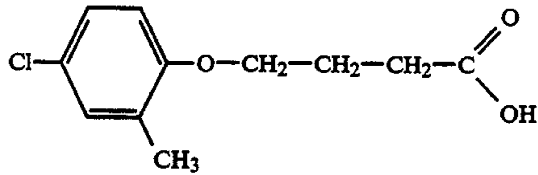
(1) 4-(2-Methyl-4-chlorophenoxy) butyric acid
