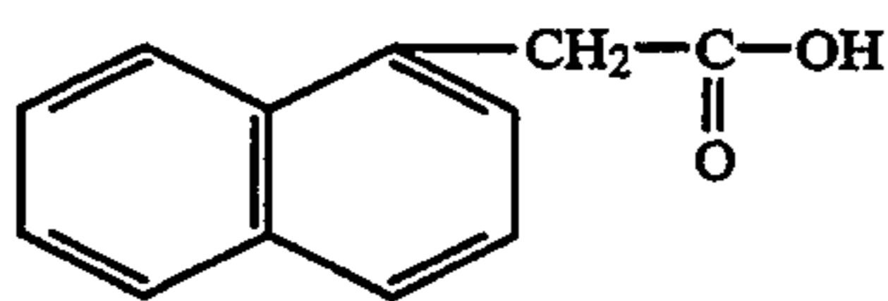
(1) 1-Naphthalene acetic acid
