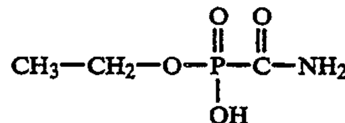
(1) (Aminocarbonyl)phosphonic acid
