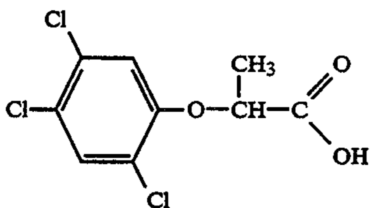
(1) 2-(2,4,5-Trichlorophenoxy) propionic acid
