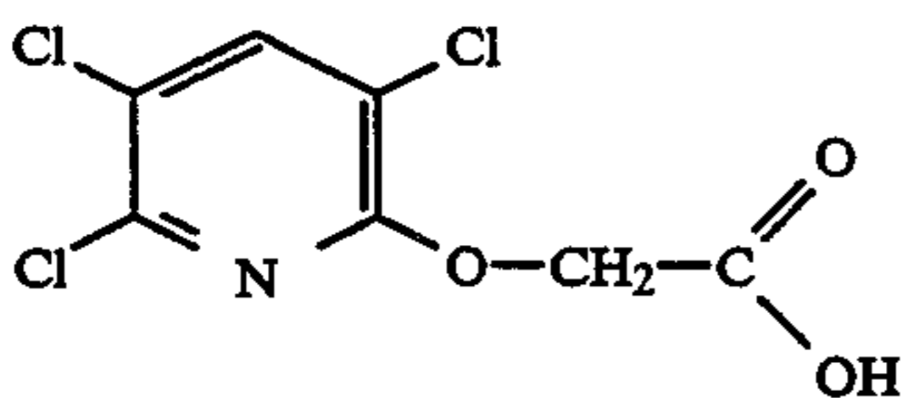
(1) 3,5,6-trichloro-2-pyridyl-oxyacetic acid
