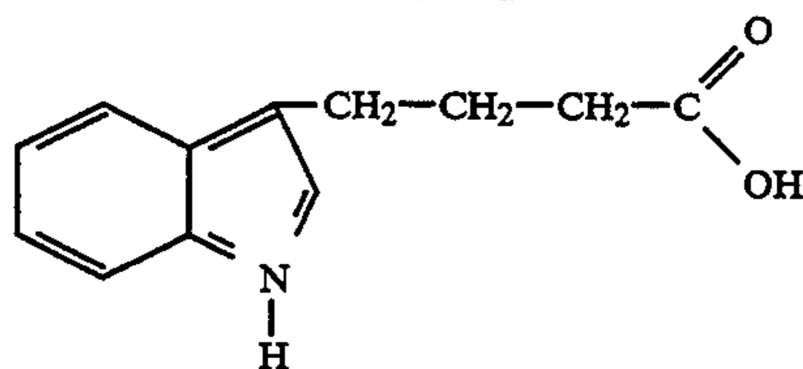
(1) 3-Indolebutyric acid
