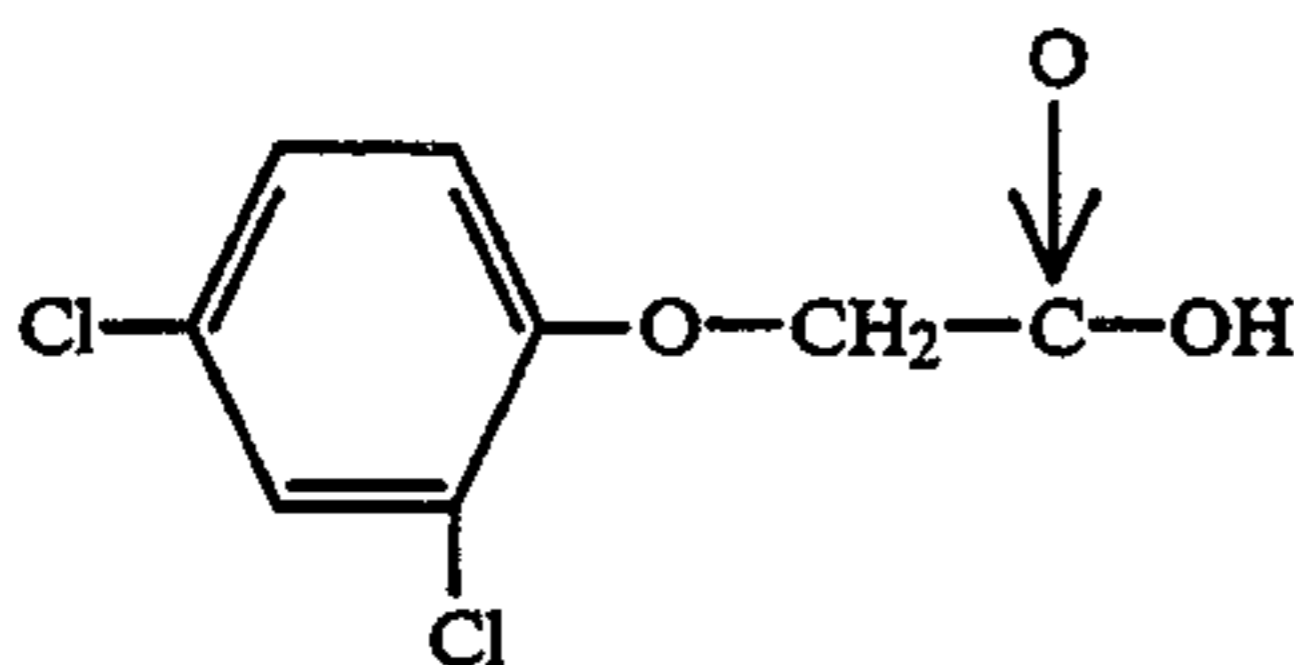
(1) 2,4-dichlorophenoxypropionic acid
