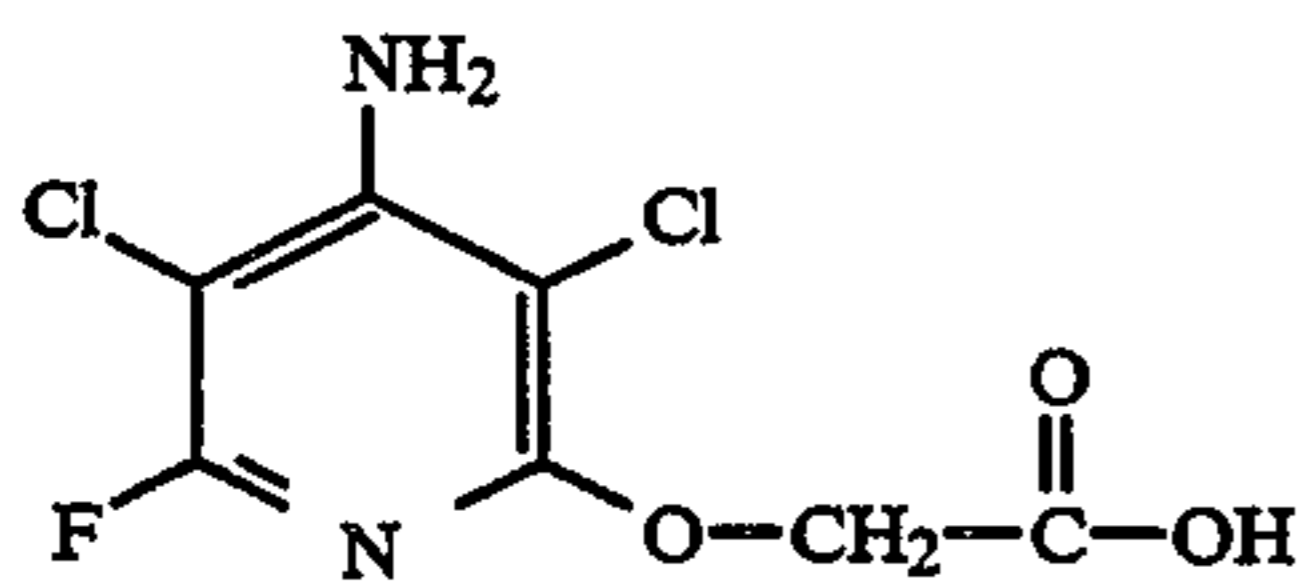
(1) 4-amino-3,5-dichloro-6-fluoro-2-pyridyloxyacetic acid
