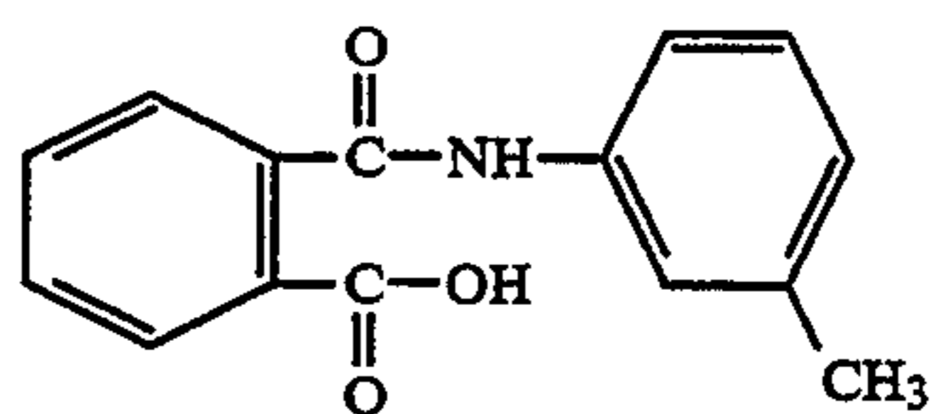
(1) N-m-tolylphthalamic acid
