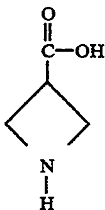
(1) Azetidine-3-carboxylic acid
