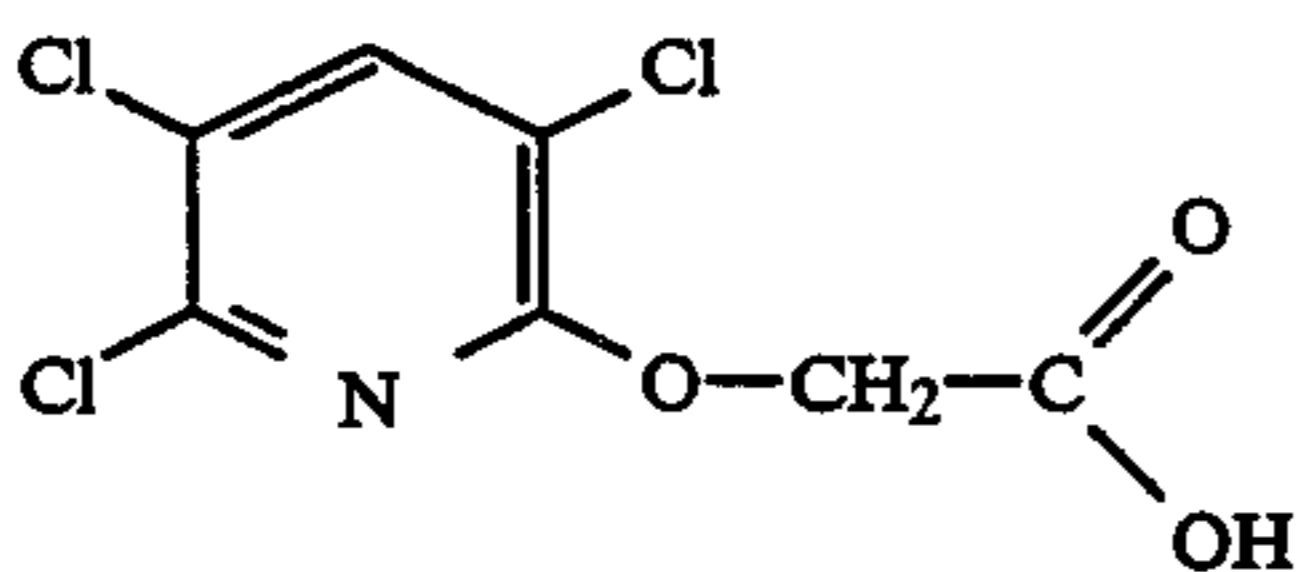
(1) 3,5,6-trichloro-2-pyridyl-oxyacetic acid
