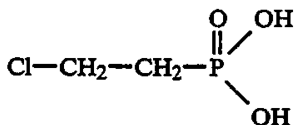
(1, 2) (2-Chloroethyl) phosphonic acid
