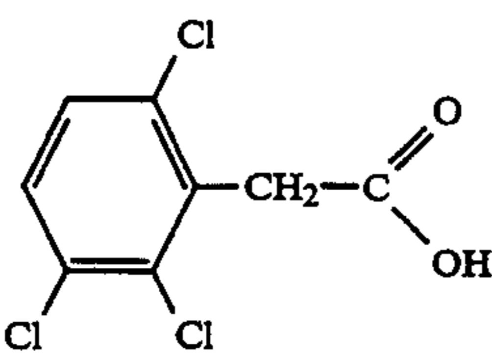
(1) 2,3,6-Trichlorophenylacetic acid
