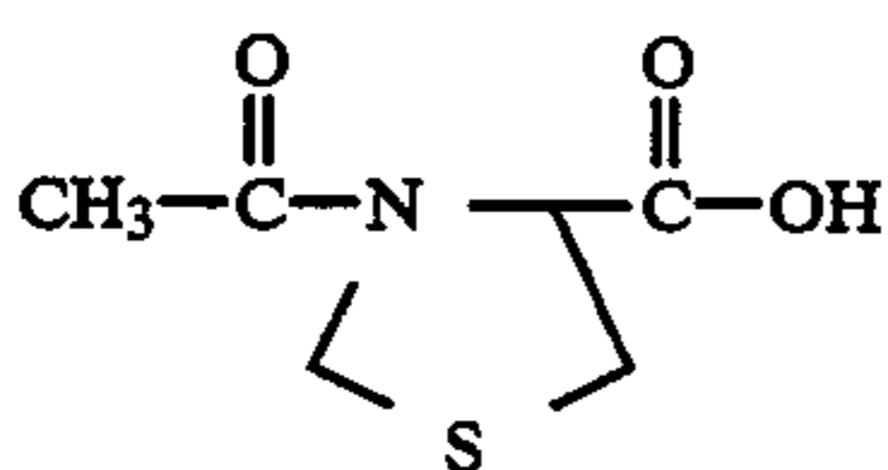
(1) 3-Acetyl-4 thiazolidine-carboxylic acid
