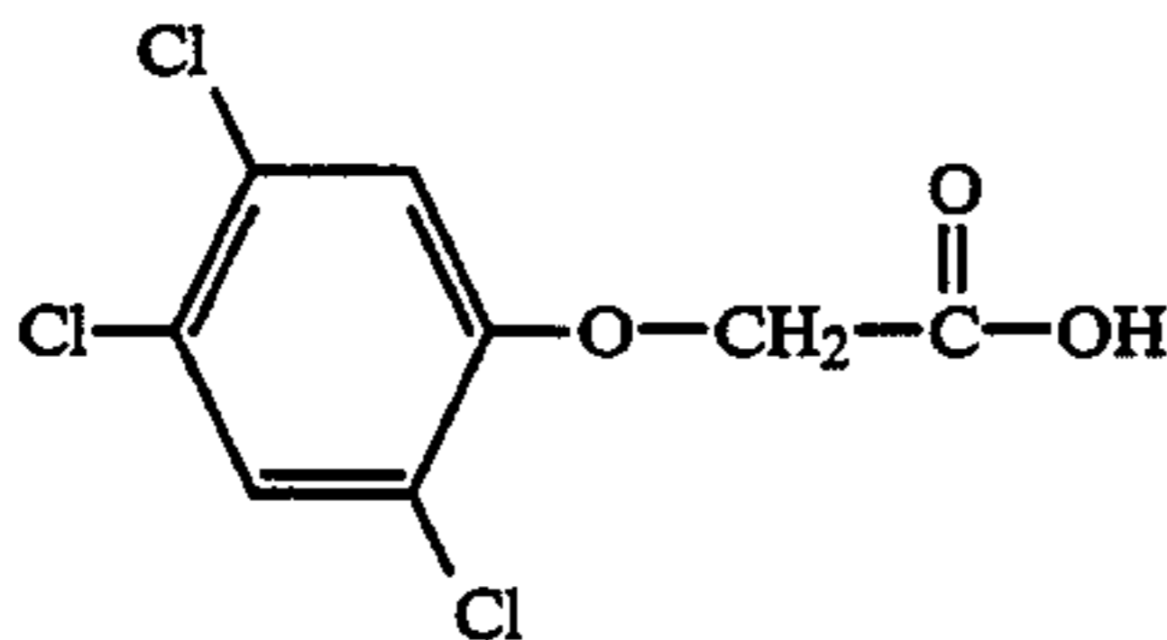
(1) 2,4,5-Trichlorophenoxyacetic acid
