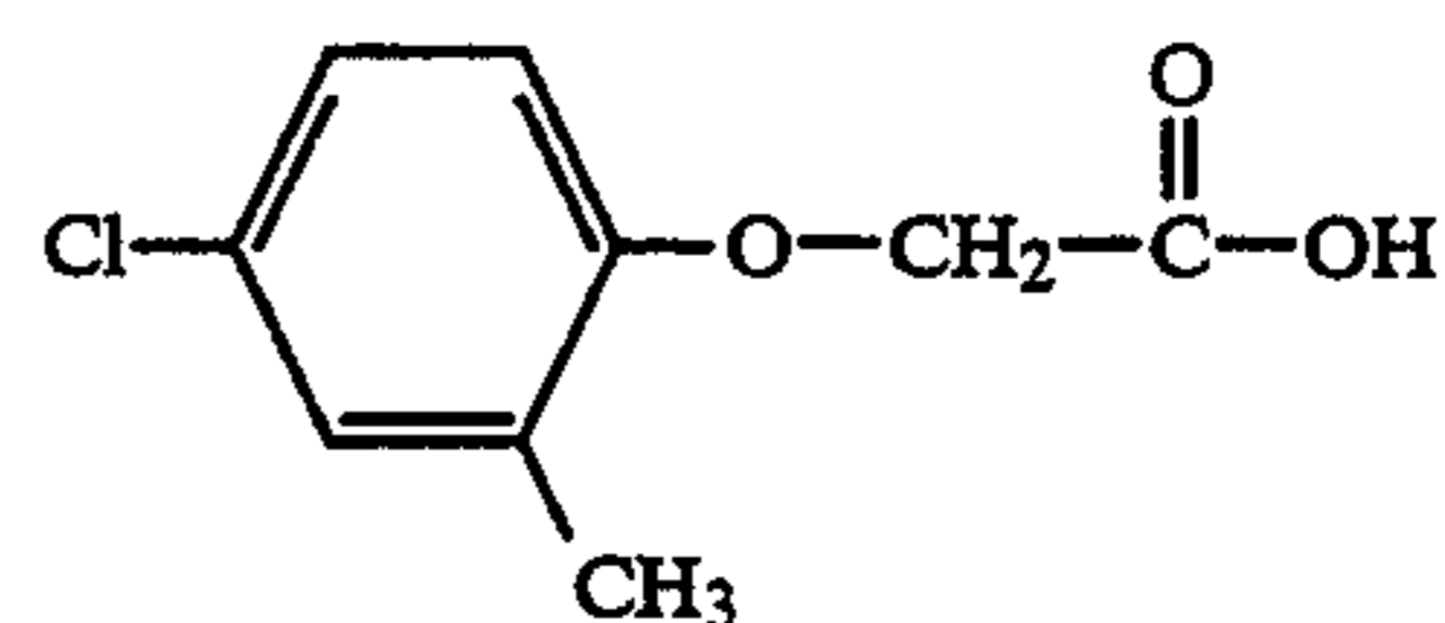
(1) 2-Methyl-4-chlorophenoxyacetic acid
