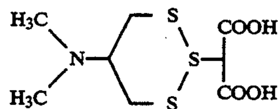
(1, 2) N,N-Dimethyl-1,2,3,-trithian-5-ylamine hydrogenoxalate
