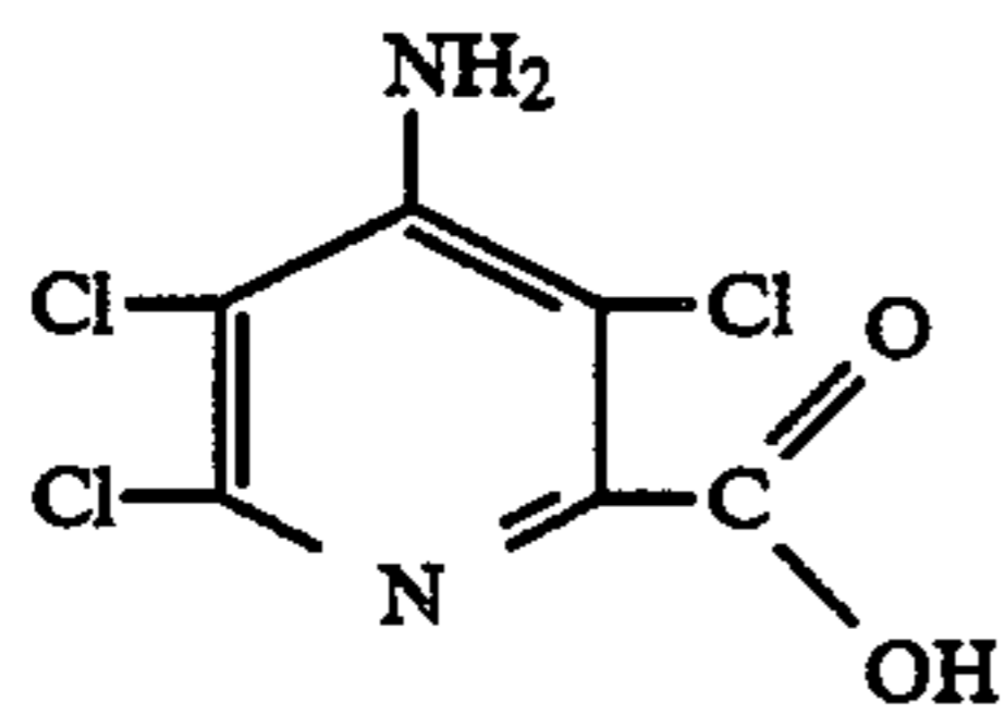
(1) 4,Amino-3,5,6-trichloro-picolinic acid
