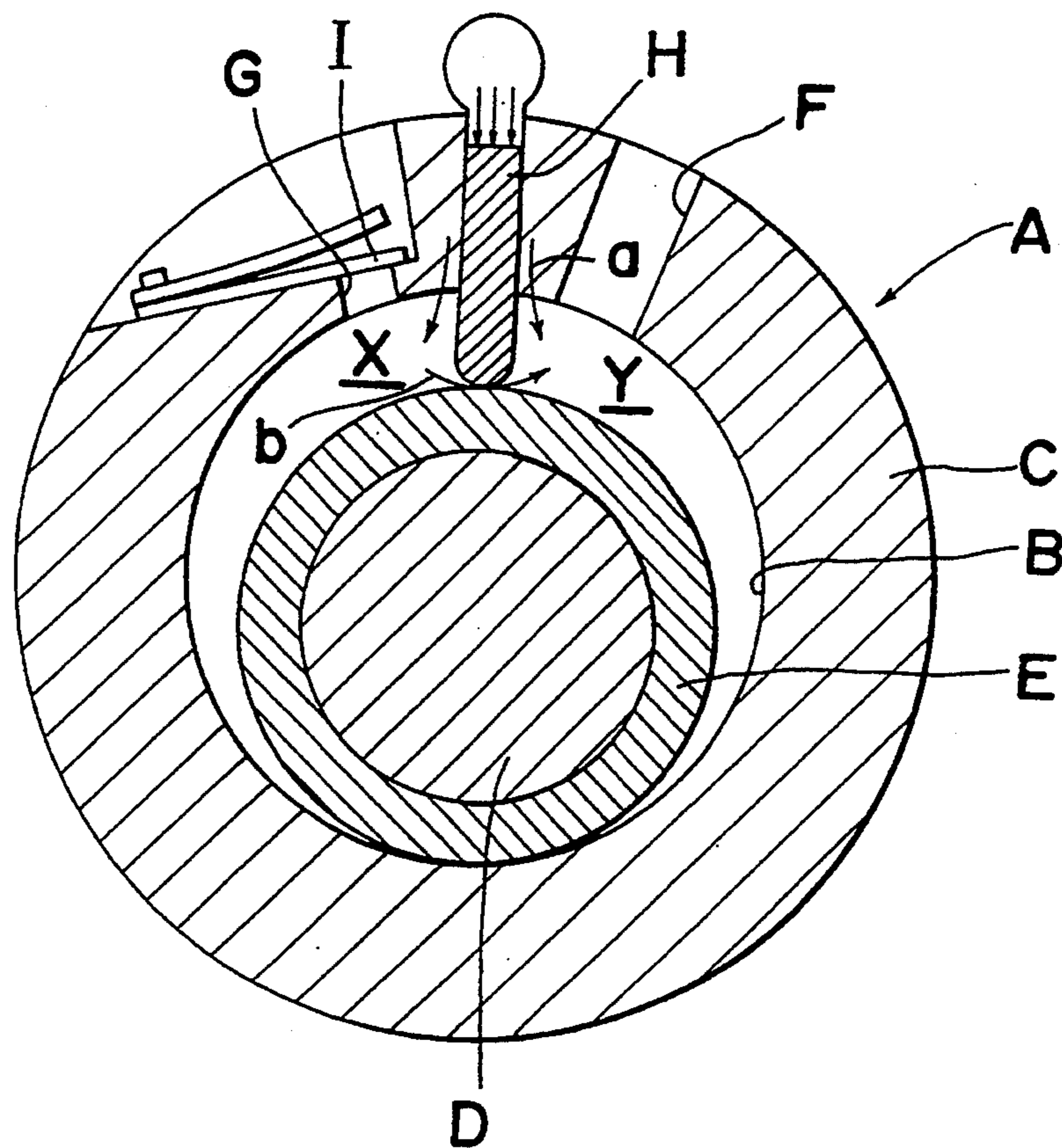
Fig. 24 PRIOR ART
