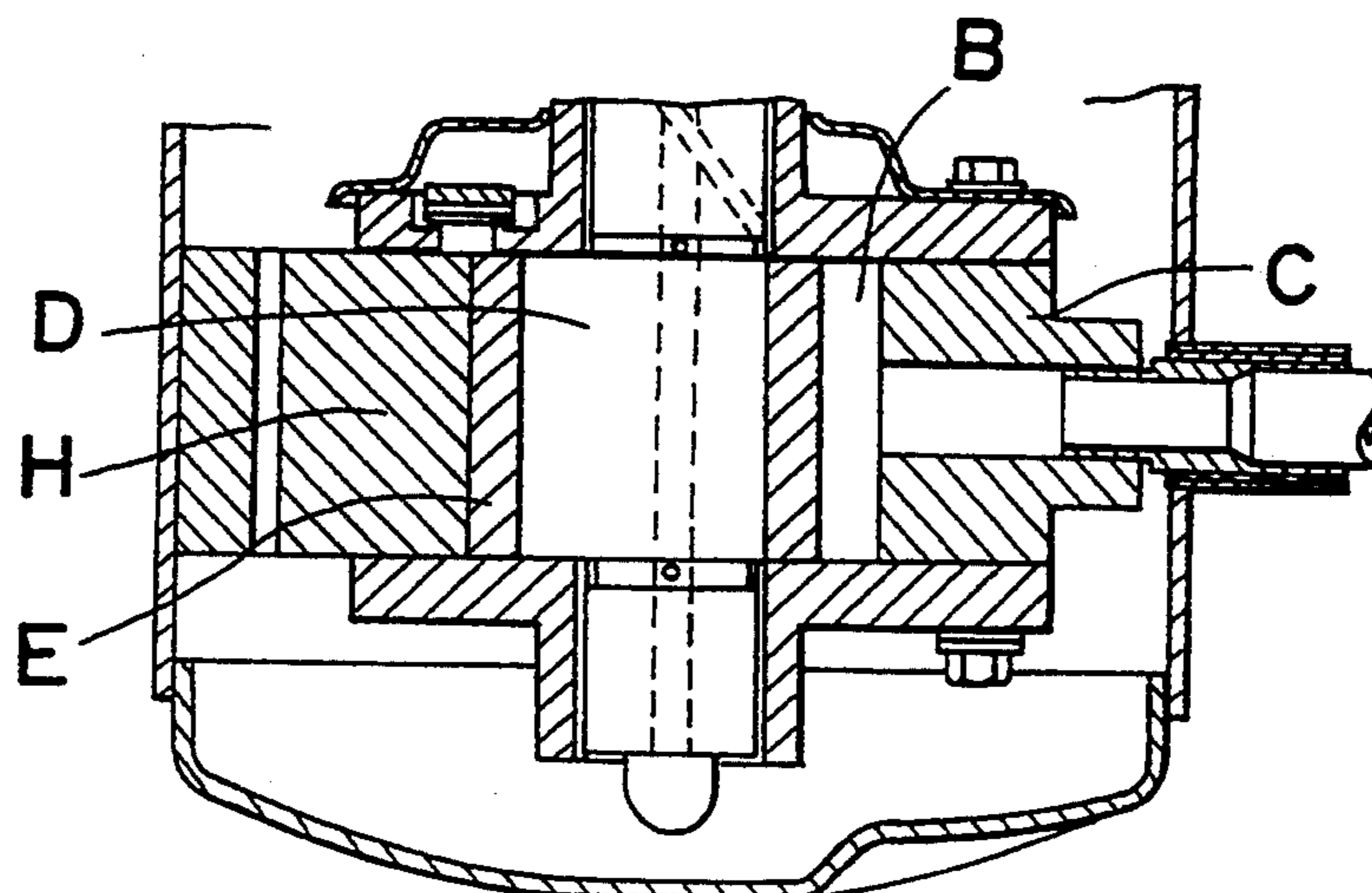
Fig. 25 PRIOR ART
