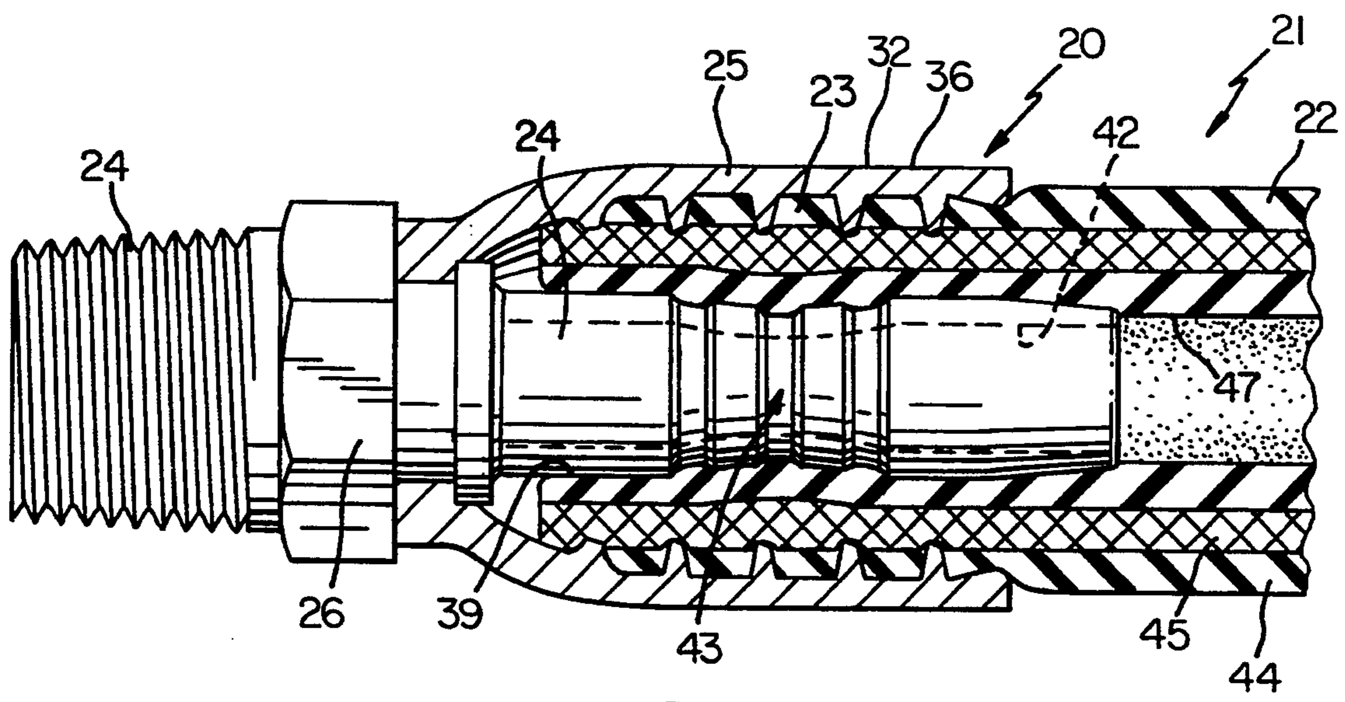
FIG. 2 PRIOR ART
