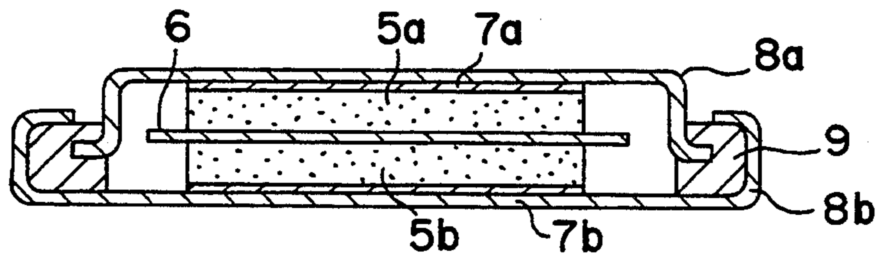
FIG. 2 PRIOR ART
