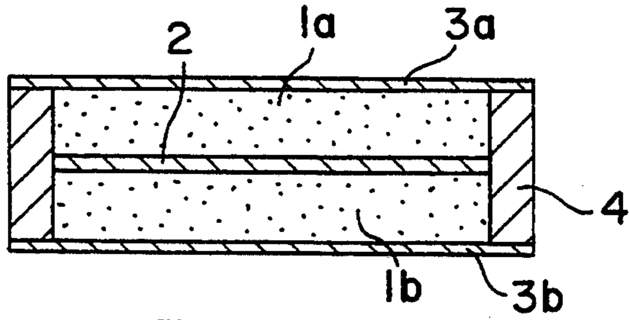
FIG. 1 PRIOR ART
