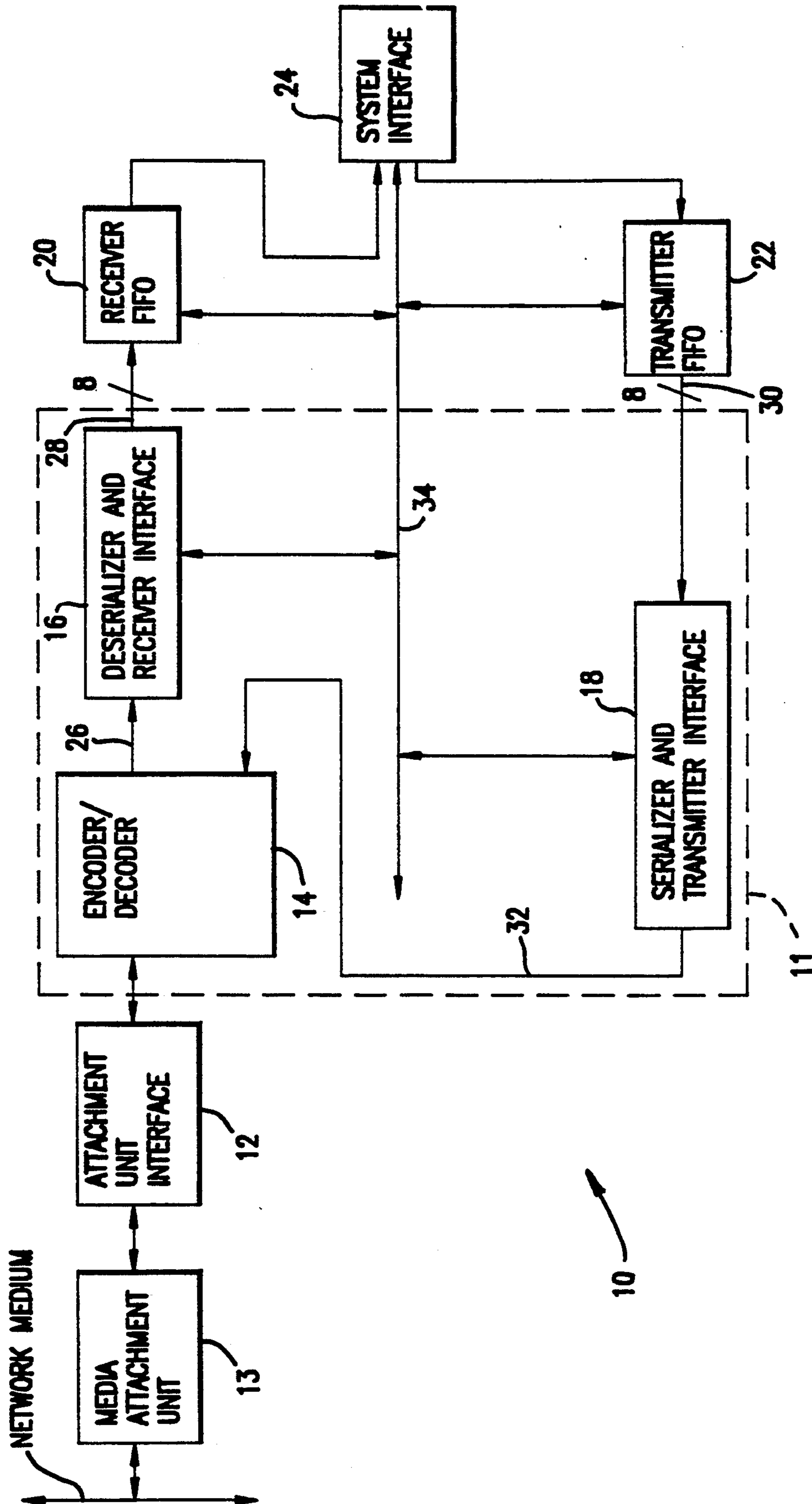
FIG. 1 (PRIOR ART)
