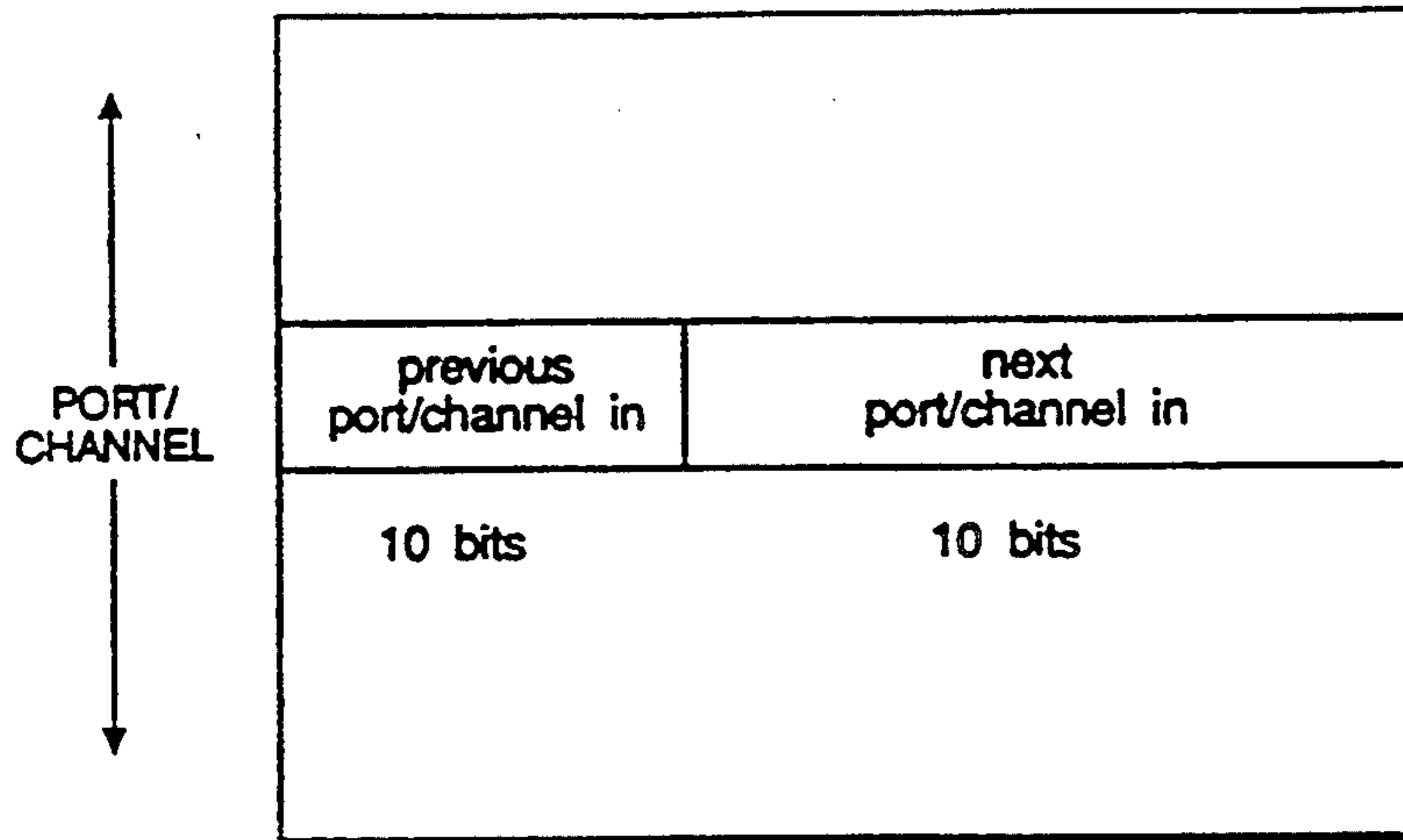
FIG. 7b NEXT CHANNEL IN LINK LIST TABLE
