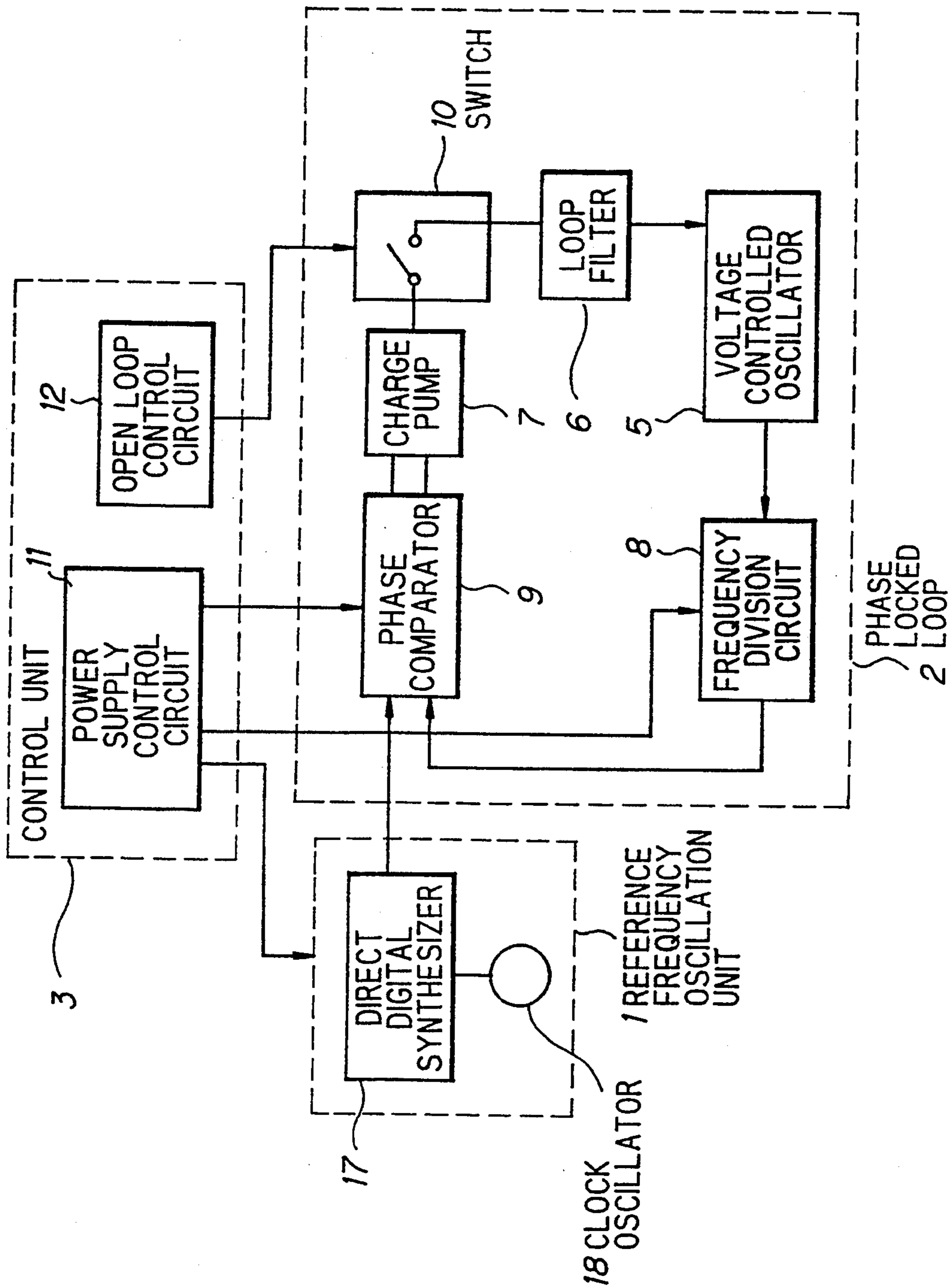
FIG. 1 PRIOR ART
