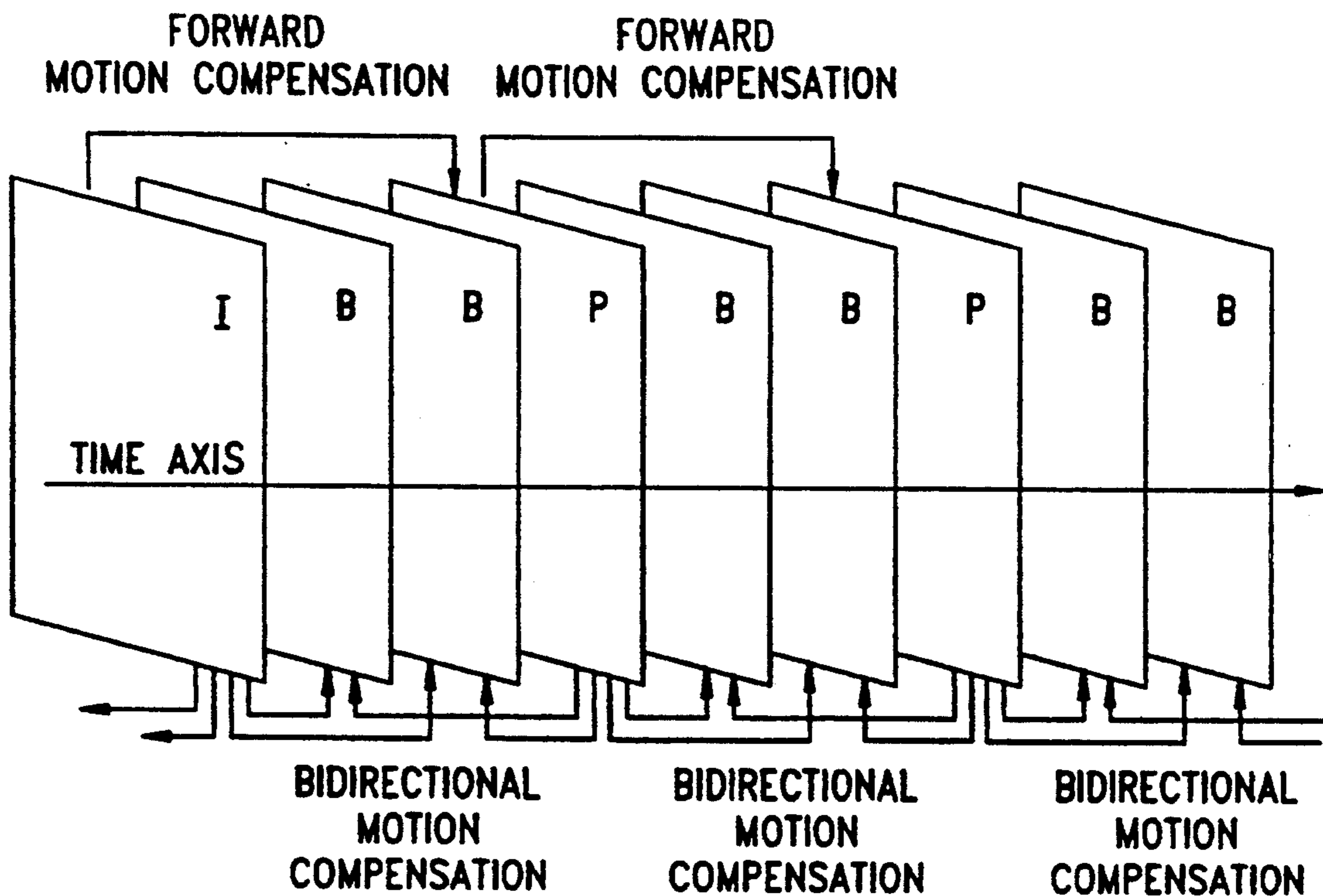
FIG. 5 PRIOR ART
