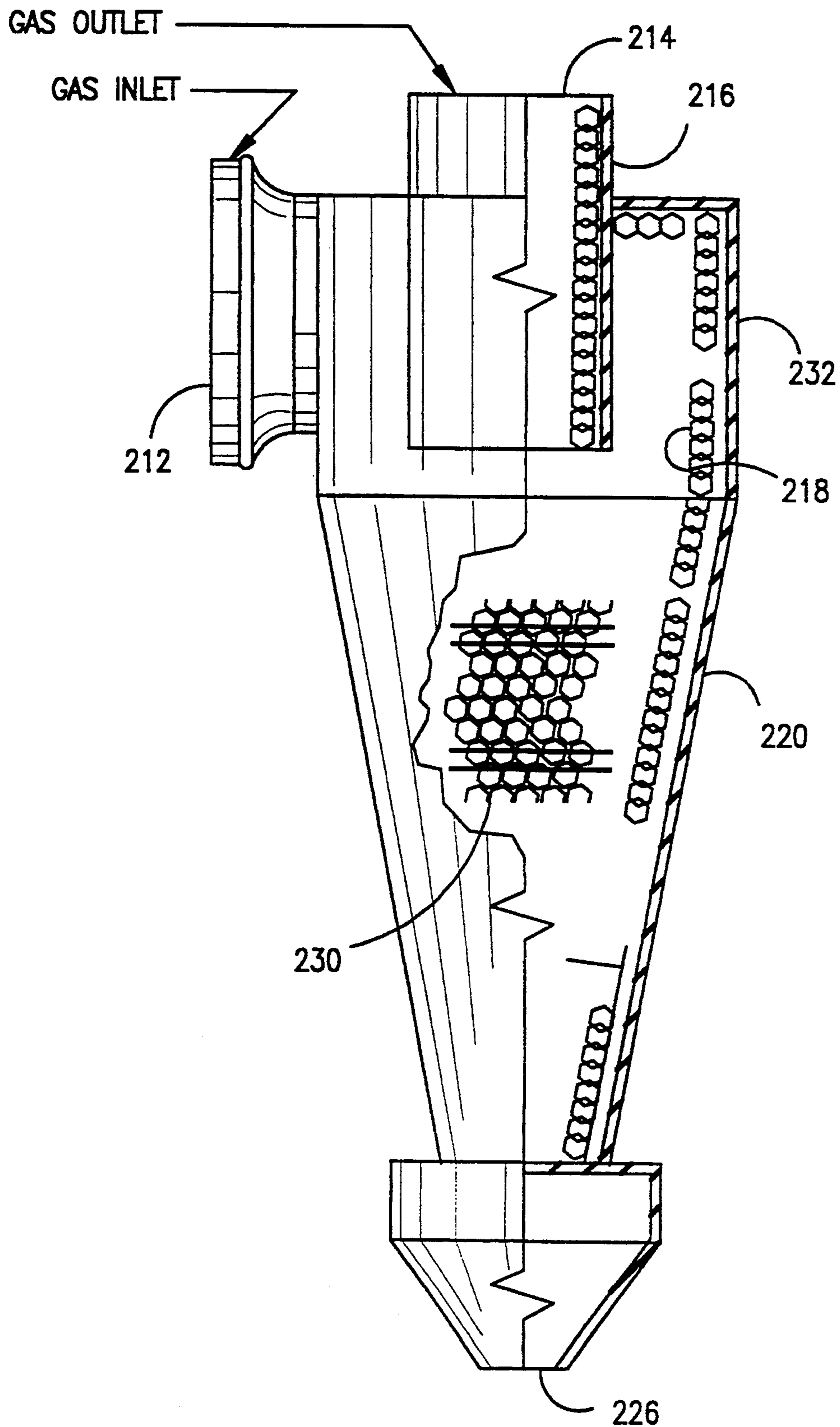
FIG. 2 (PRIOR ART)
