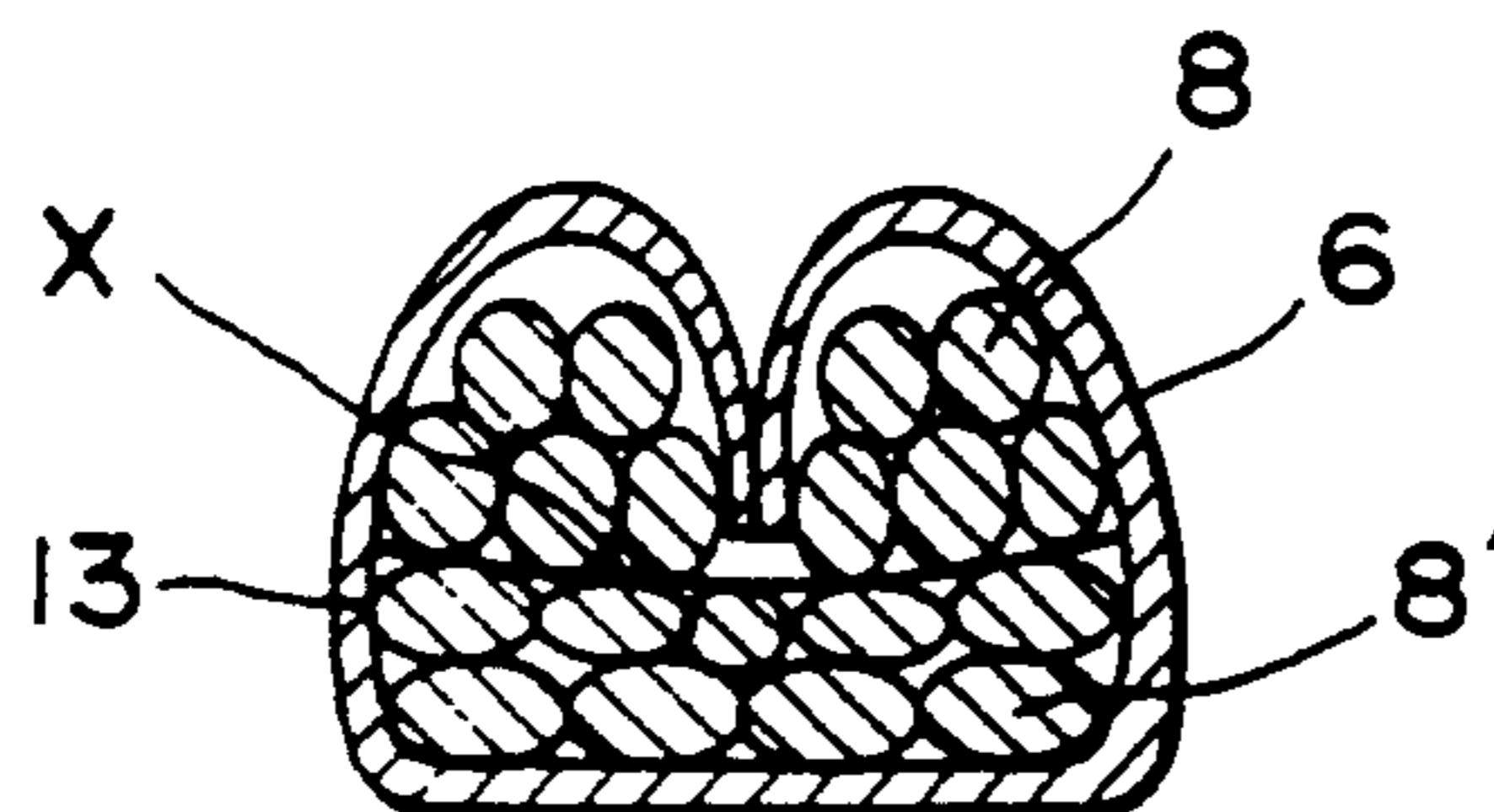
Fig. 17 Prior Art
