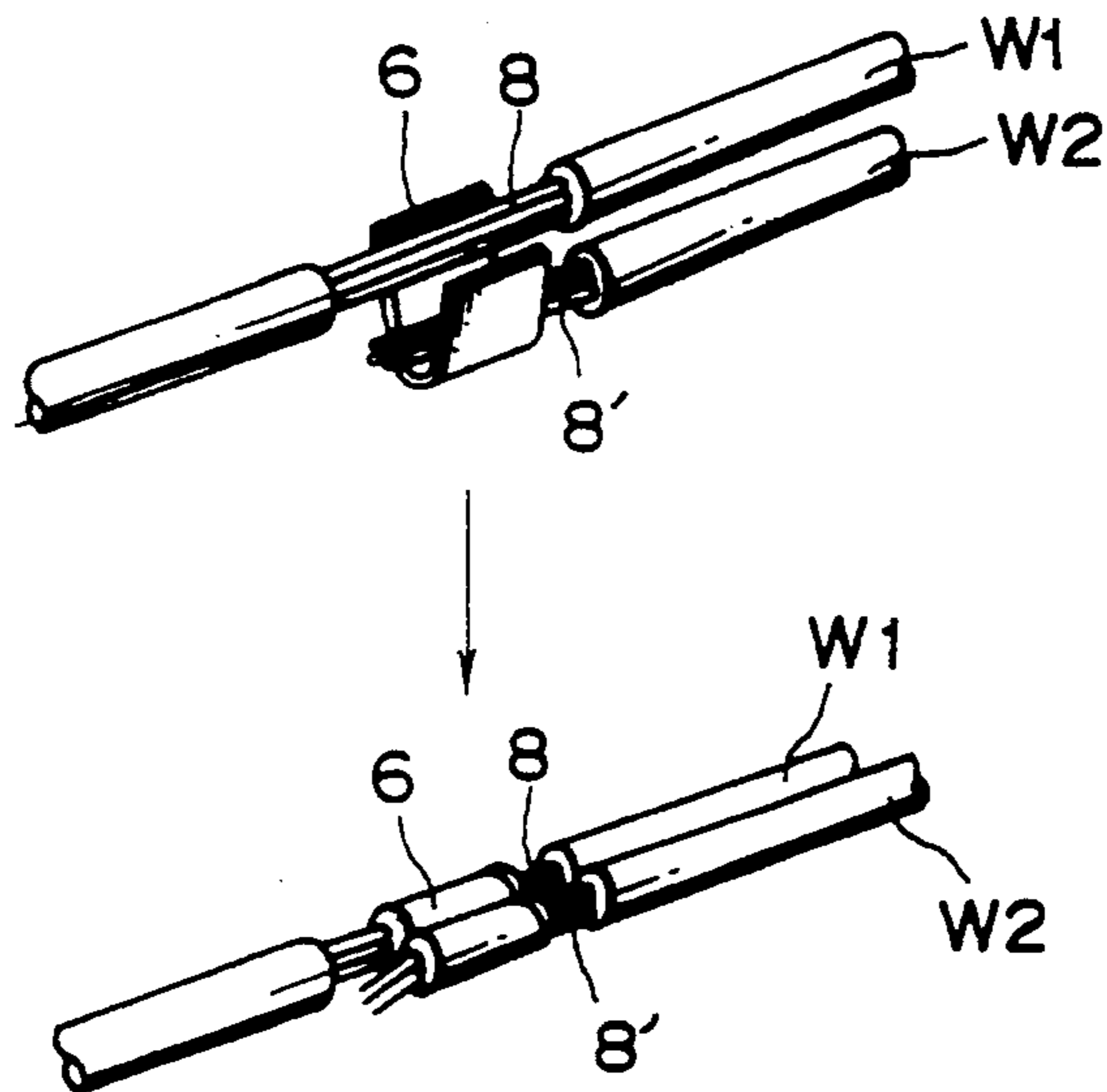
Fig. 14 Prior Art
