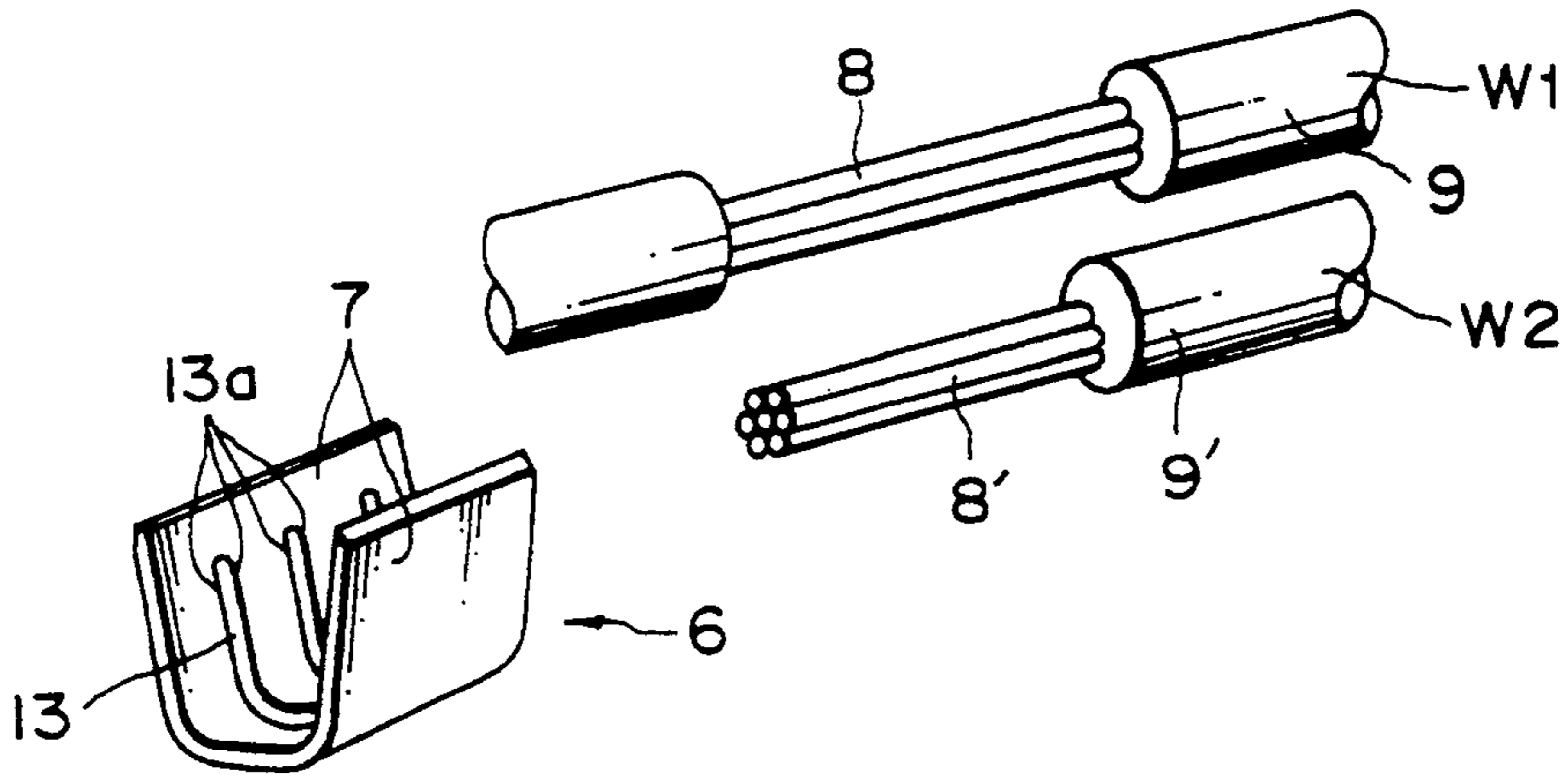
Fig. 13 Prior Art
