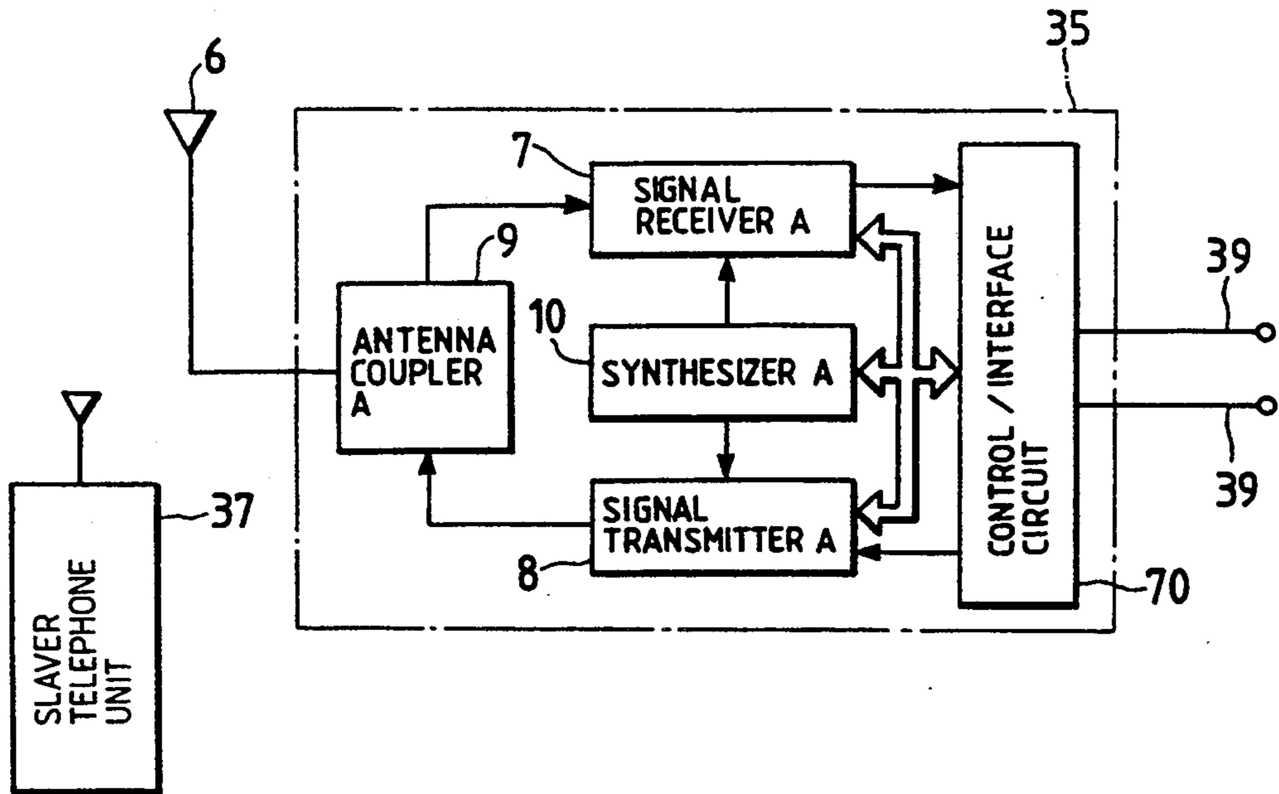
FIG. 12 PRIOR ART
