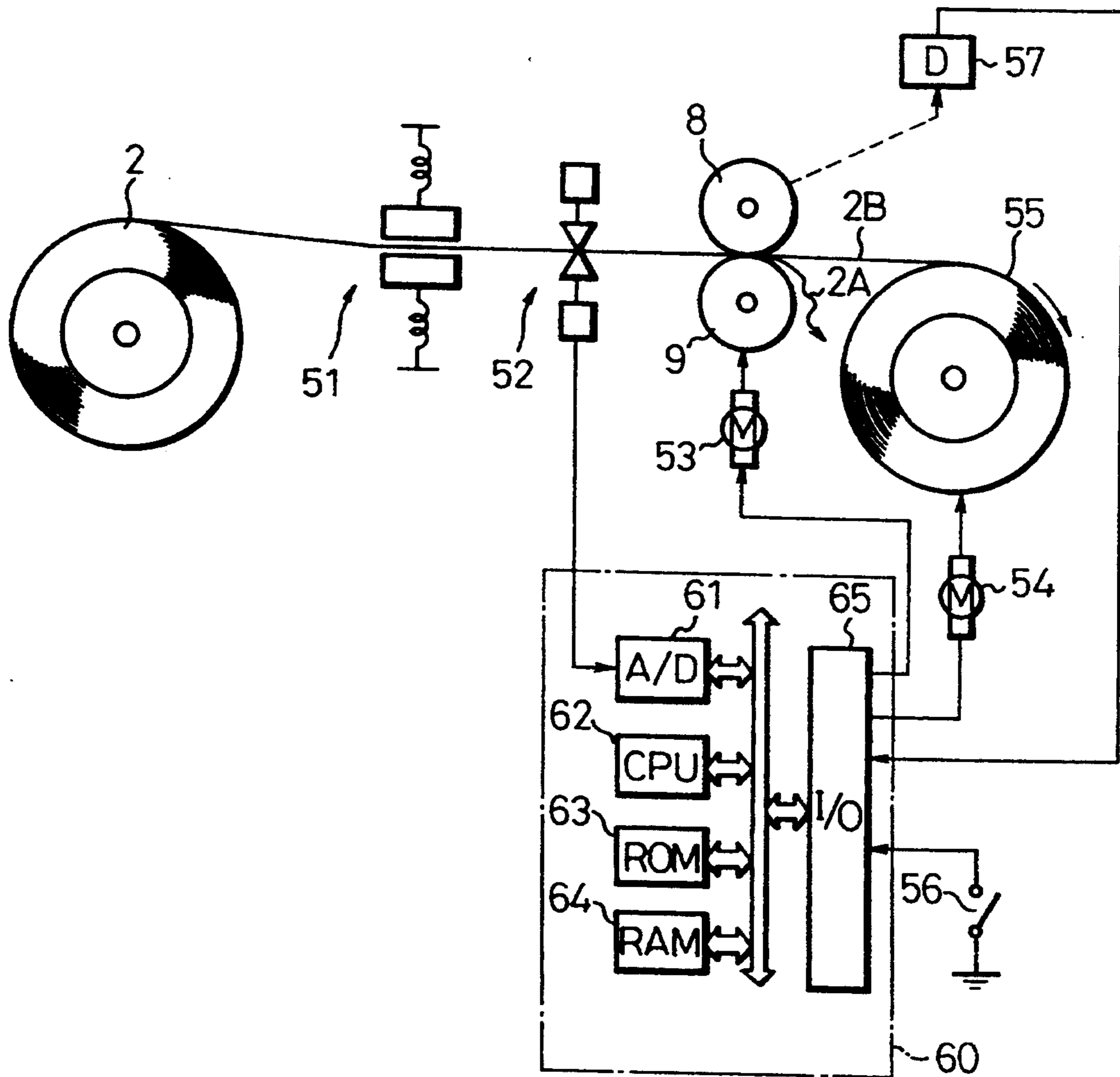
Fig.9 ( PRIOR ART )
