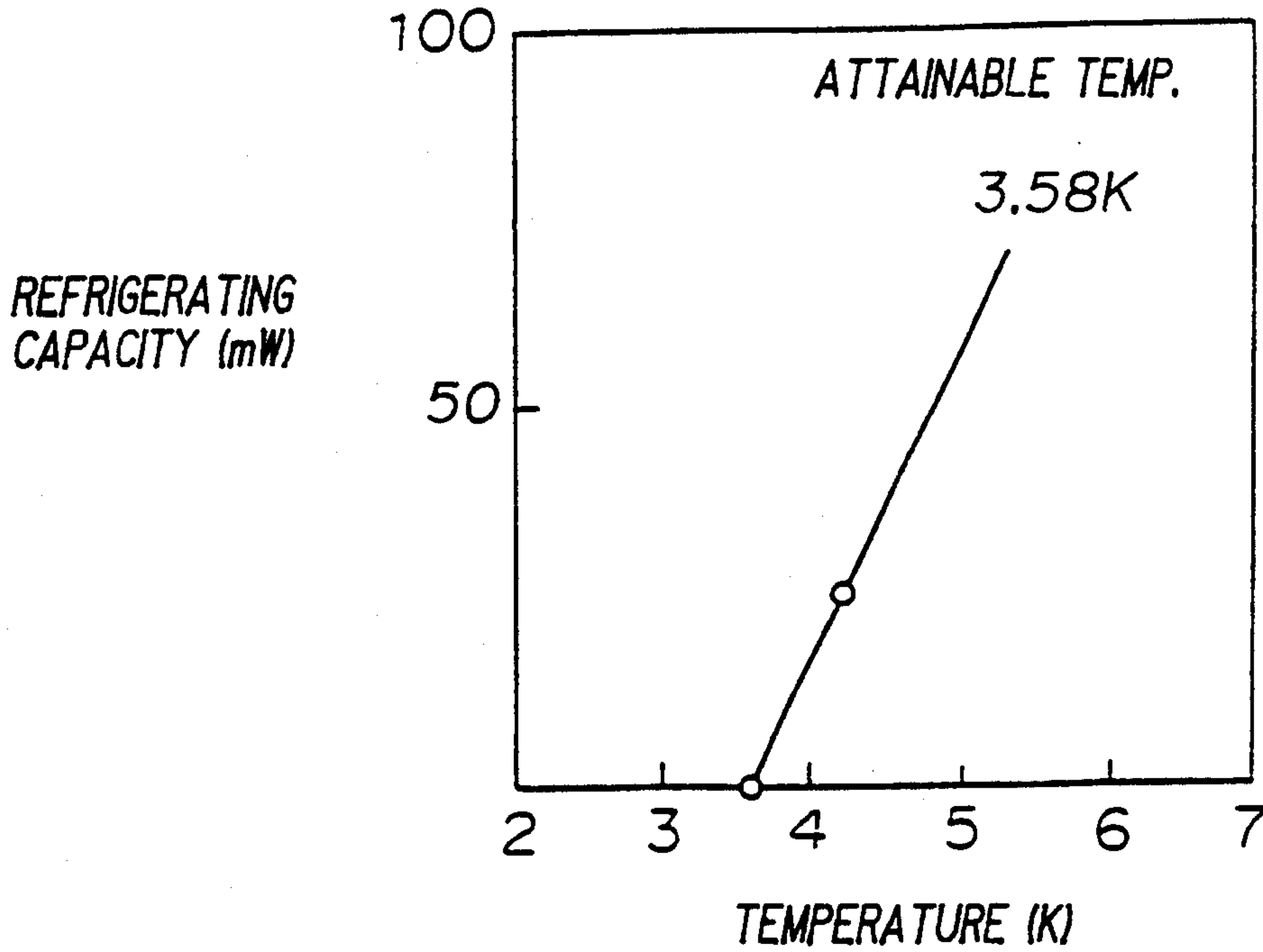
REFRIGERATING CAPACITY OF THREE-STAGE GM REFRIGERATOR
