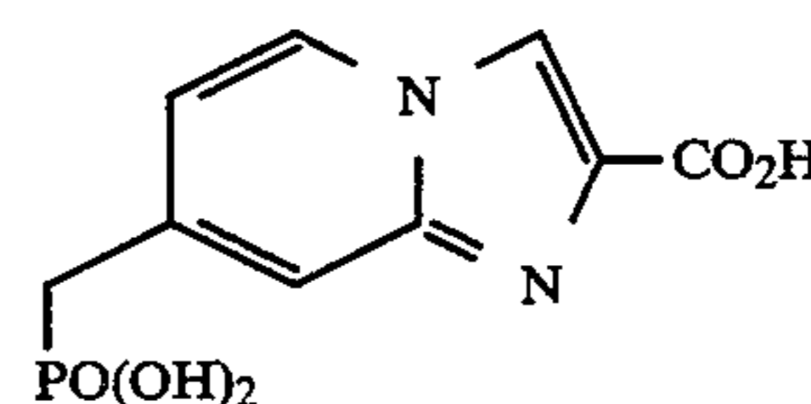
7-(phosphonomethyl)imidazo[1,2-a]pyridine-2-carboxylic acid (HCl)
