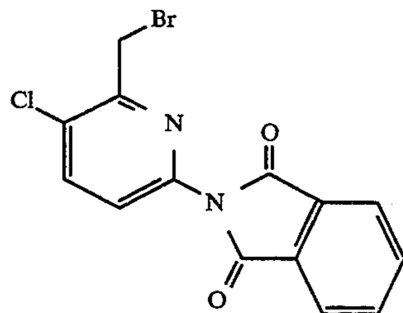
2-[6-(bromomethyl)-5-chloro-2-pyridinyl]-1H-isoindole-1,3(2H)-dione
