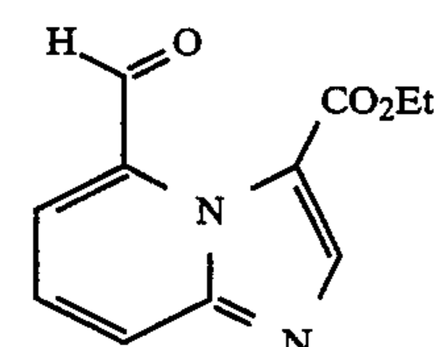
ethyl 5-formylimidazo[1,2-a]pyridine-3-carboxylate
