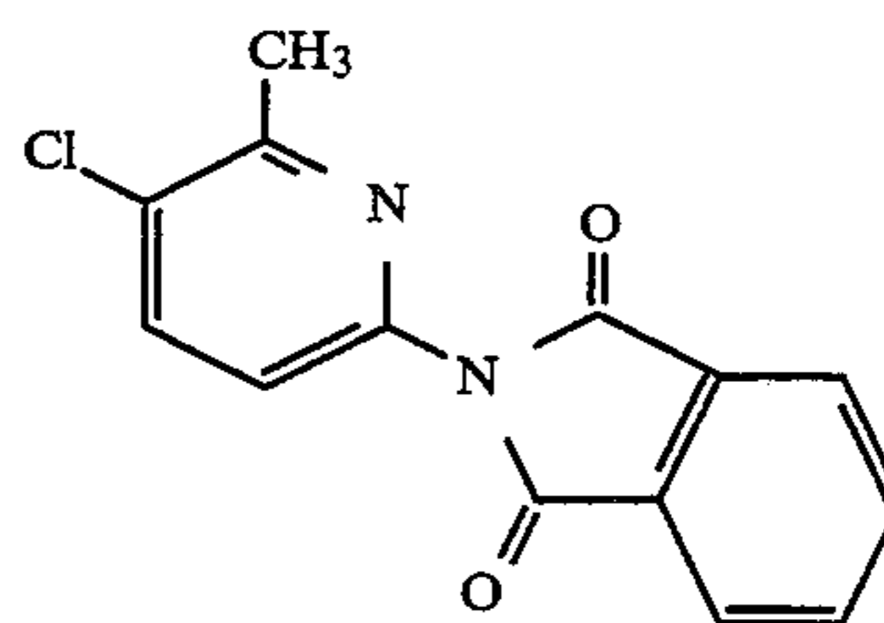
2-(5-chloro-6-methyl-2-pyridinyl)-1H-isindole-1,3(2H)-dione
