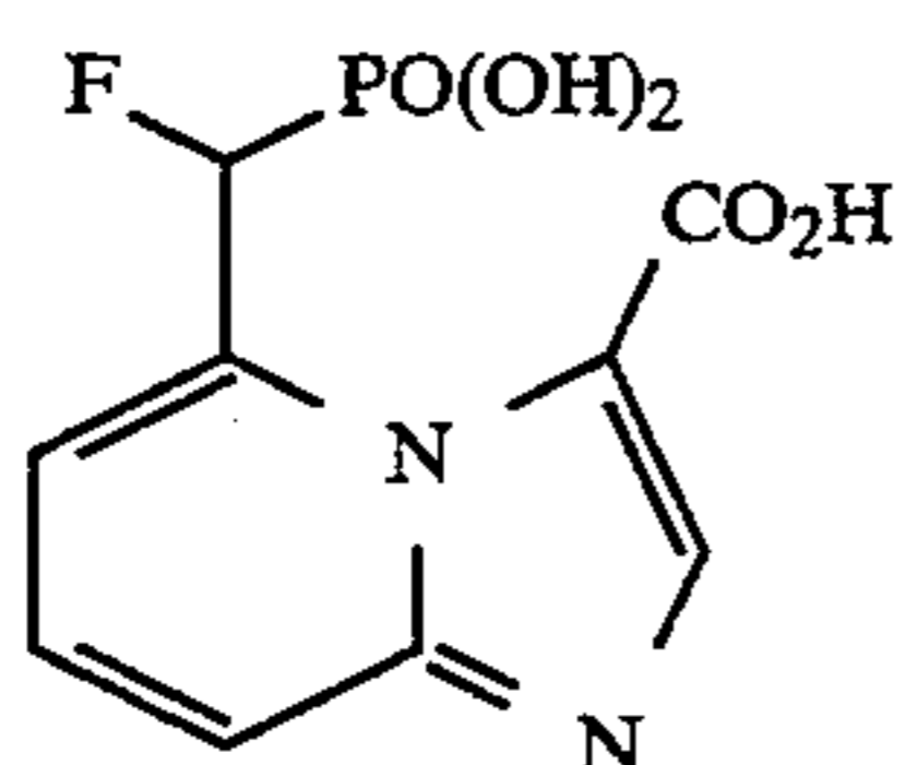
5-(fluorophosphonomethyl)imidazo[1,2-a]pyridine-3-carboxylic acid
