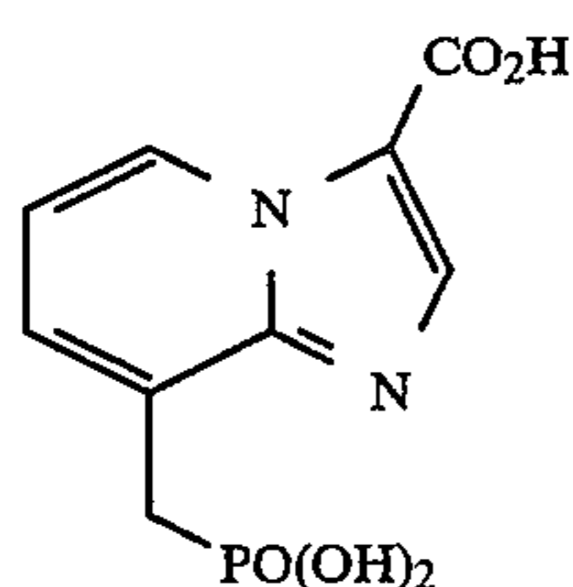
8-(phosphonomethyl)imidazo[1,2-a]pyridine-3-carboxylic acid
