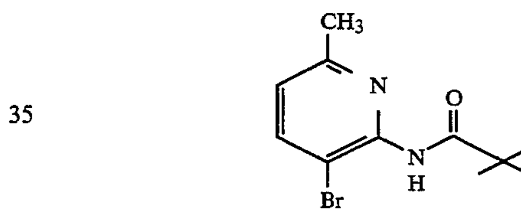
N-(3-bromo-6-methyl-2-pyridinyl)-2,2-dimethylpropanamide
