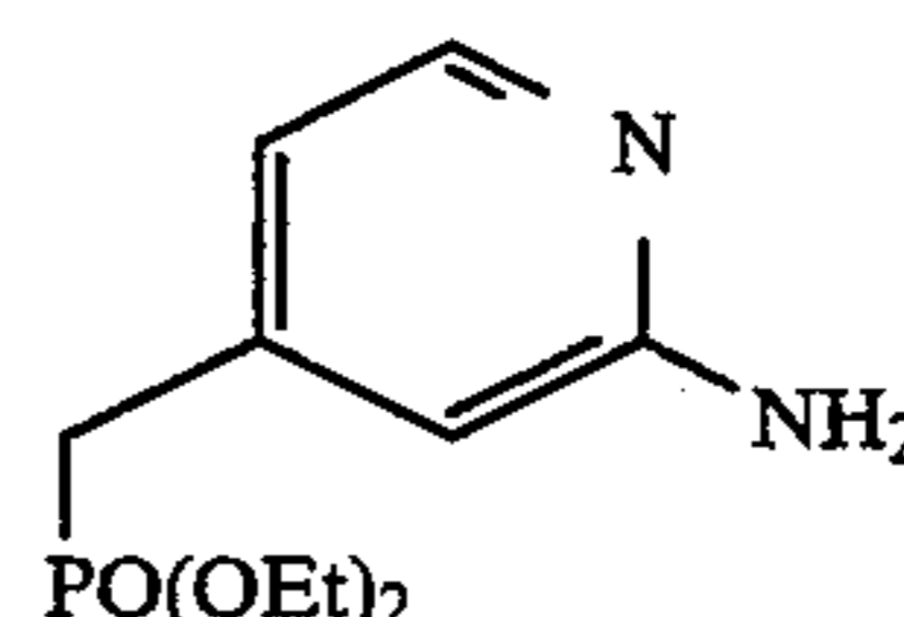
diethyl [(2-amino-4-pyridinyl)methyl]phosphonate
