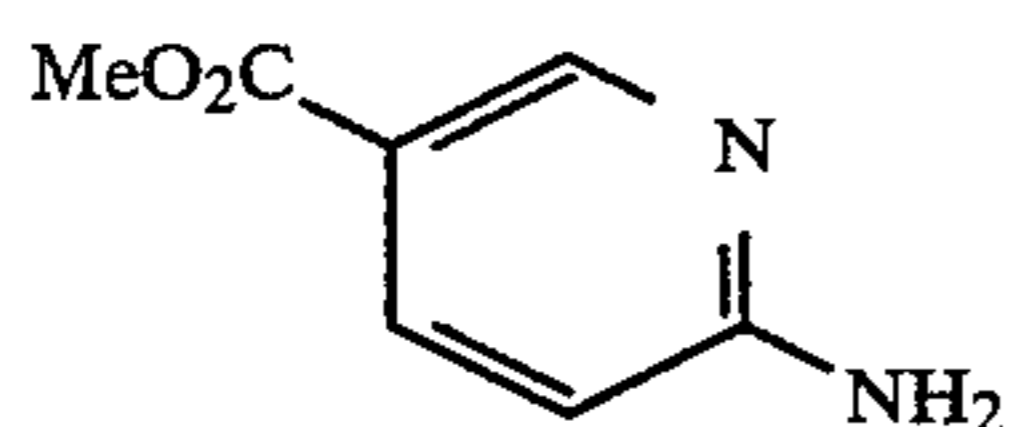
methyl 6-amino-3-pyridinecarboxylate
