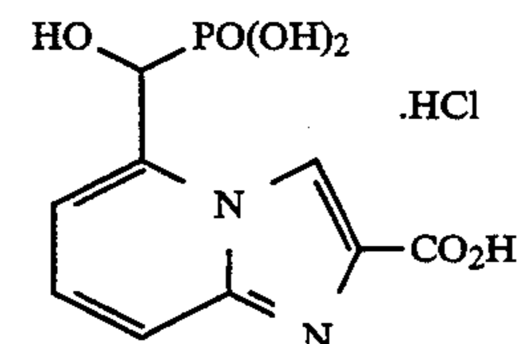
5-(hydroxyphosphonomethyl)imidazo [1,2-a]pyridine-2-carboxylic acid, monohydrochloride
