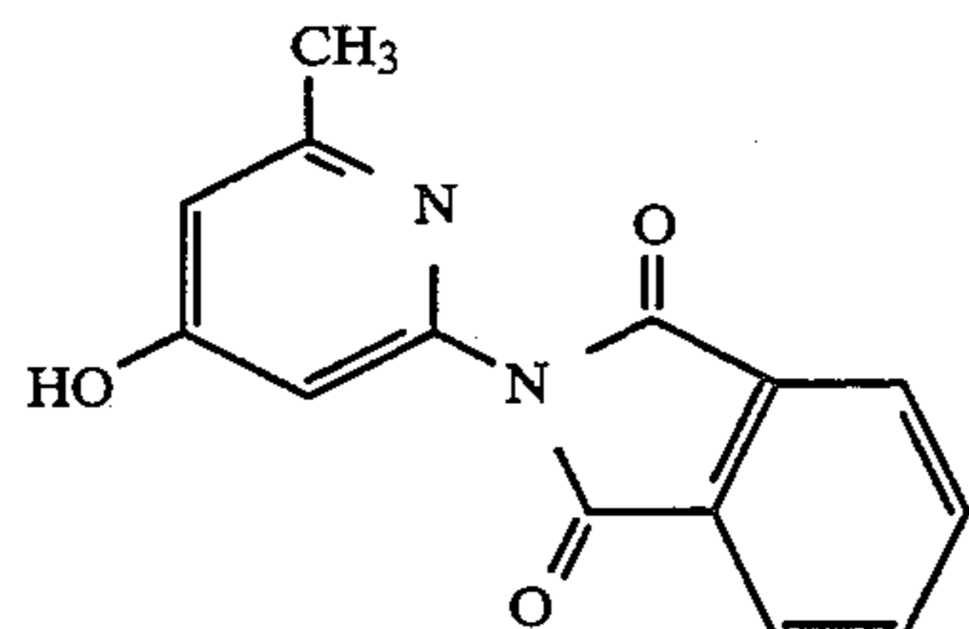
2-(4-hydroxy-6-methyl-2-pyridinyl)-1H-isoindole-1,3(2H)-dione
