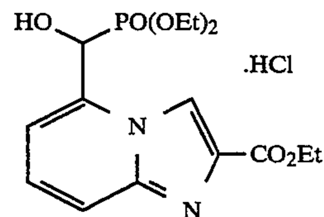
ethyl 5-[(diethoxyphosphinyl)hydroxymethyl]imidazo [1,2-a]pyridine-2-carboxylate, monohydrochloride
