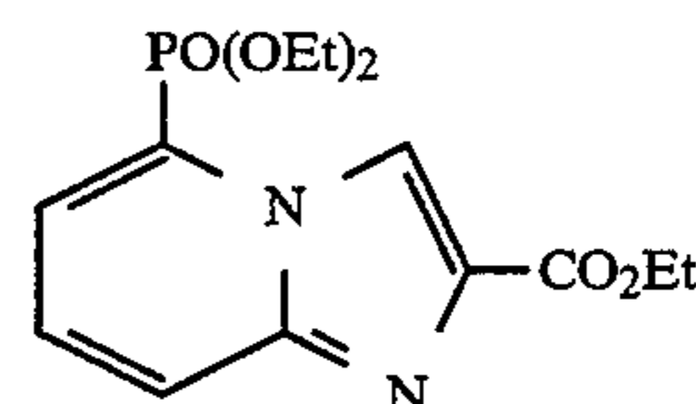
ethyl 5-(diethoxyphosphinyl)imidazo[1,2-a]pyridine-2-carboxylate
