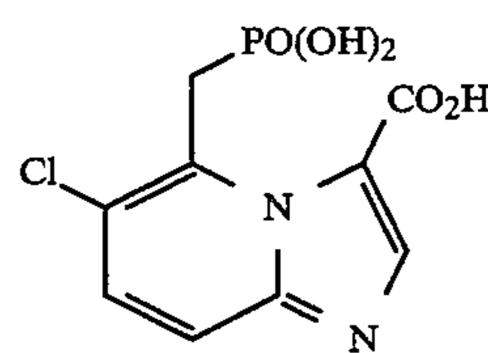
6-chloro-5-(phosphonomethyl)imidazo[1,2-a]pyridine-3-carboxylic acid
