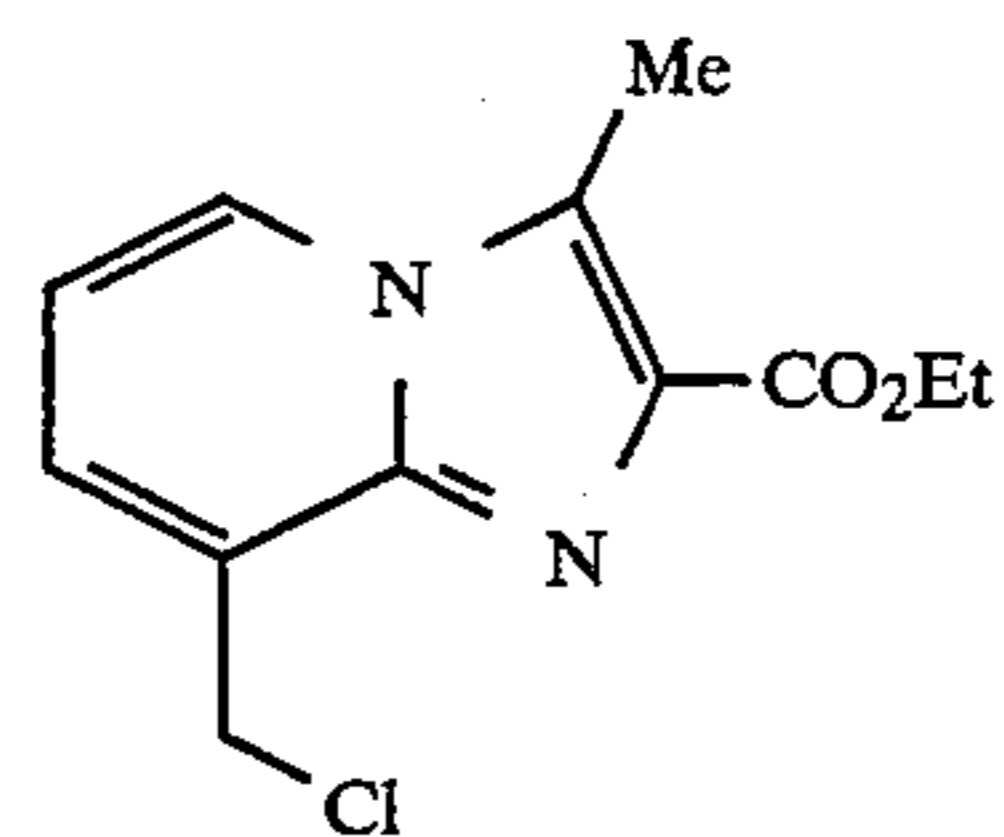
ethyl 8-(chloromethyl)-3-methylimidazo[1,2-a]pyridine-2-carboxylate
