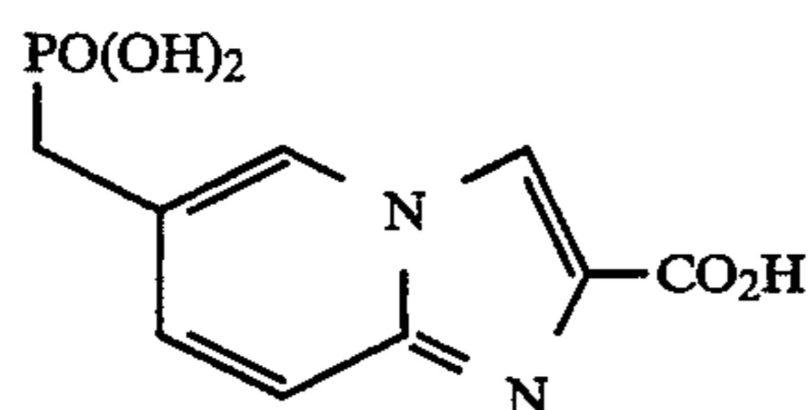
6-(phosphonomethyl)imidazo[1,2-a]pyridine-2-carboxylic acid (HCl)
