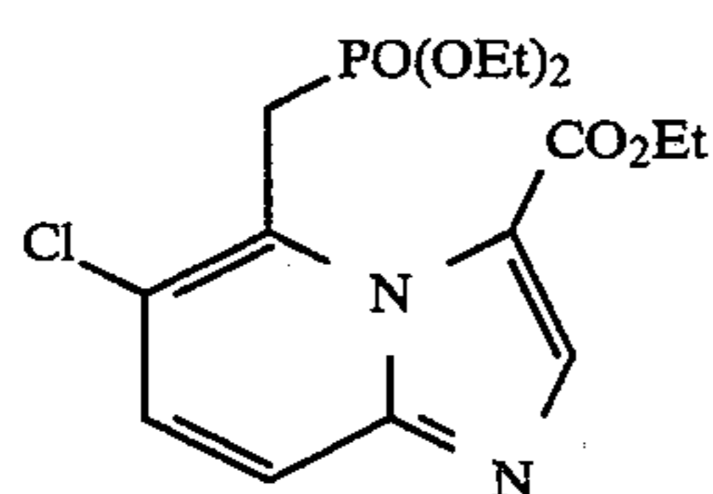
ethyl 6-chloro-5-[(diethoxyphosphinyl)methyl]imidazo[1,2-a]pyridine-3-carboxylate
