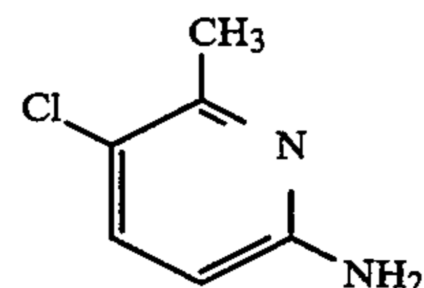
5-chloro-6-methyl-2-pyridinamine
