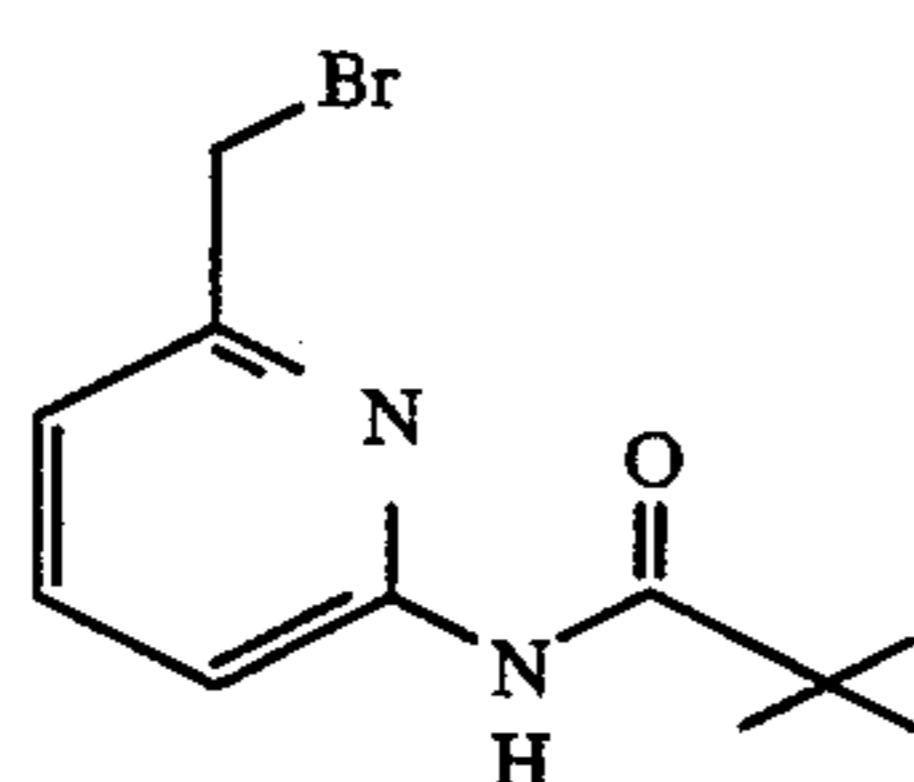
N-[6-(bromomethyl)-2-pyridinyl]-2,2-dimethylpropanamide
