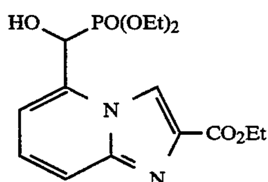
ethyl 5-[(diethoxyphosphinyl)hydroxymethyl]imidazo [1,2-a]pyridine-2-carboxylate
