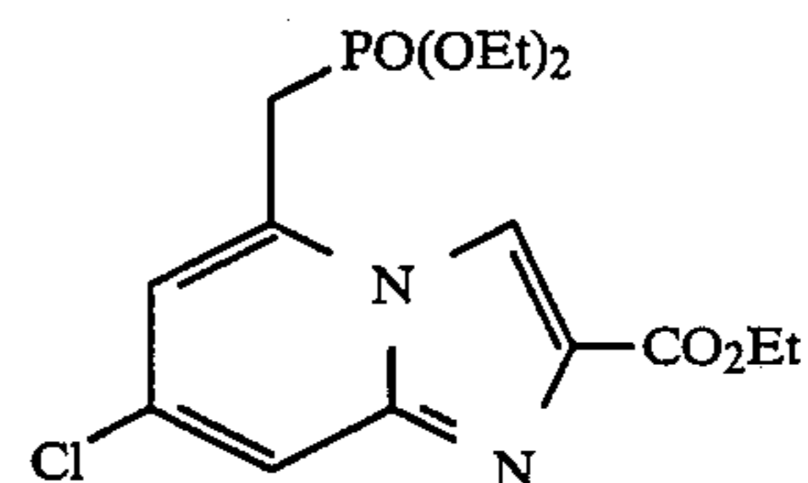
ethyl 7-chloro-5-[(diethoxyphosphinyl)methyl]imidazo[1,2-a]pyridine-2-carboxylate
