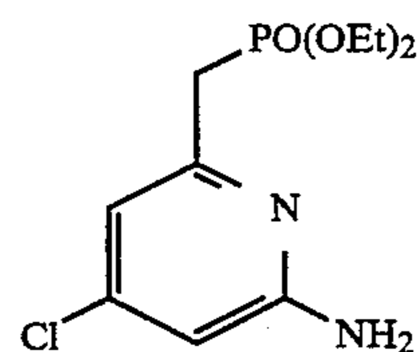
diethyl [(6-amino-4-chloro-2-pyridinyl)methyl]phosphonate
