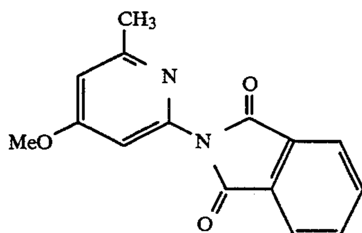
2-(4-methoxy-6-methyl-2-pyridinyl)-1H-isoindole-1,3(2H)-dione
