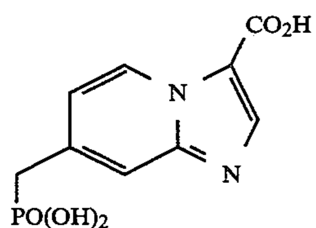
7-(phosphonomethyl)imidazo[1,2-a]pyridine-3-carboxylic acid
