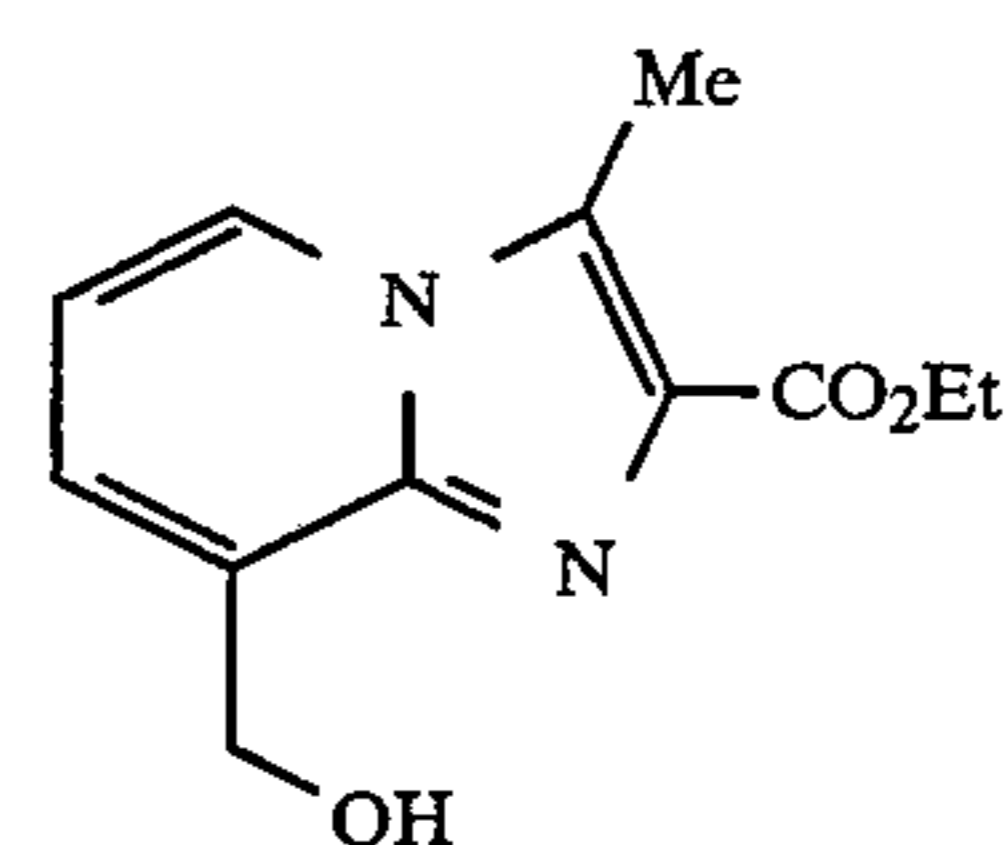
ethyl 8-(hydroxymethyl)-3-methylimidazo[1,2-a]pyridine-2-carboxylate
