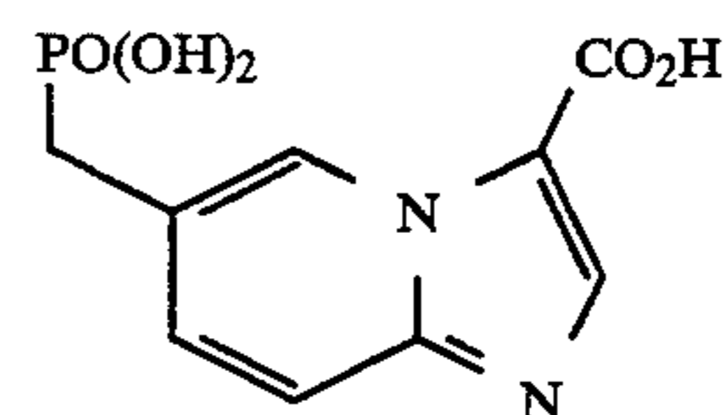
6-(phosphonomethyl)imidazo[1,2-a]pyridine-3-carboxylic acid
