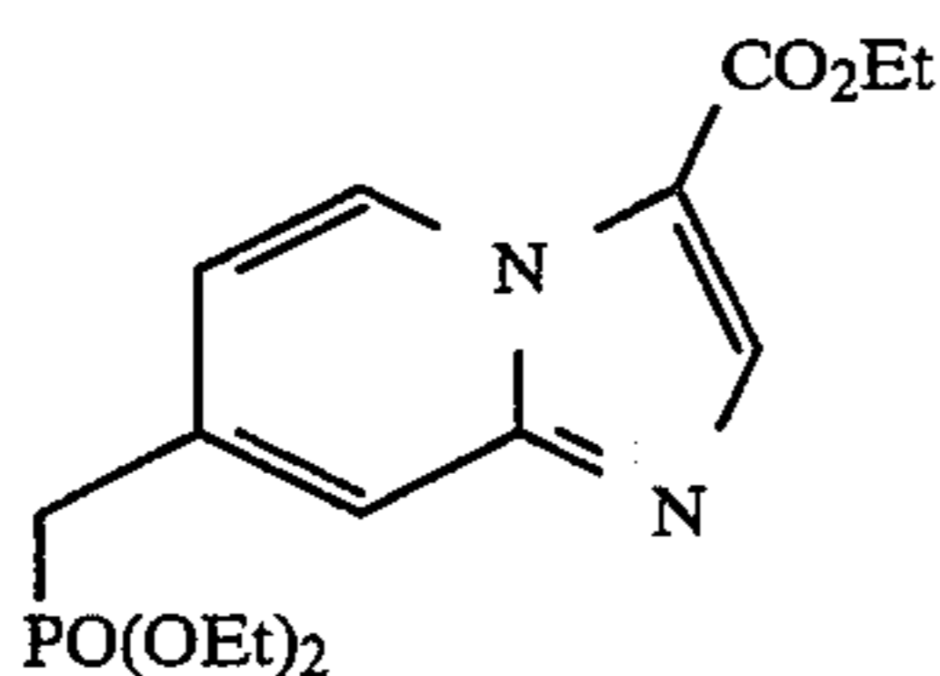
ethyl 7-[(diethoxyphosphinyl)methyl]imidazo[1,2-a]pyridine-3-carboxylate
