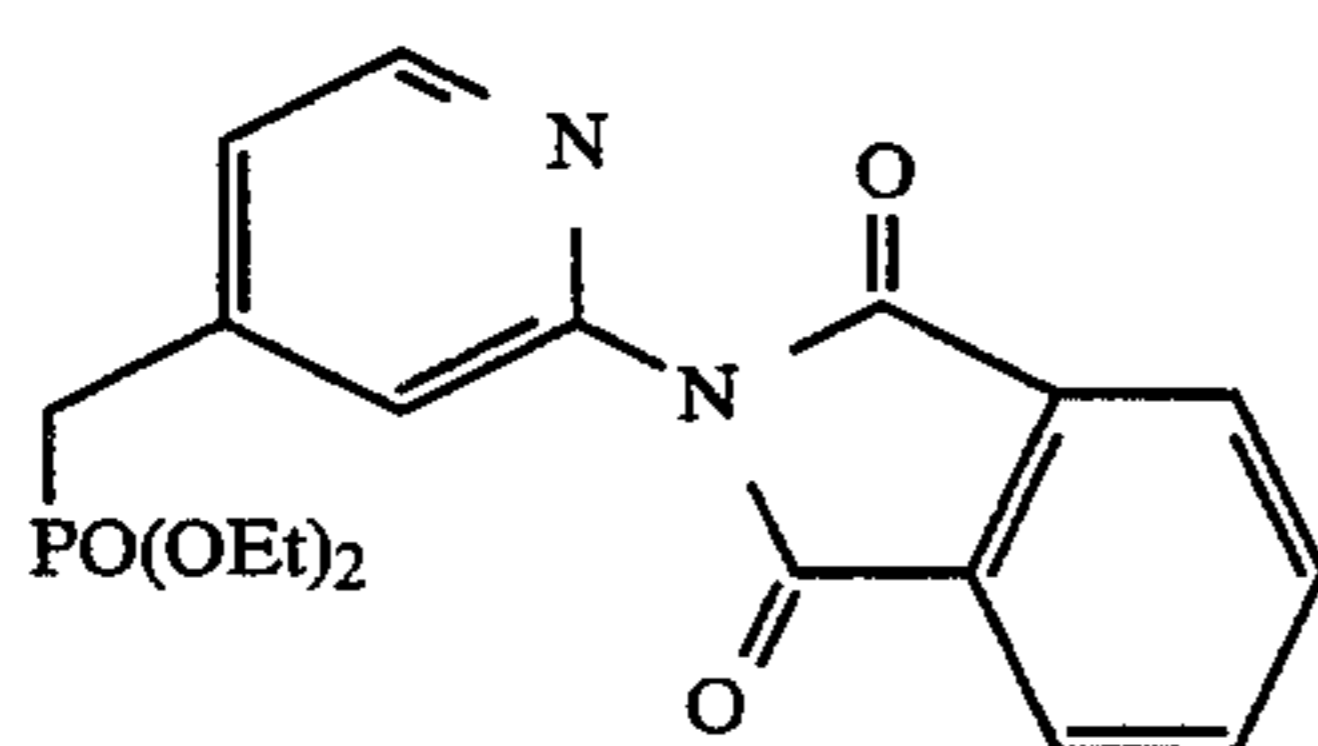
diethyl [[2-(1,3-dihydro-1,3-dioxo-2H-isoindol-2-yl)-4-pyridinyl]methyl]phosphonate
