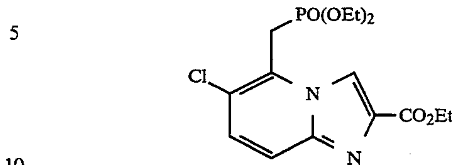
ethyl 6-chloro-5-[(diethoxyphosphinyl)methyl]imidazo[1,2-a]pyridine-2-carboxylate
