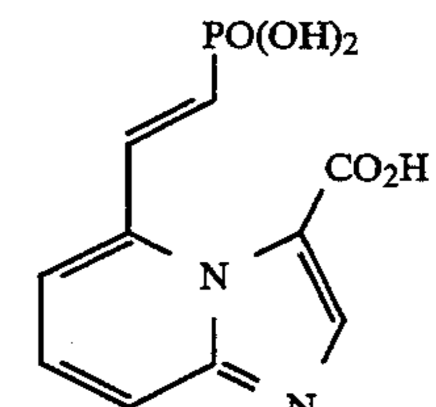
5-(2-phosphono-E-ethenyl)imidazo[1,2-a]pyridine-3-carboxylic acid
