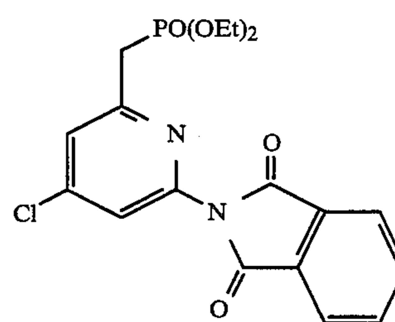
diethyl [[4-chloro-6-(1,3-dihydro-1,3-dioxo-2H-isoindol-2-yl)-2-pyridinyl]methyl]phosphonate
