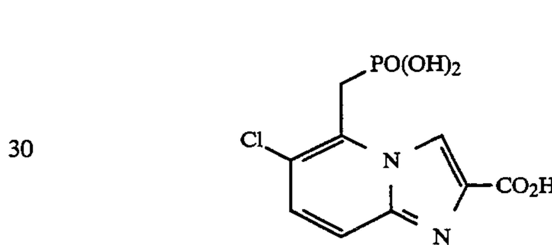
6-chloro-5-(phosphonomethyl)imidazo[1,2-a]pyridine-2-carboxylic acid
