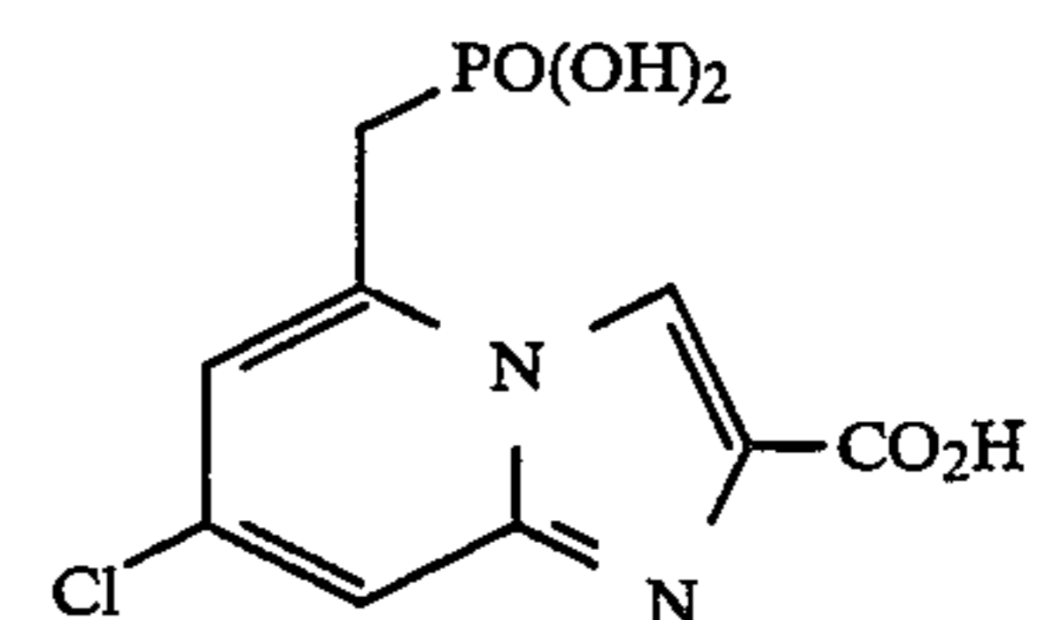
7-chloro-5-(phosphonomethyl)imidazo[1,2-a]pyridine-2-carboxylic acid
