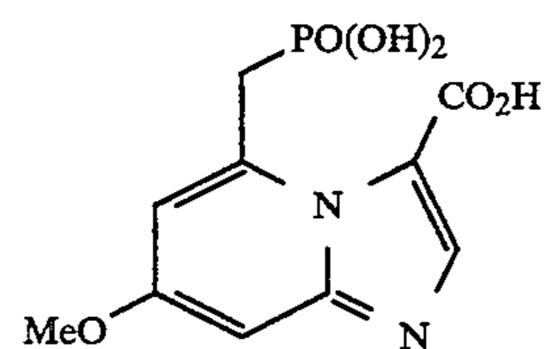
7-methoxy-5-(phosphonomethyl)imidazo[1,2-a]pyridine-3-carboxylic acid
