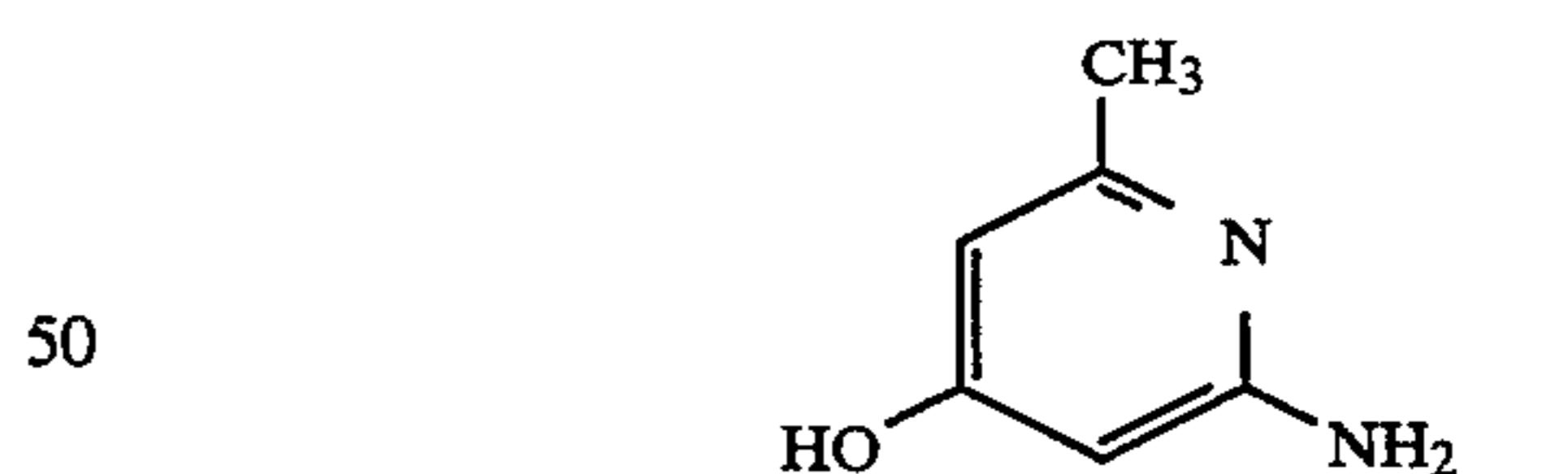
4-hydroxy-6-methyl-2-pyridinamine
