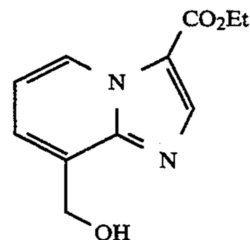
ethyl 8-(hydroxymethyl)imidazo[1,2-a]pyridine-3-carboxylate
