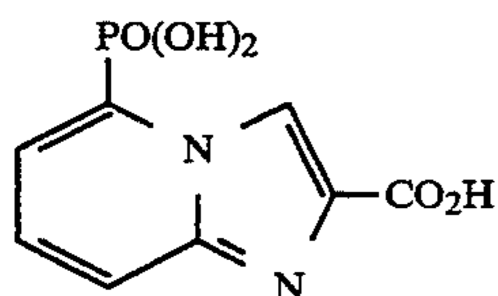
5-phosphonoimidazo [1,2-a]pyridine-2-carboxylic acid
