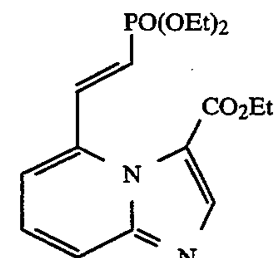
ethyl 5-[2-(diethoxyphosphinyl)-E-ethenyl]imidazo[1,2-a]pyridine-3-carboxylate
