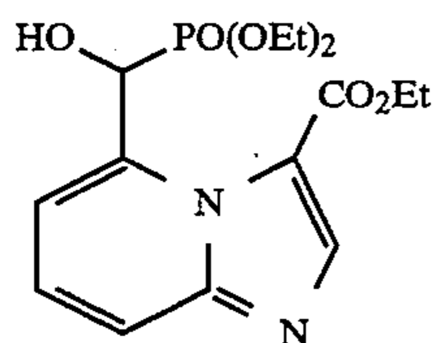
ethyl 5-[(diethoxyphosphinyl)hydroxymethyl]imidazo[1,2-a]pyridine-3-carboxylate
