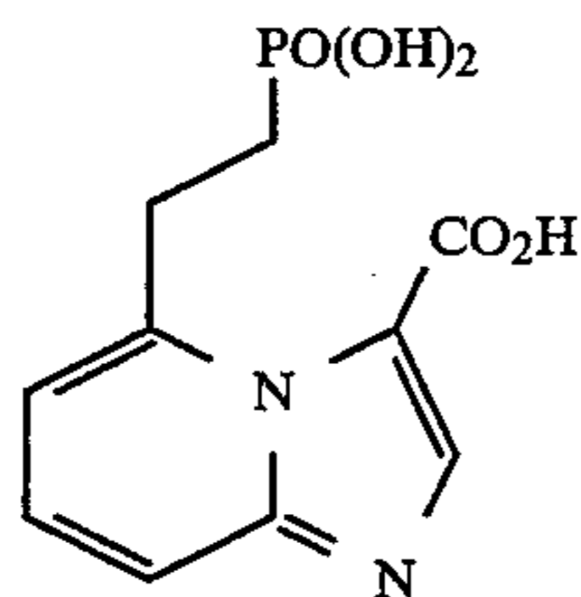
5-(2-phosphonoethyl)imidazo[1,2-a]pyridine-3-carboxylic acid
