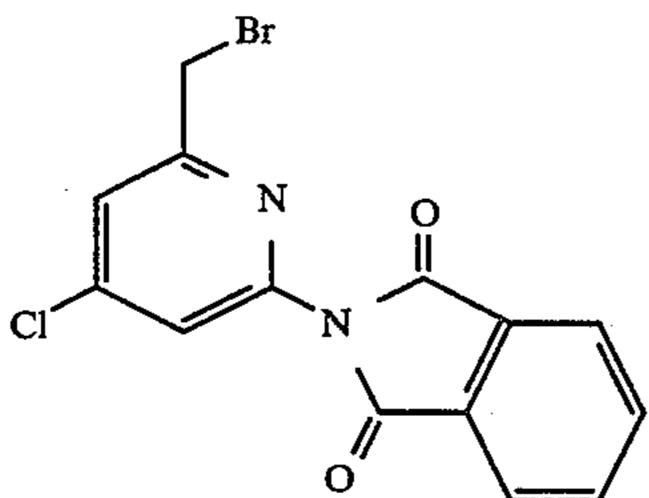
2-[6-(bromomethyl)-4-chloro-2-pyridinyl]-1H-isoindole-1,3(2H)-dione
