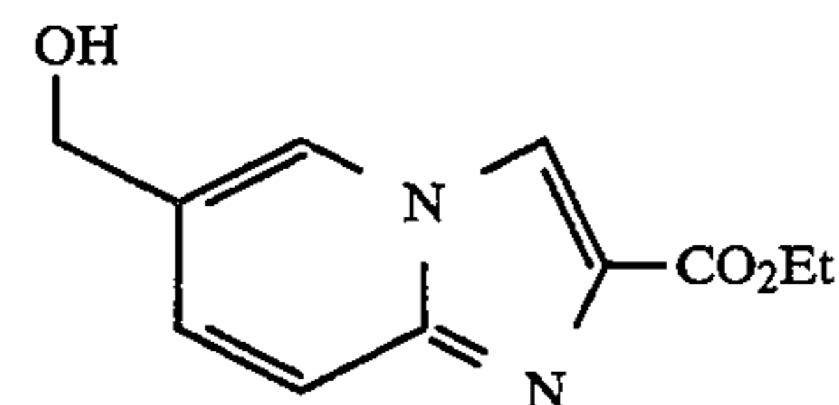
ethyl 6-(hydroxymethyl)imidazo[1,2-a]pyridine-2-carboxylate
