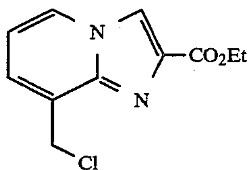
ethyl 8-(chloromethyl)imidazo[1,2-a]pyridine-2-carboxylate
