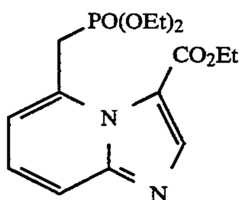
ethyl 5-[(diethoxyphosphinyl)methyl]imidazo[1,2-a]pyridine-3-carboxylate
