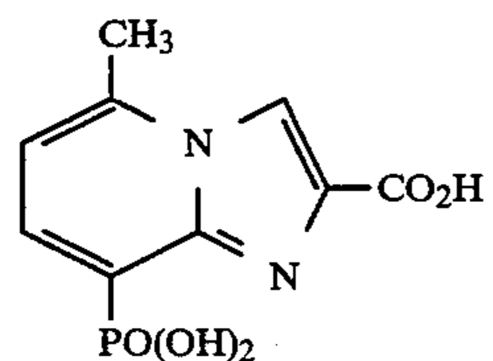
5-methyl-8-phosphonoimidazo[1,2-a]pyridine-2-carboxylic acid
