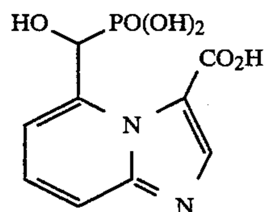
5-[hydroxyphosphonomethyl]imidazo[1,2-a]pyridine-3-carboxylic acid
