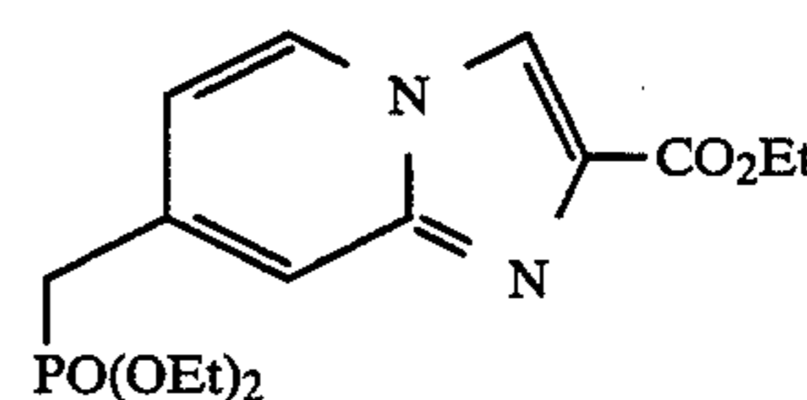
ethyl 7-[(diethoxyphosphinyl)methyl]imidazo[1,2-a]pyridine-2-carboxylate
