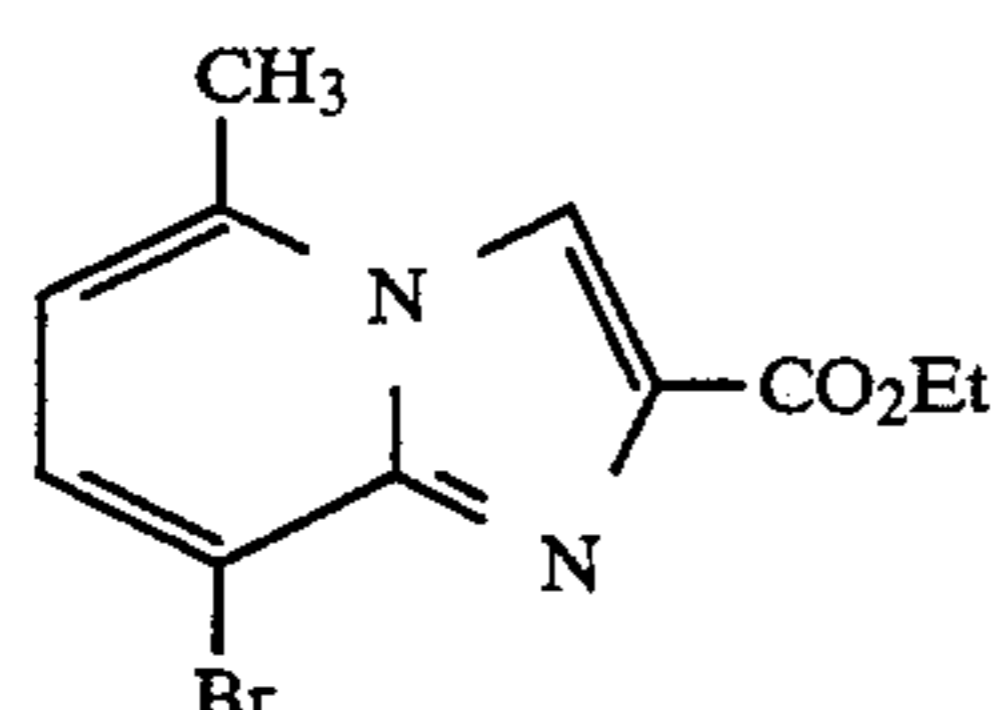
ethyl 8-bromo-5-methylimidazo[1,2-a]pyridine-2-carboxylate
