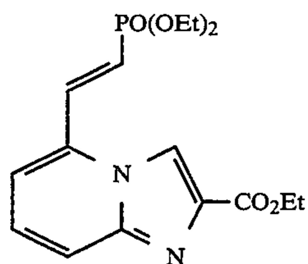
ethyl 5-[2-(diethoxyphosphinyl)-E-ethenyl]imidazo[1,2-a]pyridine-2-carboxylate
