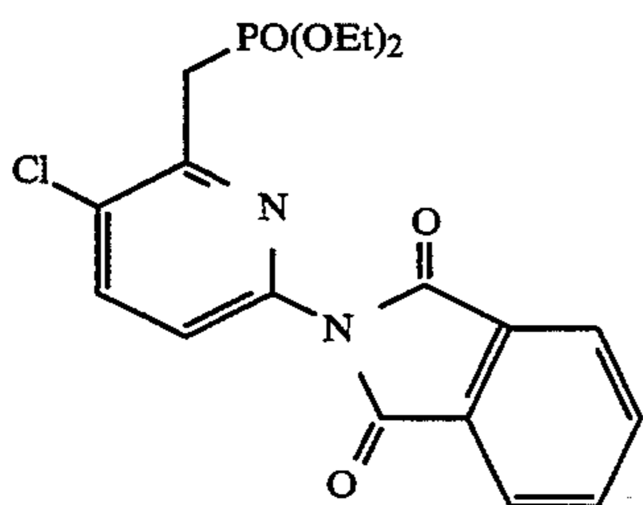
diethyl [[3-chloro-6-(1,3-dihydro-1,3-dioxo-2H-isoindol-2-yl)-2-pyridinyl]methyl]phosphonate
