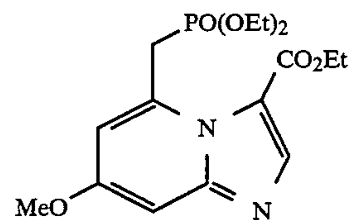
ethyl 5-[(diethoxyphosphinyl)methyl]-7-methoxyimidazo[1,2-a]pyridine-3-carboxylate
