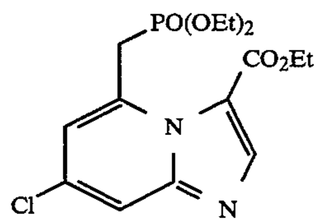
ethyl 7-chloro-5-[(diethoxyphosphinyl)methyl]imidazo[1,2-a]pyridine-3-carboxylate
