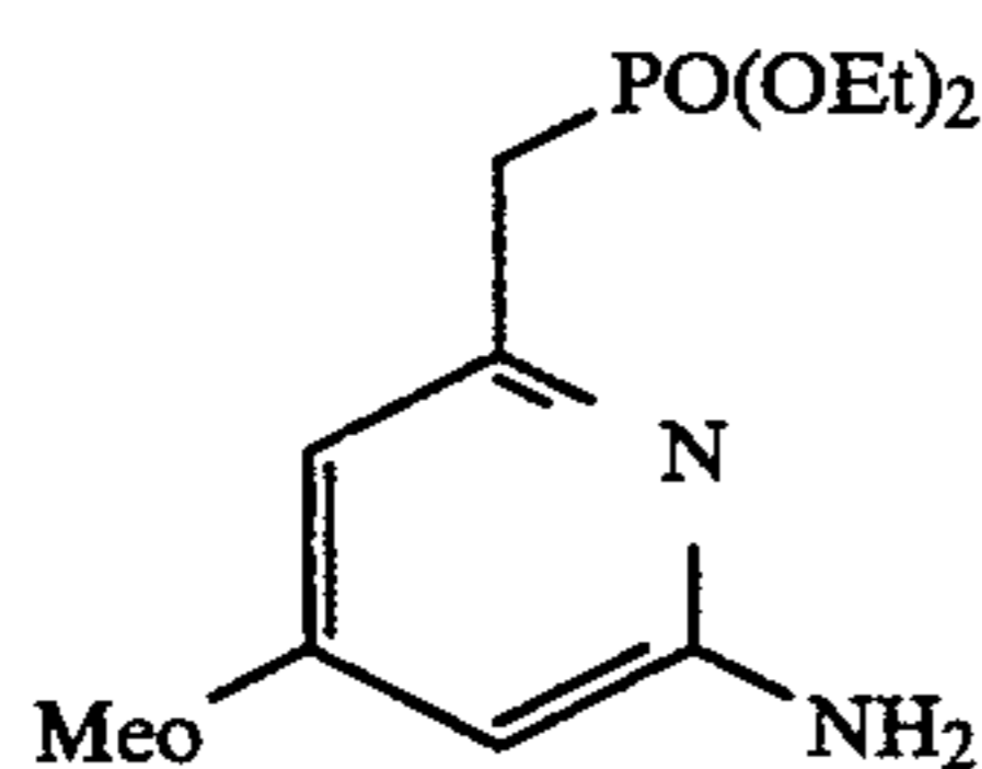
diethyl [(6-amino-4-methoxy-2-pyridinyl)methyl]phosphonate
