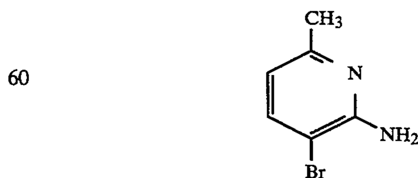
3-bromo-6-methyl-2-pyridinamine
