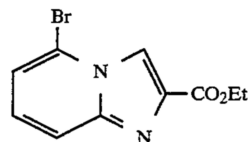
ethyl 5-bromoimidazo[1,2-a]pyridine-2-carboxylate
