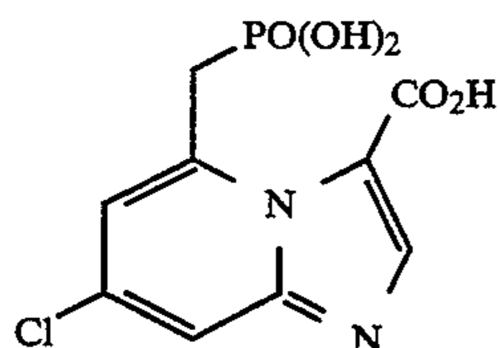
7-chloro-5-(phosphonomethyl)imidazo[1,2-a]pyridine-3-carboxylic acid
