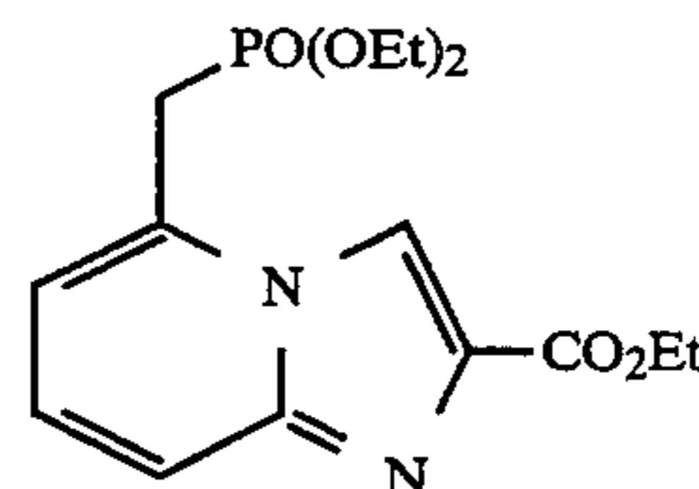
ethyl 5-[(diethoxyphosphinyl)methyl]imidazo[1,2-a]pyridine-2-carboxylate
