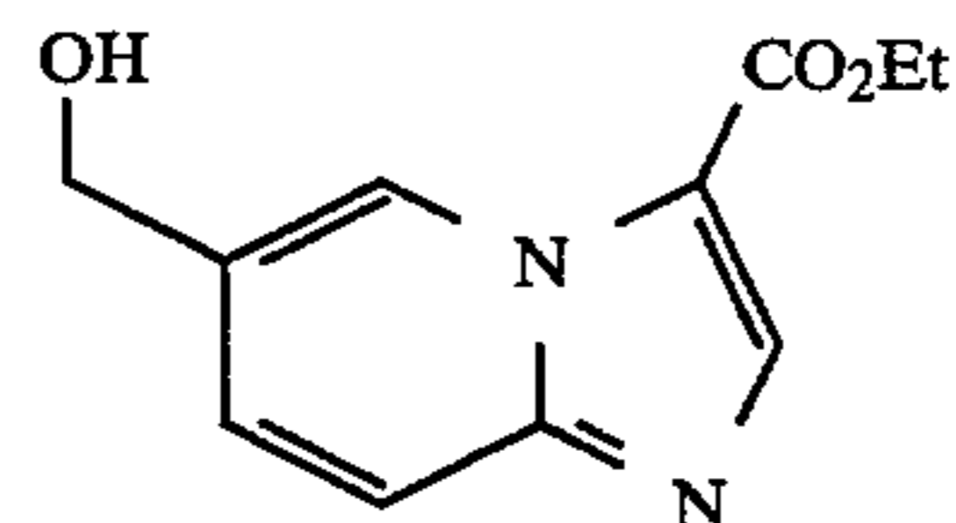
ethyl 6-(hydroxymethyl)imidazo[1,2-a]pyridine-3-carboxylate
