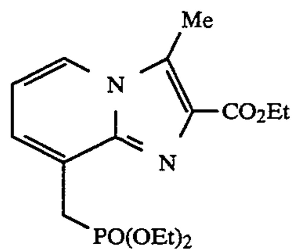
ethyl 8-[(diethoxyphosphinyl)methyl]-3-methylimidazo[1,2-a]pyridine-2-carboxylate
