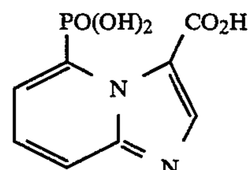
5-phosphonoimidazo[1,2-a]pyridine-3-carboxylic acid
