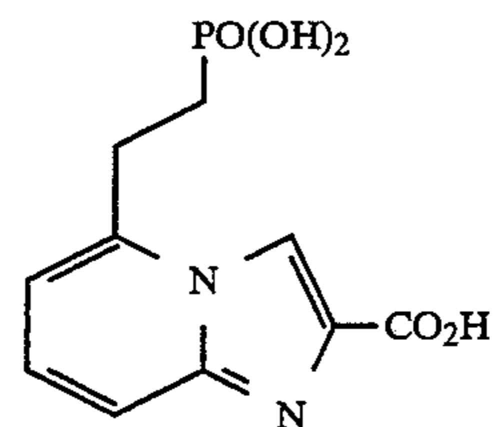
5-(2-phosphonoethyl)imidazo[1,2-a]pyridine-2-carboxylic acid
