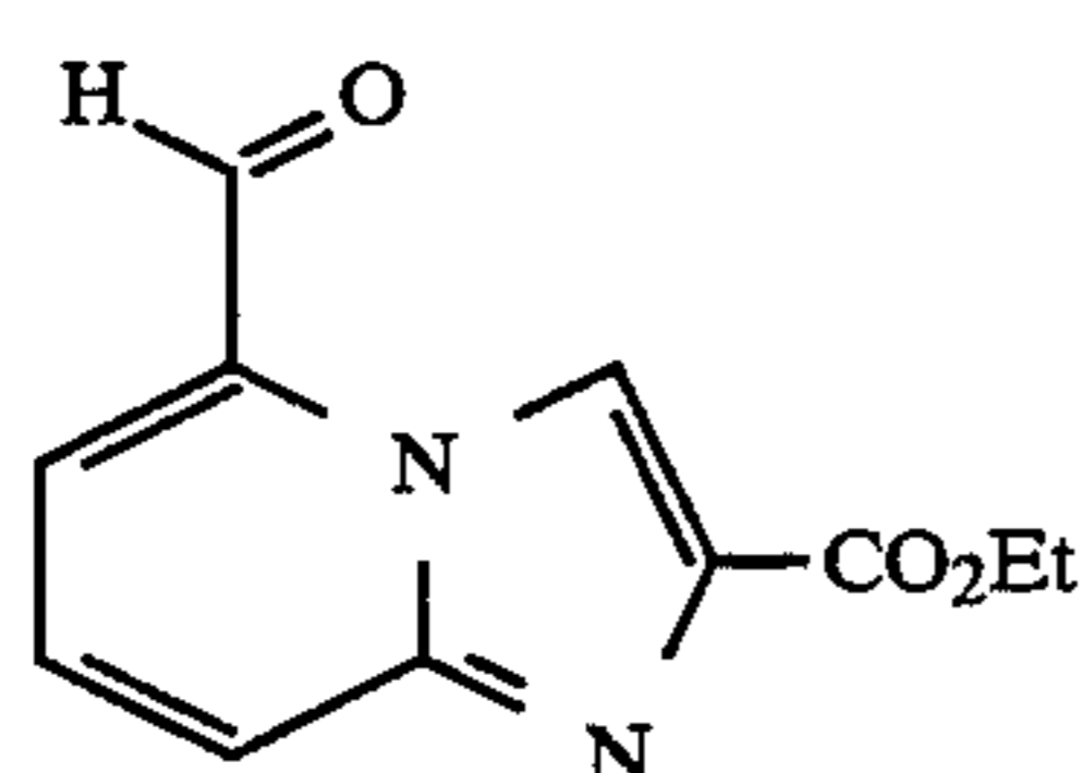
ethyl 5-formylimidazo [1,2-a]pyridine-2-carboxylate
