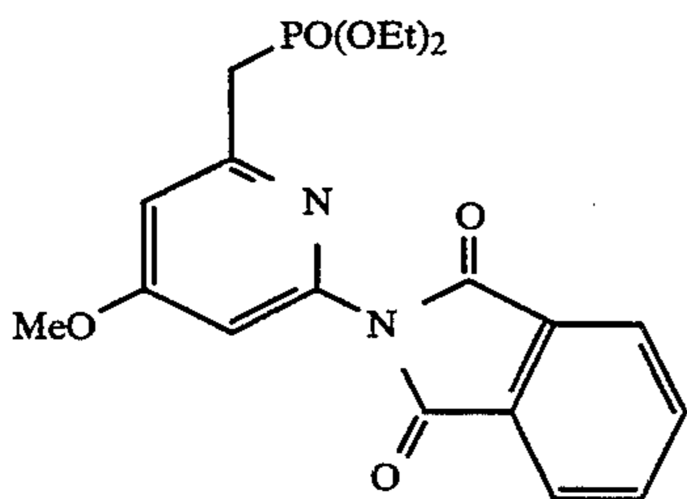
diethyl [[6-(1,3-dihydro-1,3-dioxo-2H-isoindol-2-yl)-4-methoxy-2-pyridinyl]methyl]phosphonate
