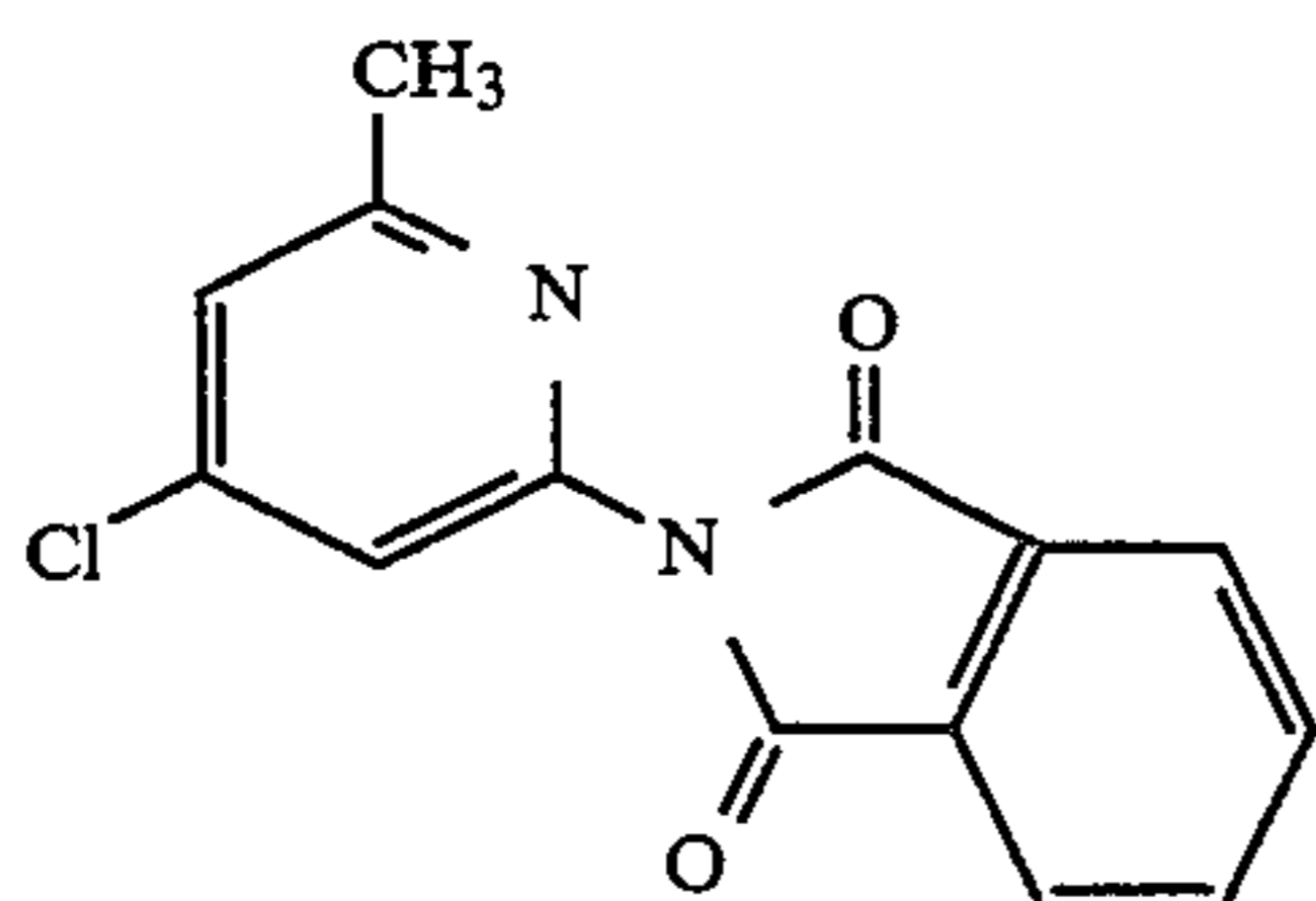
2-(4-chloro-6-methyl-2-pyridinyl)-1H-isoindole-1,3(2H)-dione
