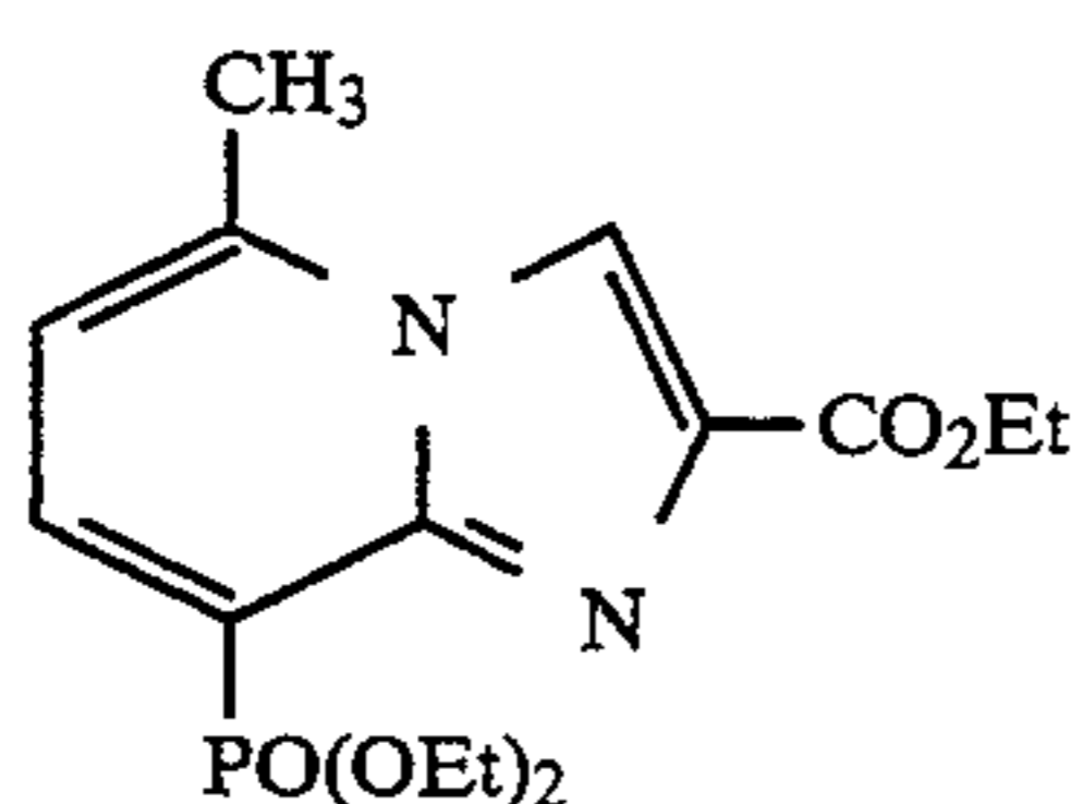
ethyl 8-(diethoxyphosphinyl)-5-methylimidazo[1,2-a]pyridine-2-carboxylate
