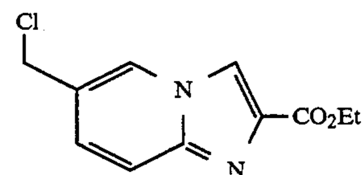
ethyl 6-(chloromethyl)imidazo[1,2-a]pyridine-2-carboxylate
