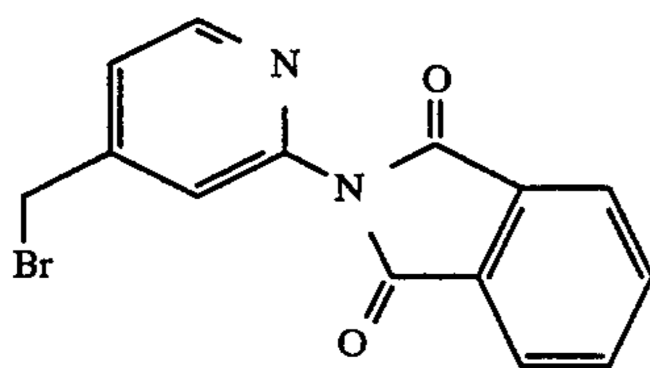
2-[4-(bromomethyl)-2-pyridinyl]-1H-isoindole-1,3(2H)-dione
