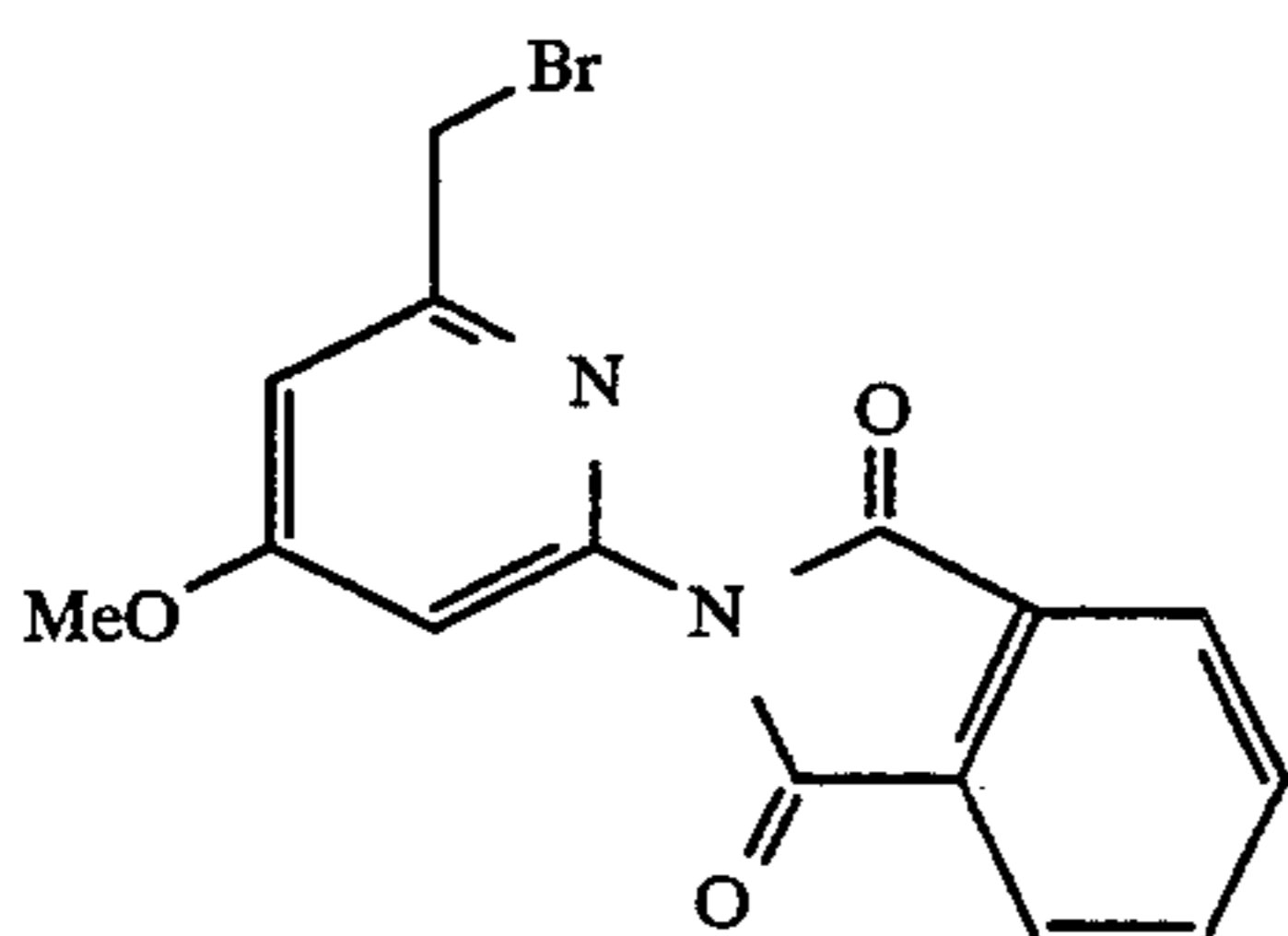
2-[6-(bromomethyl)-4-methoxy-2-pyridinyl]-1H-isoindole-1,3(2H)-dione
