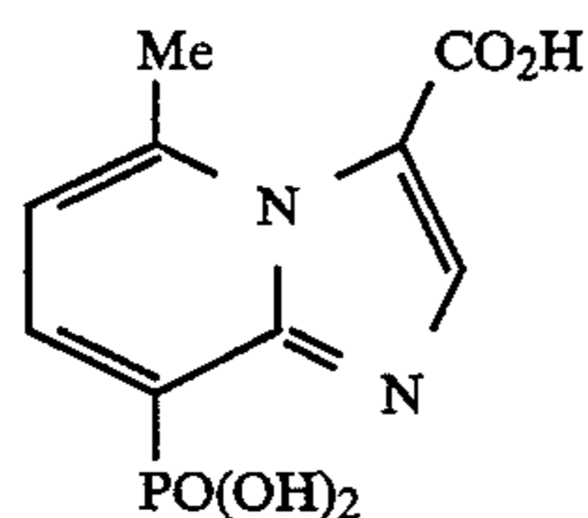
5-methyl-8-phosphonoimidazo[1,2-a]pyridine-3-carboxylic acid
