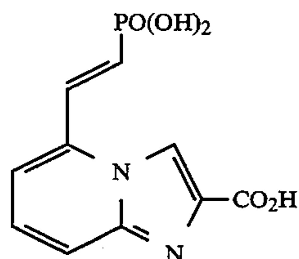
5-(2-phosphono-E-ethenyl)imidazo[1,2-a]pyridine-2-carboxylic acid
