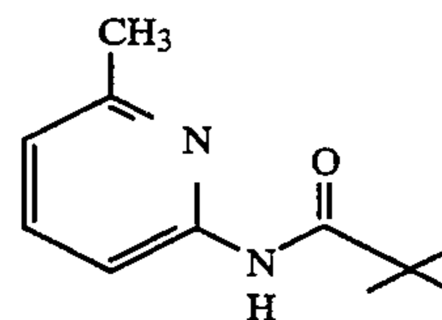
2,2-dimethyl-N-(6-methyl-2-pyridinyl)propanamide
