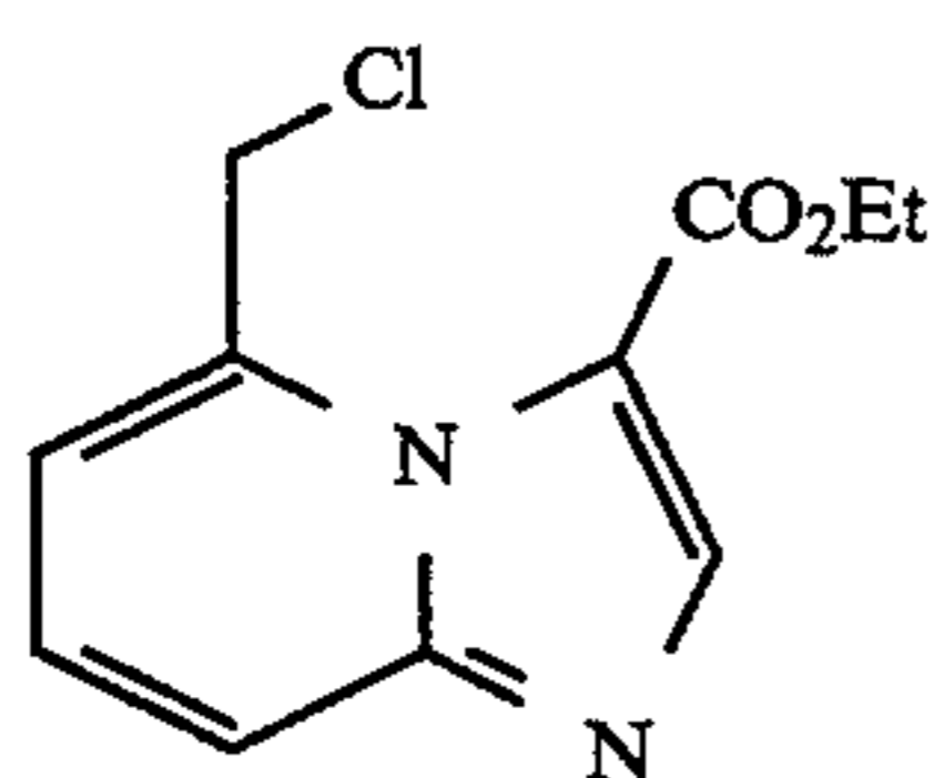
ethyl 5-(chloromethyl)imidazo[1,2-a]pyridine-3-carboxylate
