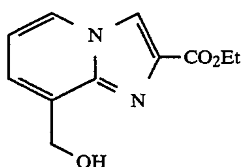
ethyl 8-(hydroxymethyl)imidazo[1,2-a]pyridine-2-carboxylate
