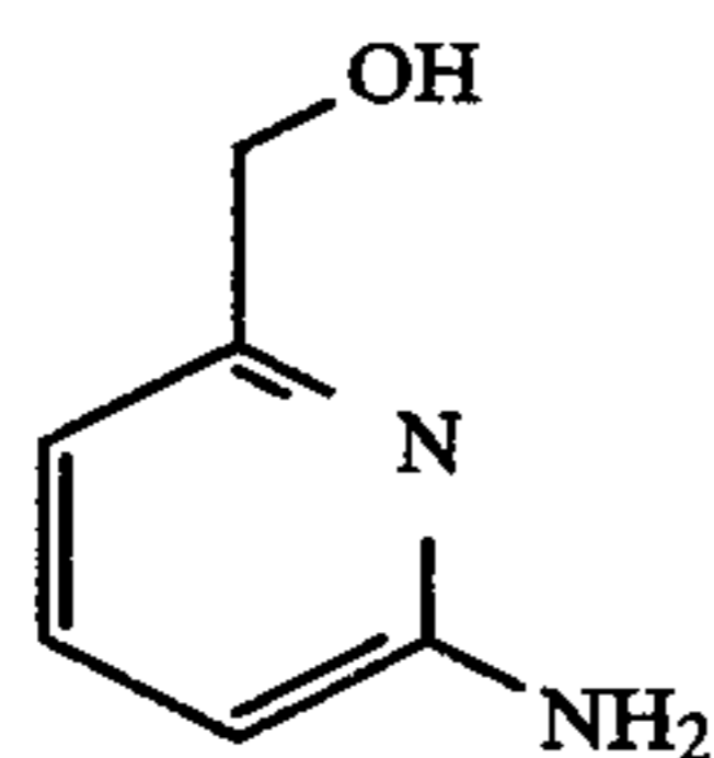
6-amino-2-pyridinemethanol
