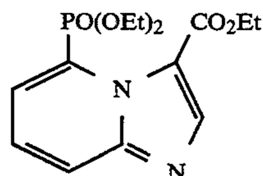
ethyl 5-(diethoxyphosphinyl)imidazo[1,2-a]pyridine-3-carboxylate
