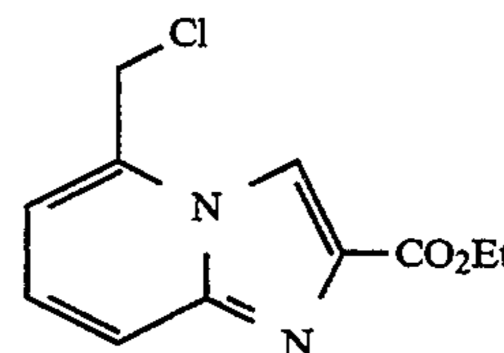
ethyl 5-(chloromethyl)imidazo[1,2-a]pyridine-2-carboxylate
