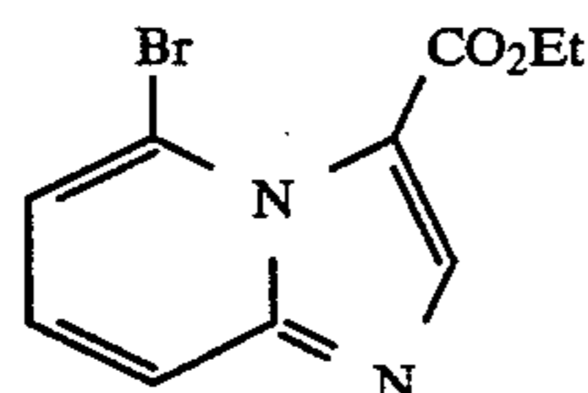
ethyl 5-bromoimidazo[1,2-a]pyridine-3-carboxylate
