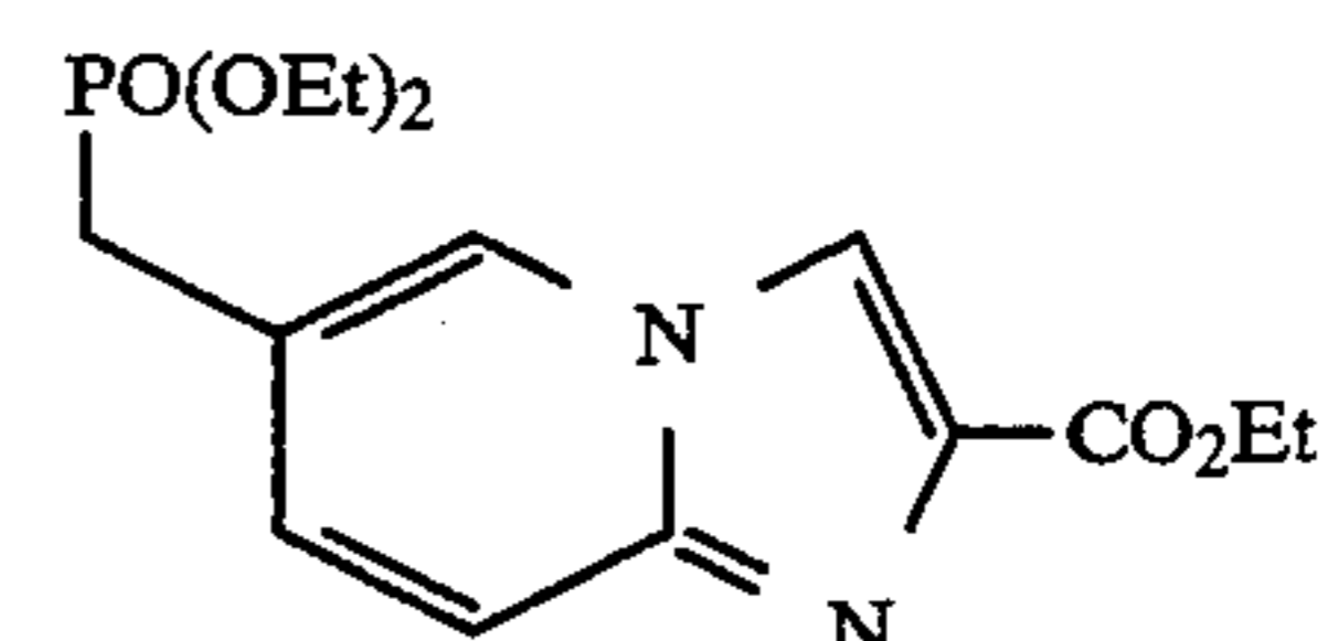
ethyl 6-[(diethoxyphosphinyl)methyl]imidazo[1,2-a]pyridine-2-carboxylate
