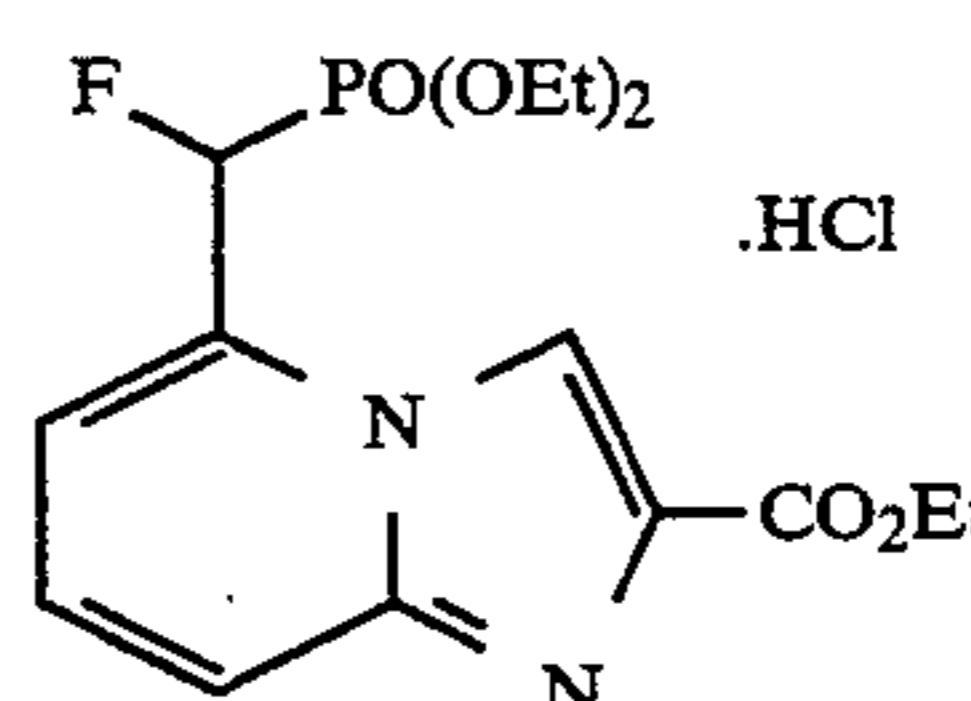
ethyl 5-[(diethoxyphosphinyl)fluoromethyl]imidazo [1,2-a]pyridine-2-carboxylate, monohydrochloride
