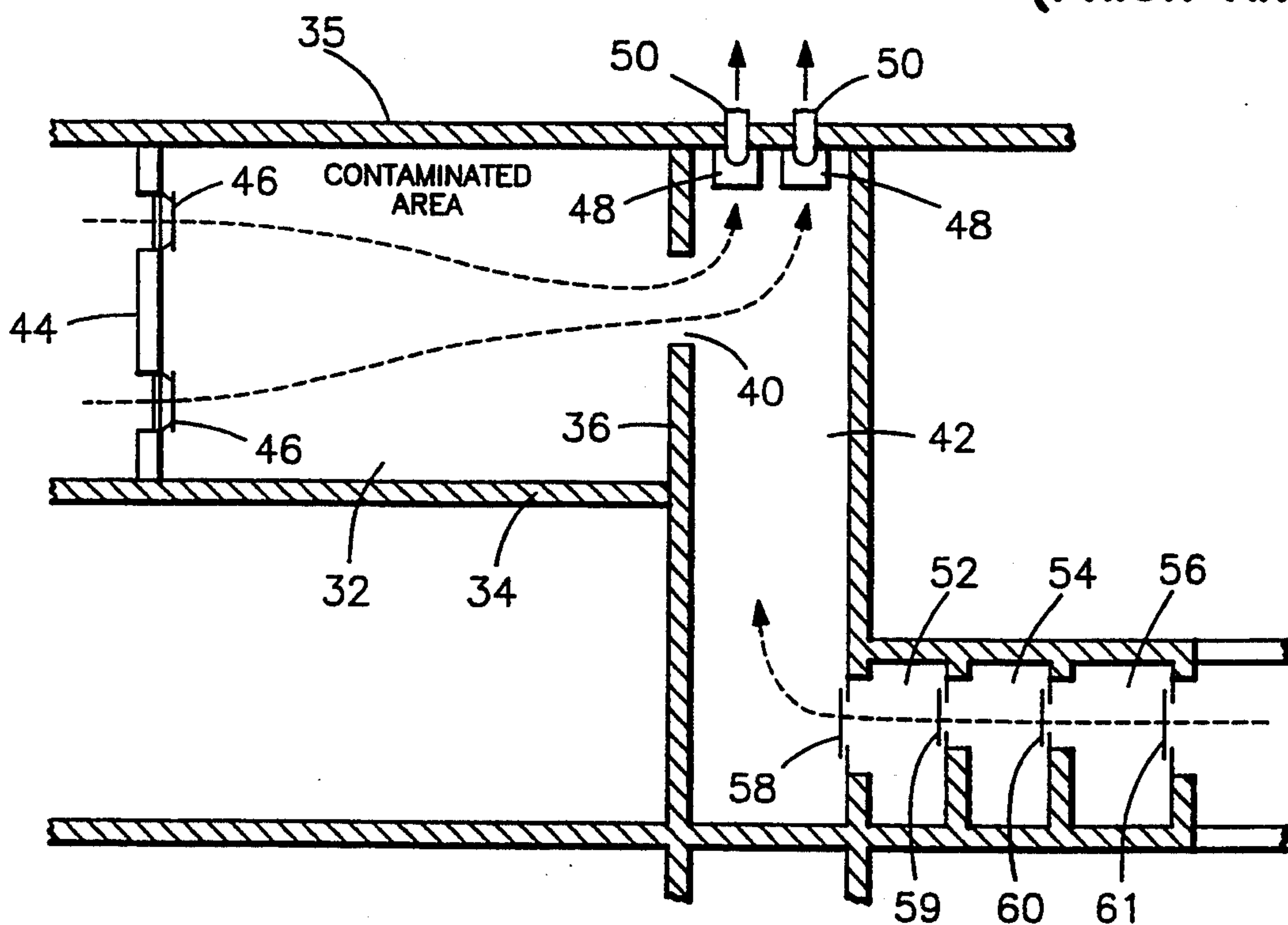
FIG. 2 (PRIOR ART)
