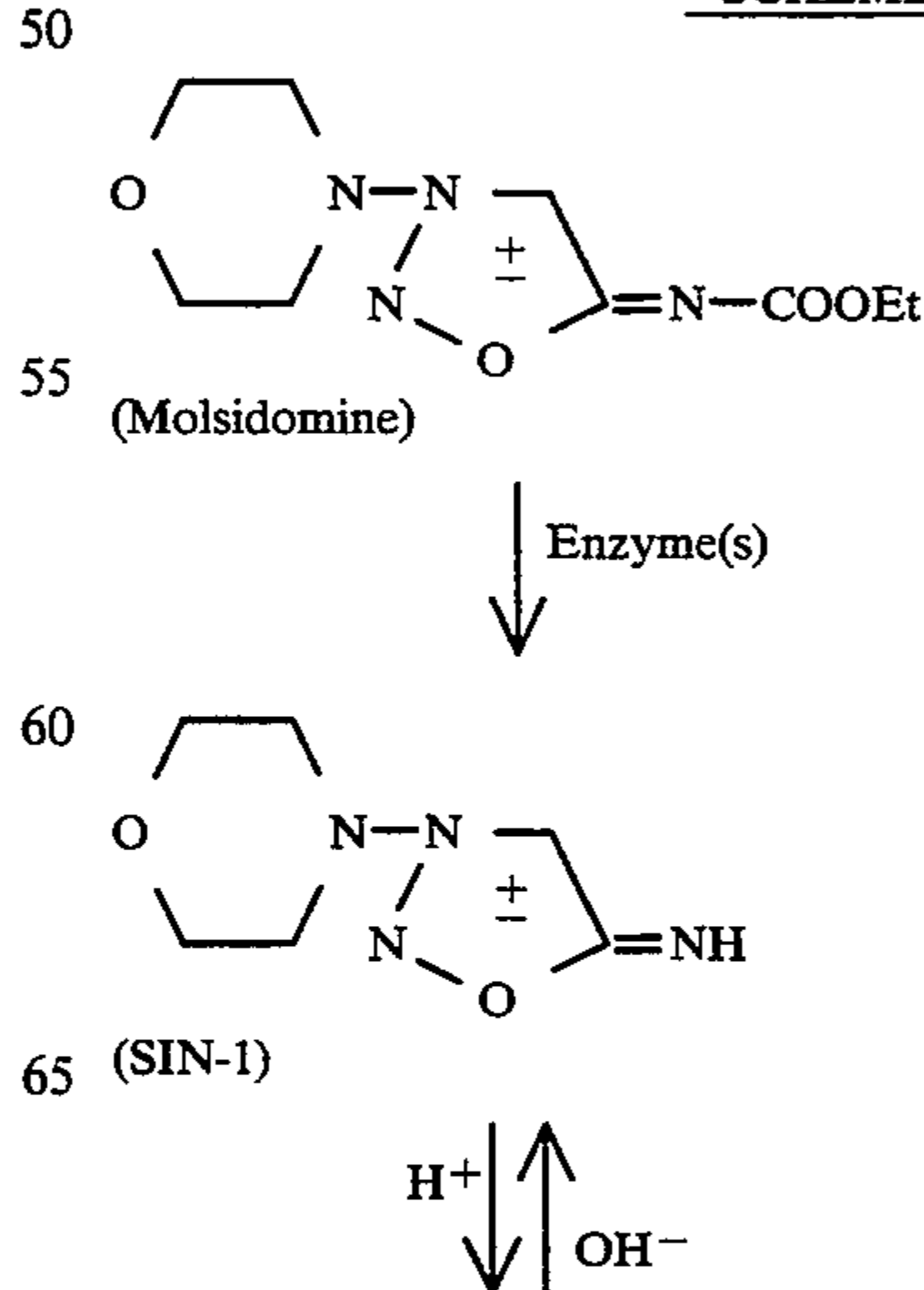
SCHEME 1
