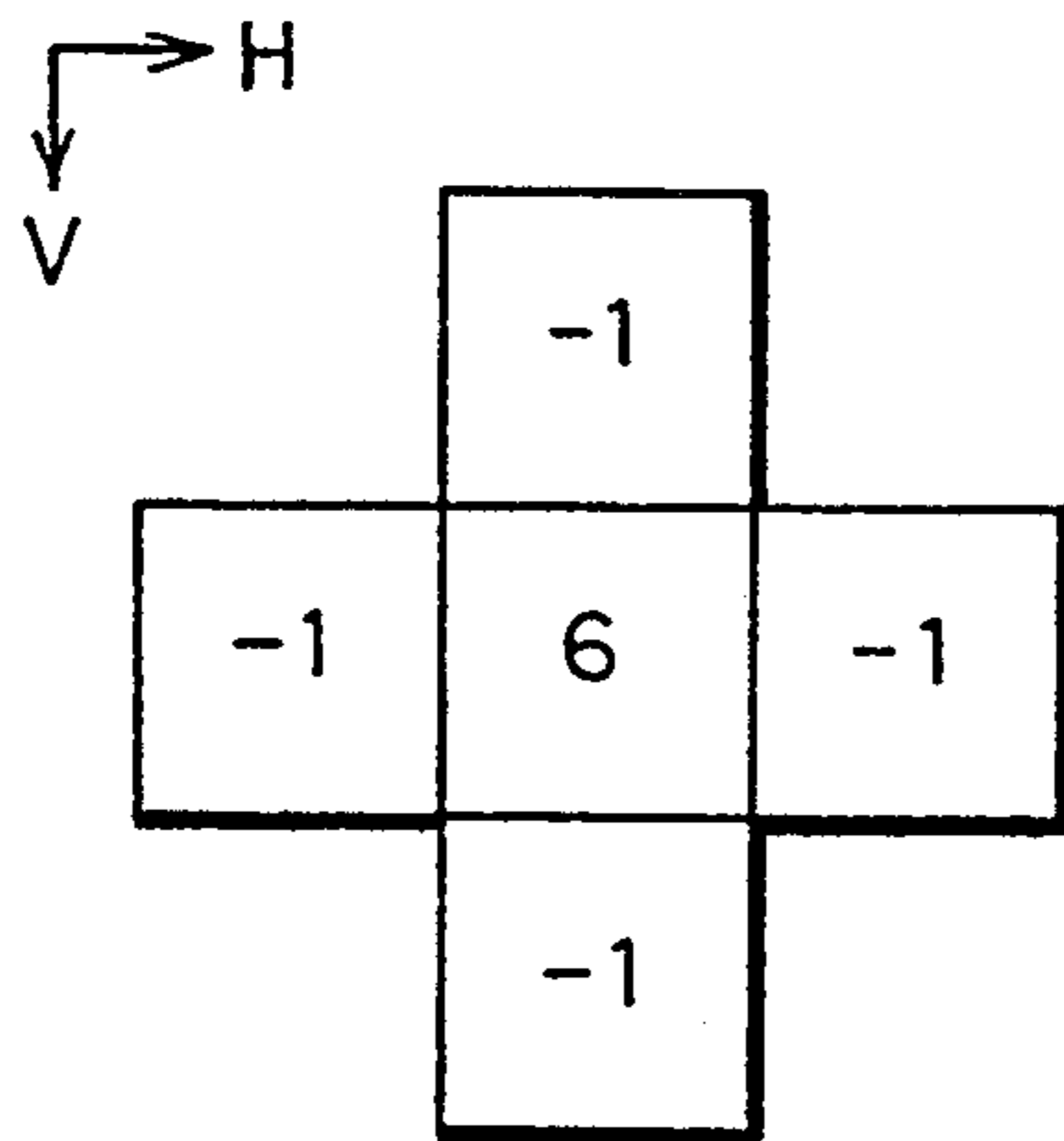
MTF CORRECTION
