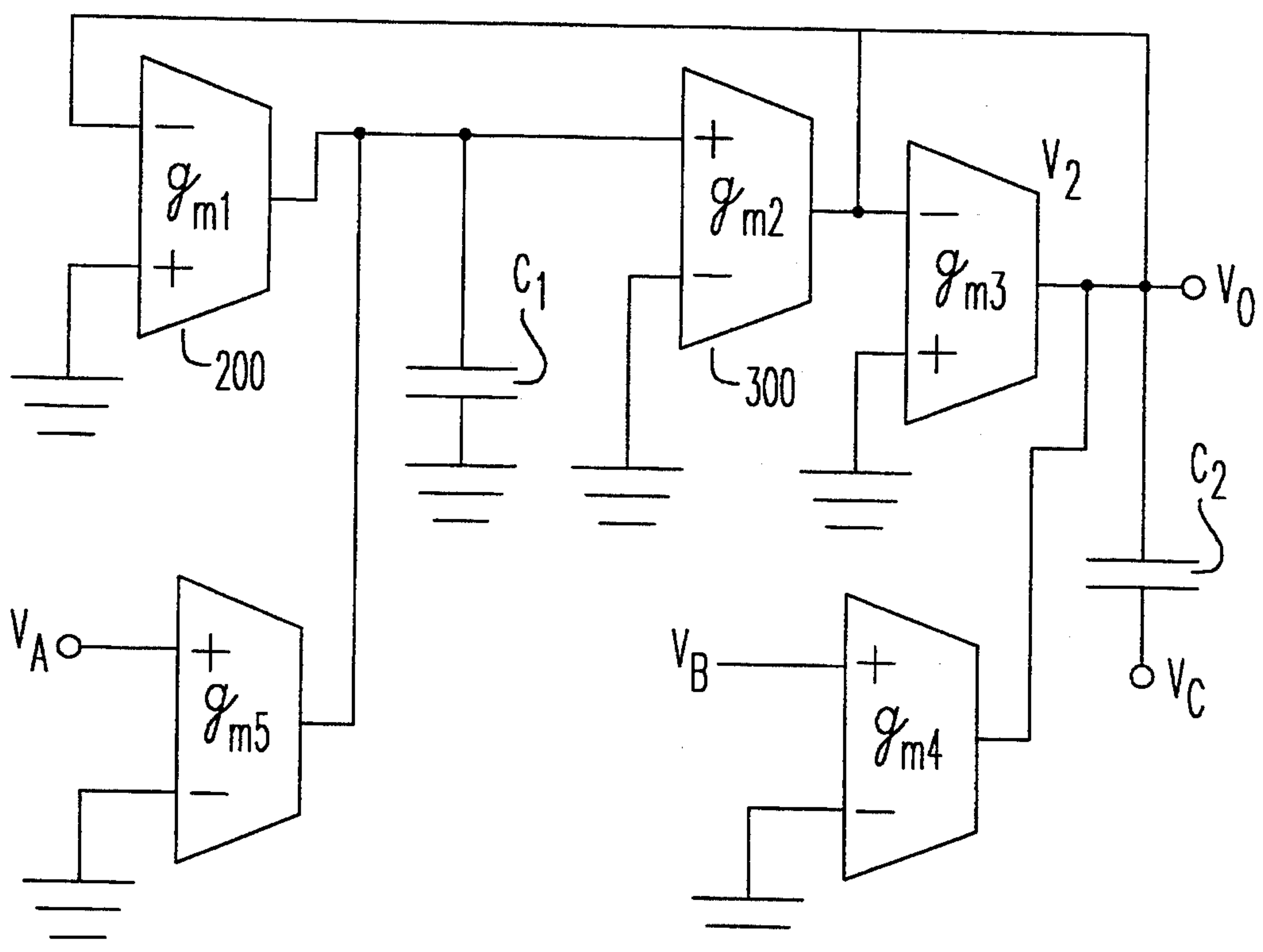
FIG. 3 (PRIOR ART)
